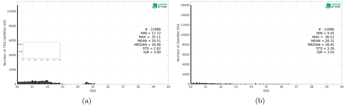
Figure 2: Histograms of SSS from TSG (SAMOS) (a) and SMOS SSS L3 Arctic v1.1 - 7-Day running mean (CATDS-CEC-LOCEAN) (b) considering all match-up pairs per bins of 0.1 over the Arctic Ocean Pi-MEP region and for the full satellite product period.
