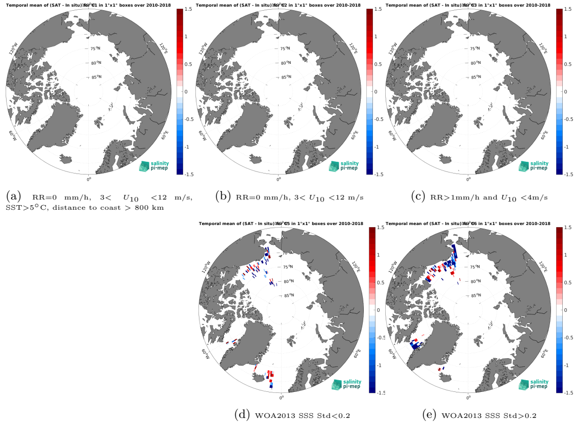
Figure 12: Temporal mean gridded over spatial boxes of size 1^{\circ}\times 1^{\circ} of \Delta\text{SSS} (SMOS SSS L3 Arctic v1.1 - 7-Day running mean (CATDS-CEC-LOCEAN) - TSG (SAMOS)) for 5 different subdatasets corresponding to:RR=0 mm/h, 3 < U_{10} < 12 m/s, SST > 5^{\circ}\text{C} , distance to coast > 800 km (a), RR=0 mm/h, 3 < U_{10} < 12 m/s (b), RR > 1 mm/h and U_{10} < 4 m/s (c), WOA2013 SSS Std < 0.2 (d), WOA2013 SSS Std > 0.2 (e).
