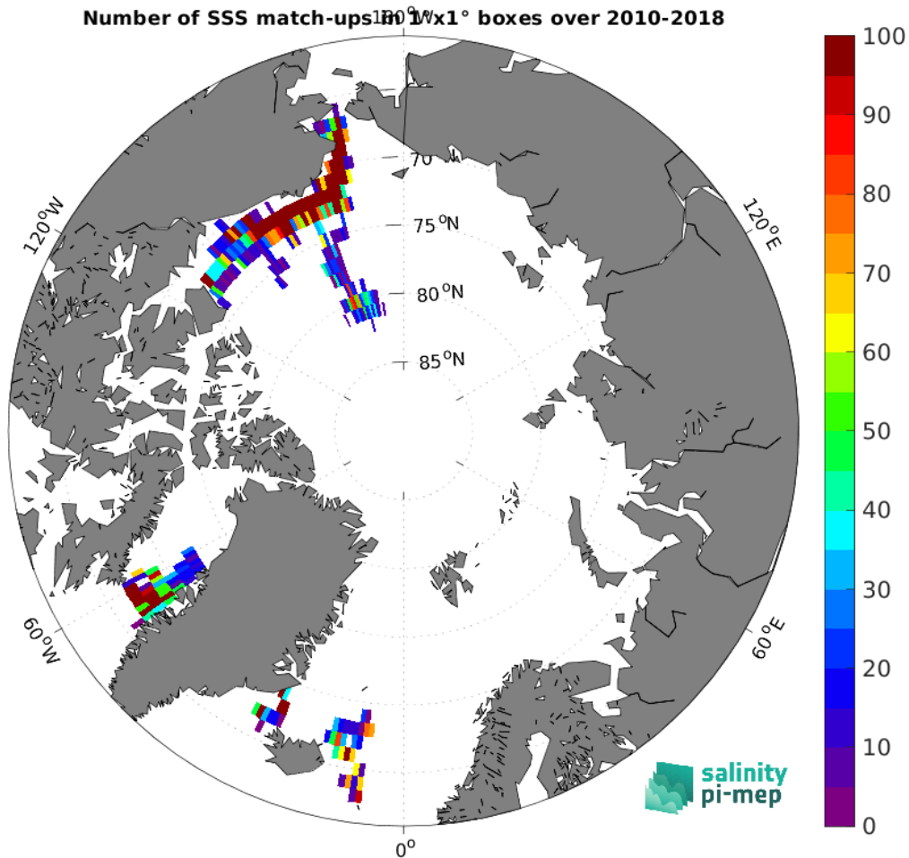
Figure 4: Number of SSS match-ups between TSG (SAMOS) SSS and the SMOS SSS L3 Arctic v1.1 - 7-Day running mean (CATDS-CEC-LOCEAN) SSS product for the Arctic Ocean Pi-MEP region over 1^\circ \times 1^\circ boxes and for the full satellite product period.
