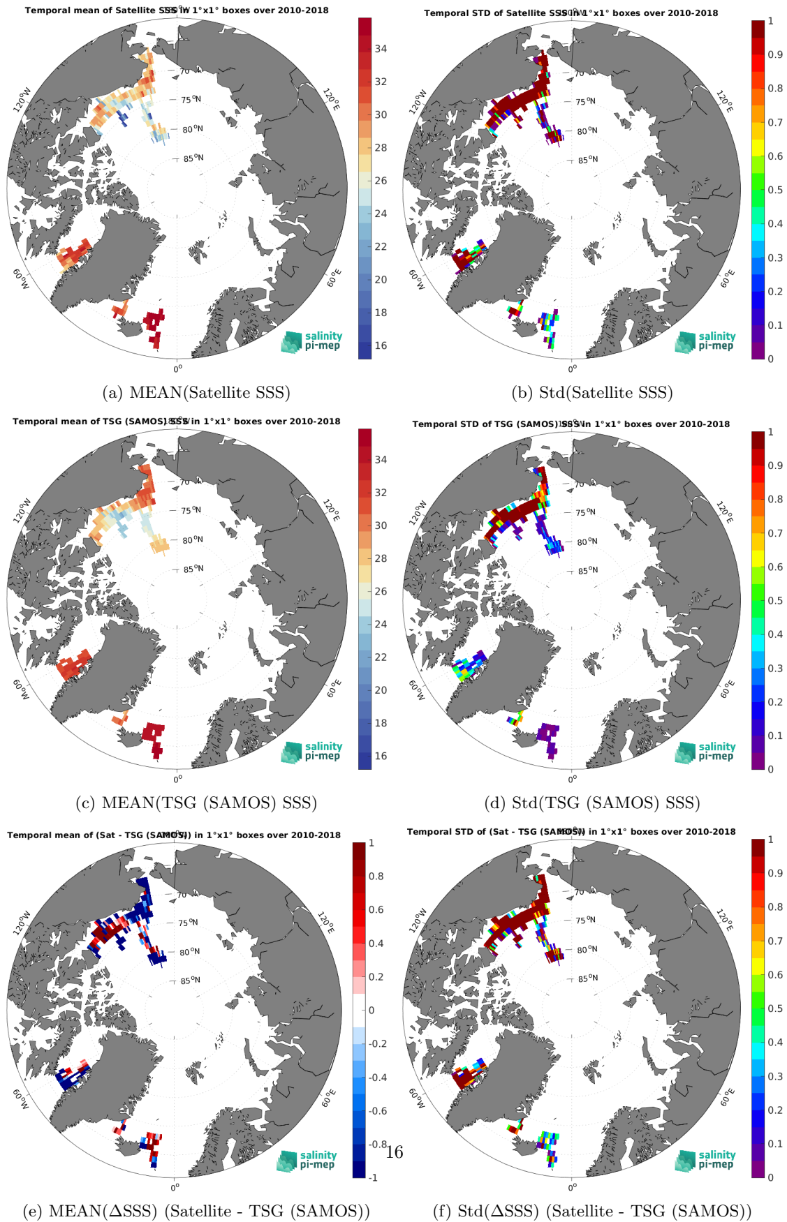
Figure 6: Temporal mean (left) and Std (right) of SSS from SMOS SSS L3 Arctic v1.1 - 7-Day running mean (CATDS-CEC-LOCEAN) (top), TSG (SAMOS) (middle), and of \Delta SSS (Satellite - TSG (SAMOS)). Only match-up pairs are used to generate these maps.
