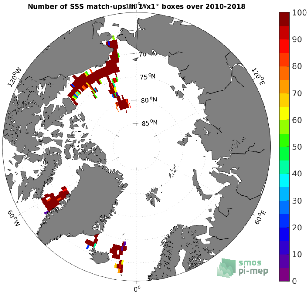
Figure 4: Number of SSS match-ups between TSG (SAMOS) SSS and the SMOS SSS L3 Arctic v1.1 - 7-Day running mean (CATDS-CECOS-LOCEAN) SSS product for the Arctic Ocean Pi-MEP region over 1^{\circ} \times 1^{\circ} boxes and for the full satellite product period.
