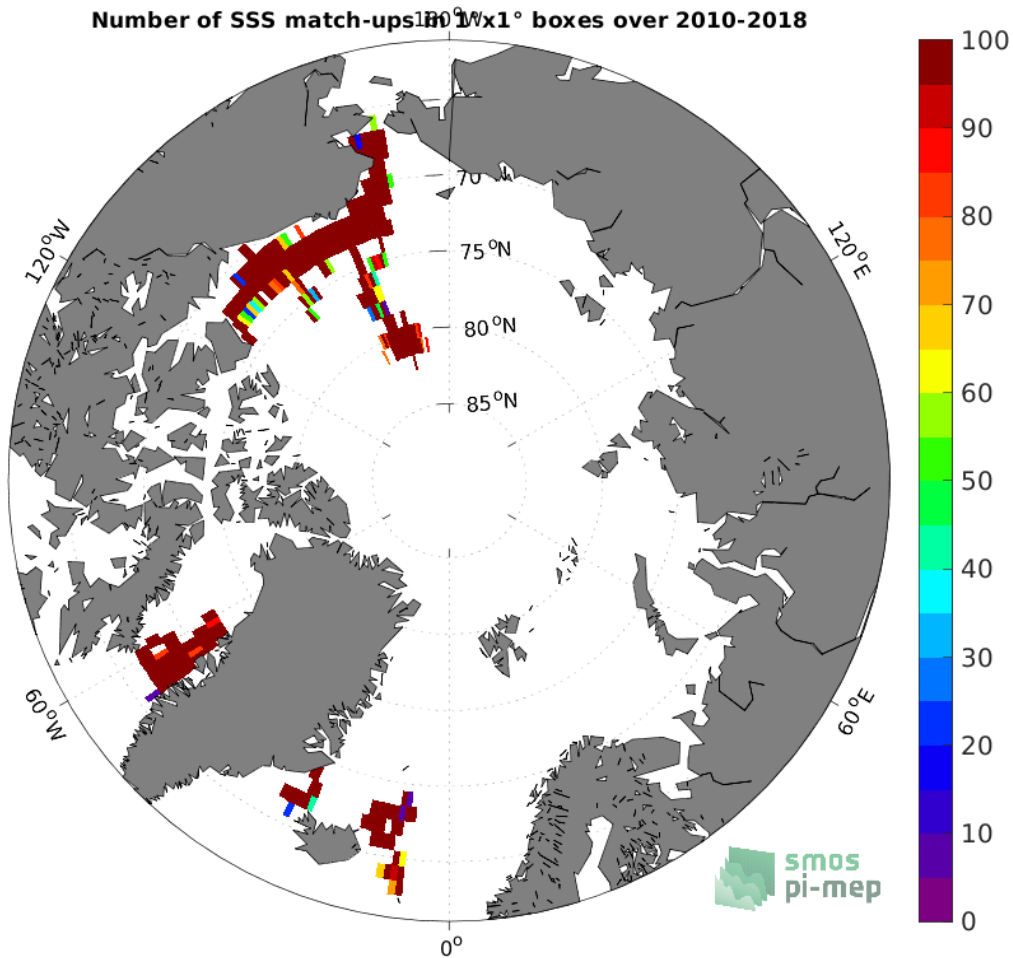
Figure 4: Number of SSS match-ups between TSG (SAMOS) SSS and the SMOS SSS L3 Arctic v1.1 - 7-Day running mean (CATDS-CECOS-LOCEAN) SSS product for the Arctic Ocean Pi-MEP region over 1^\circ \times 1^\circ boxes and for the full satellite product period.
