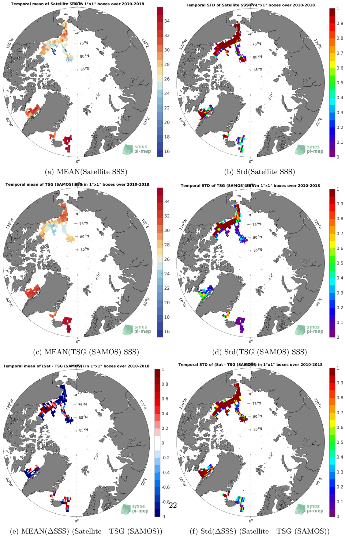
Figure 6: Temporal mean (left) and Std (right) of SSS from SMOS SSS L3 Arctic v1.1 - 7-Day running mean (CATDS-CECOS-LOCEAN) (top), TSG (SAMOS) (middle), and of \Delta SSS (Satellite - TSG (SAMOS)). Only match-up pairs are used to generate these maps.
