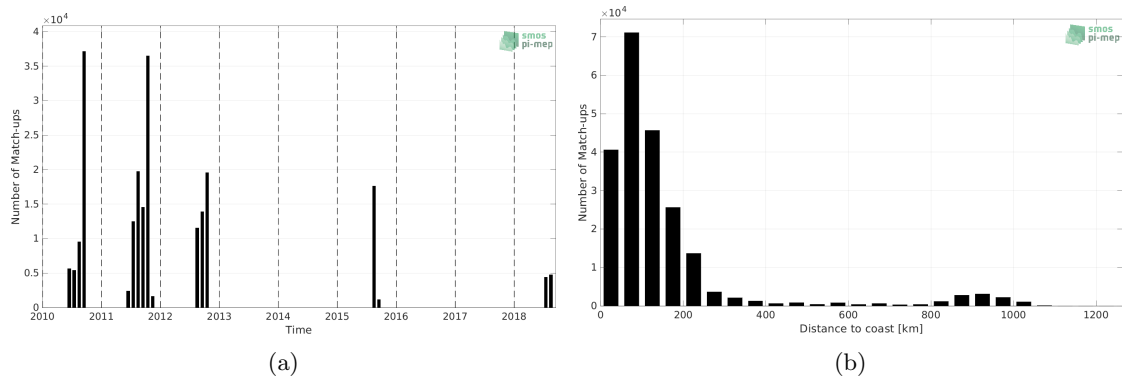
Figure 1: Number of match-ups between TSG (SAMOS) and SMOS SSS L3 Arctic v1.1 - 7-Day running mean (CATDS-CECOS-LOCEAN) SSS as a function of time (a) and as function of the distance to coast (b) over the Arctic Ocean Pi-MEP region and for the full satellite product period.
