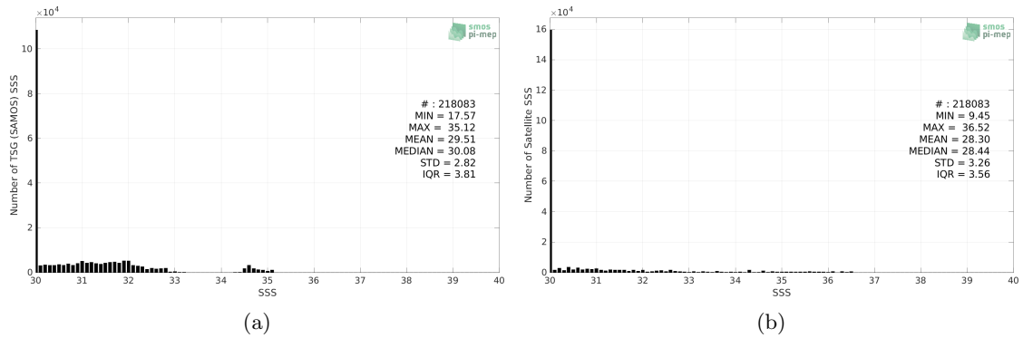
Figure 2: Histograms of SSS from TSG (SAMOS) (a) and SMOS SSS L3 Arctic v1.1 - 7-Day running mean (CATDS-CECOS-LOCEAN) (b) considering all match-up pairs per bins of 0.1 over the Arctic Ocean Pi-MEP region and for the full satellite product period.
