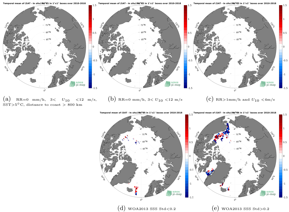
Figure 12: Temporal mean gridded over spatial boxes of size 1^{\circ}\times 1^{\circ} of \Delta\text{SSS} (SMOS SSS L3 Arctic v1.1 - 7-Day running mean (CATDS-CECOS-LOCEAN) - TSG (SAMOS)) for 5 different subdatasets corresponding to:RR=0 mm/h, 3 < U_{10} < 12 m/s, SST >5^{\circ}\text{C} , distance to coast > 800 km (a), RR=0 mm/h, 3 < U_{10} < 12 m/s (b), RR >1 mm/h and U_{10} < 4 m/s (c), WOA2013 SSS Std <0.2 (d), WOA2013 SSS Std >0.2 (e).
