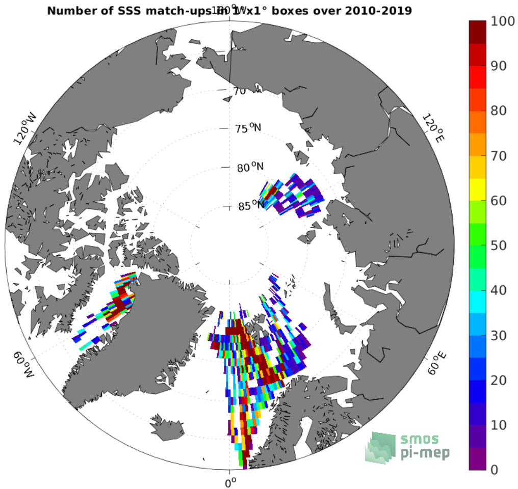
Figure 4: Number of SSS match-ups between TSG (Polarstern) SSS and the SMOS SSS L3 Arctic v1.1 - 7-Day running mean (CATDS-CECOS-LOCEAN) SSS product for the Arctic Ocean Pi-MEP region over 1^\circ \times 1^\circ boxes and for the full satellite product period.
