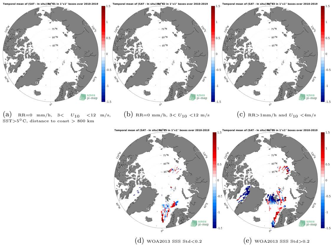
Figure 12: Temporal mean gridded over spatial boxes of size 1^{\circ}\times 1^{\circ} of \Delta\text{SSS} (SMOS SSS L3 Arctic v1.1 - 7-Day running mean (CATDS-CECOS-LOCEAN) - TSG (Polarstern)) for 5 different subdatasets corresponding to:RR=0 mm/h, 3 < U_{10} < 12 m/s, SST >5^{\circ}\text{C} , distance to coast > 800 km (a), RR=0 mm/h, 3 < U_{10} < 12 m/s (b), RR >1 mm/h and U_{10} < 4 m/s (c), WOA2013 SSS Std <0.2 (d), WOA2013 SSS Std >0.2 (e).
