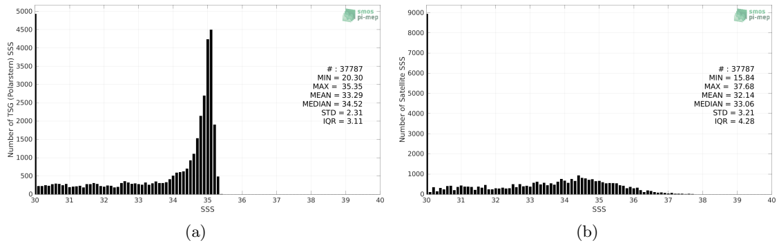
Figure 2: Histograms of SSS from TSG (Polarstern) (a) and SMOS SSS L3 Arctic v1.1 - 7-Day running mean (CATDS-CECOS-LOCEAN) (b) considering all match-up pairs per bins of 0.1 over the Arctic Ocean Pi-MEP region and for the full satellite product period.
