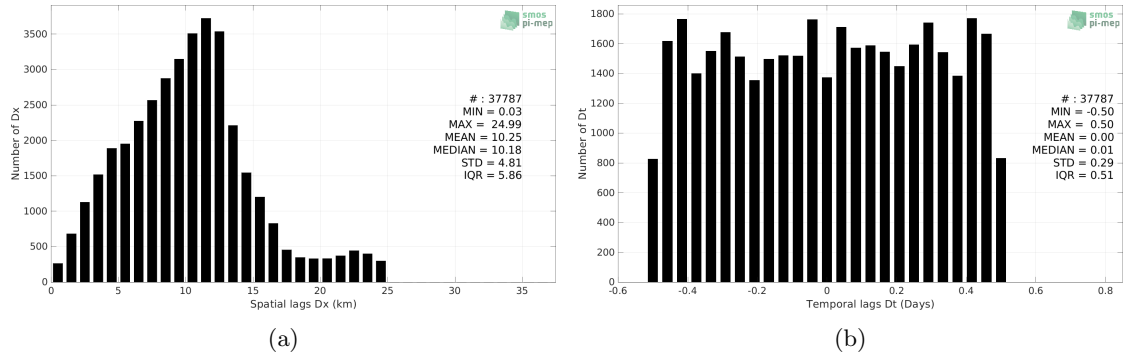
Figure 5: Histograms of the spatial (a) and temporal (b) lags between the location/time of the TSG (Polarstern) measurement and the corresponding SMOS SSS L3 Arctic v1.1 - 7-Day running mean (CATDS-CECOS-LOCEAN) SSS pixel.
