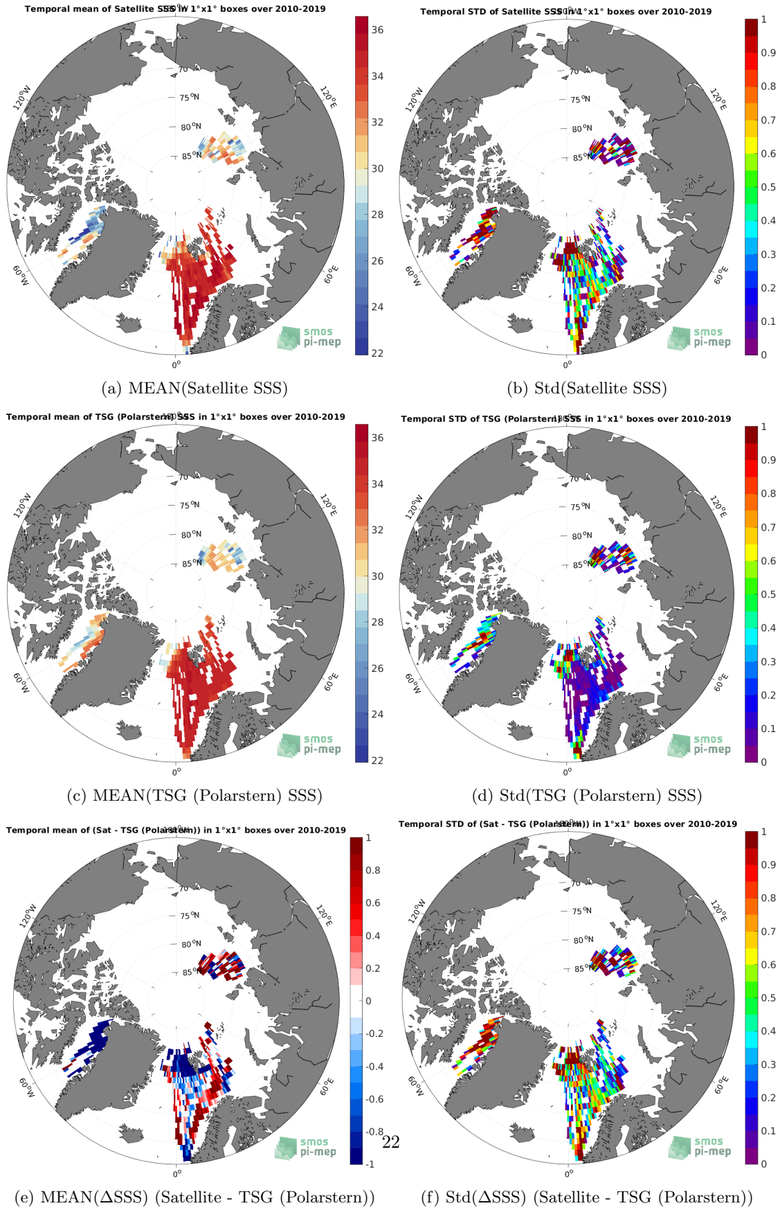
Figure 6: Temporal mean (left) and Std (right) of SSS from SMOS SSS L3 Arctic v1.1 - 7-Day running mean (CATDS-CECOS-LOCEAN) (top), TSG (Polarstern) (middle), and of \Delta SSS (Satellite - TSG (Polarstern)). Only match-up pairs are used to generate these maps.
