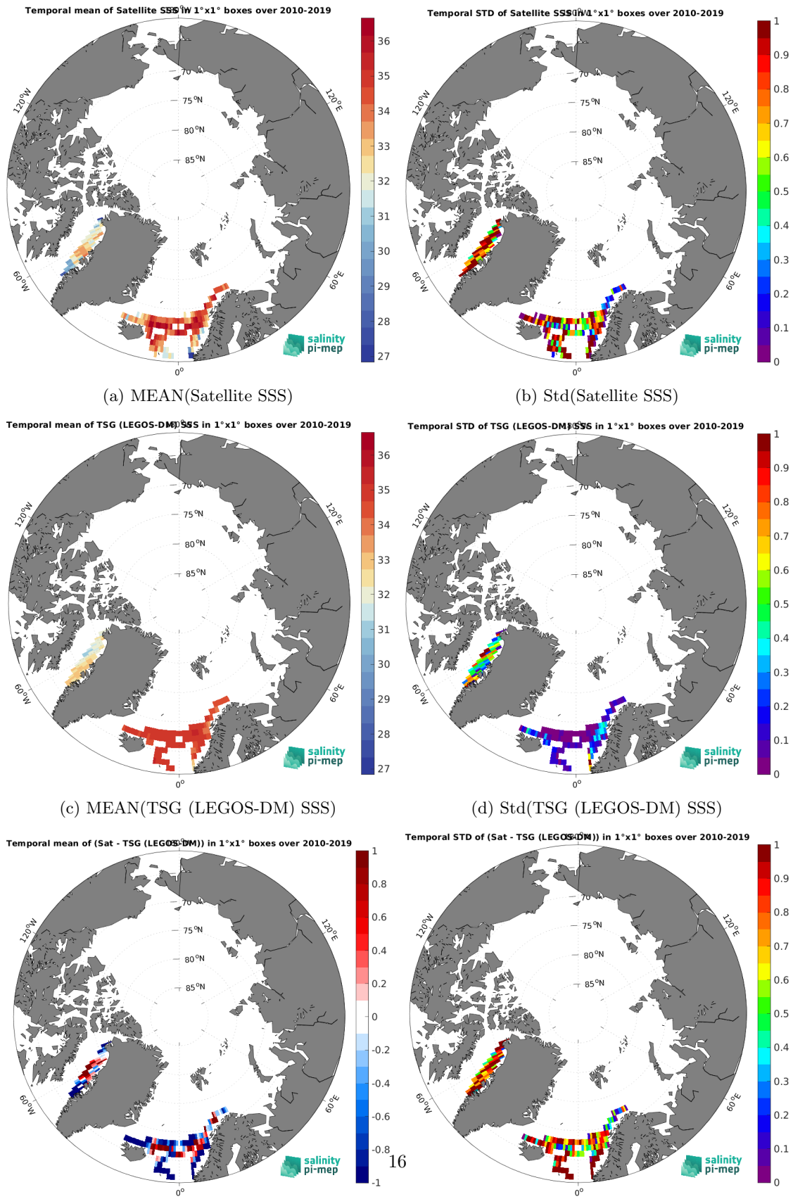
Figure 6: Temporal mean (left) and Std (right) of SSS from SMOS SSS L3 Arctic v1.1 - 7-Day running mean (CATDS-CEC-LOCEAN) (top), TSG (LEGOS-DM) (middle), and of \Delta SSS (Satellite - TSG (LEGOS-DM)). Only match-up pairs are used to generate these maps.
