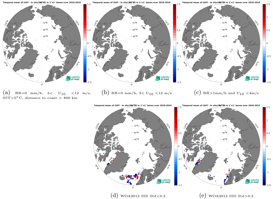
Figure 12: Temporal mean gridded over spatial boxes of size 1^{\circ}\times 1^{\circ} of \Delta\text{SSS} (SMOS SSS L3 Arctic v1.1 - 7-Day running mean (CATDS-CEC-LOCEAN) - TSG (LEGOS-DM)) for 5 different subdatasets corresponding to:RR=0 mm/h, 3 < U_{10} < 12 m/s, SST > 5^{\circ}\text{C} , distance to coast > 800 km (a), RR=0 mm/h, 3 < U_{10} < 12 m/s (b), RR > 1 mm/h and U_{10} < 4 m/s (c), WOA2013 SSS Std < 0.2 (d), WOA2013 SSS Std > 0.2 (e).
