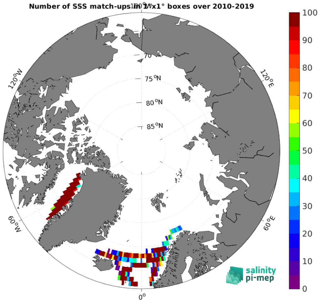
Figure 4: Number of SSS match-ups between TSG (LEGOS-DM) SSS and the SMOS SSS L3 Arctic v1.1 - 7-Day running mean (CATDS-CEC-LOCEAN) SSS product for the Arctic Ocean Pi-MEP region over 1^\circ \times 1^\circ boxes and for the full satellite product period.
