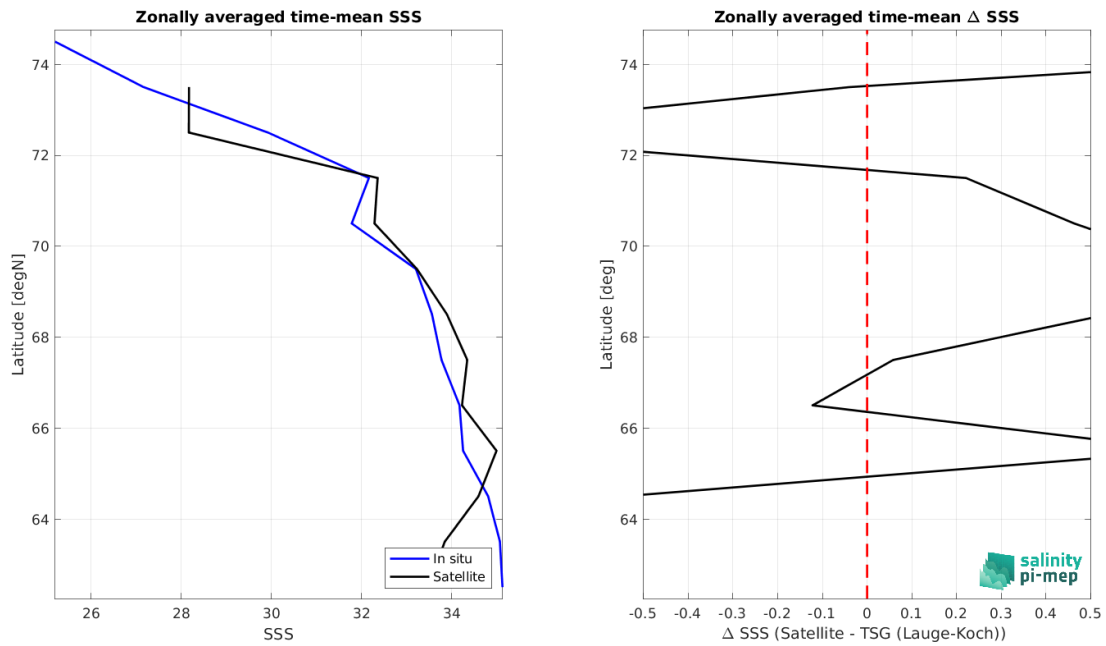
Figure 8: Left panel: Zonal mean SSS from SMOS SSS L3 Arctic v1.1 - 7-Day running mean (CATDS-CEC-LOCEAN) satellite product (black) and from TSG (Lauge-Koch) (blue). Right panel: Zonal mean of \Delta SSS (Satellite - TSG (Lauge-Koch)) for all the collected Pi-MEP match-up pairs estimated over the full satellite product period.
