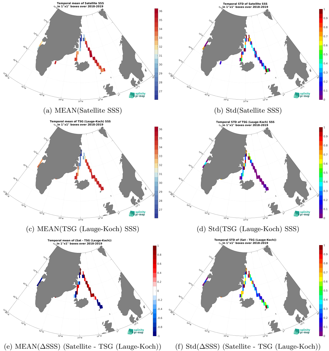
Figure 6: Temporal mean (left) and Std (right) of SSS from SMOS SSS L3 Arctic v1.1 - 7-Day running mean (CATDS-CEC-LOCEAN) (top), TSG (Lauge-Koch) (middle), and of \Delta SSS (Satellite - TSG (Lauge-Koch)). Only match-up pairs are used to generate these maps.
