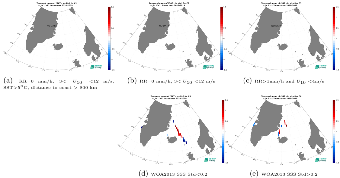
Figure 12: Temporal mean gridded over spatial boxes of size 1^{\circ}\times 1^{\circ} of \Delta\text{SSS} (SMOS SSS L3 Arctic v1.1 - 7-Day running mean (CATDS-CEC-LOCEAN) - TSG (Lauge-Koch)) for 5 different subdatasets corresponding to:RR=0 mm/h, 3 < U_{10} < 12 m/s, SST >5^{\circ}\text{C} , distance to coast > 800 km (a), RR=0 mm/h, 3 < U_{10} < 12 m/s (b), RR >1 mm/h and U_{10} < 4 m/s (c), WOA2013 SSS Std <0.2 (d), WOA2013 SSS Std >0.2 (e).
