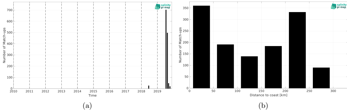
Figure 1: Number of match-ups between TSG (Lauge-Koch) and SMOS SSS L3 Arctic v1.1 - 7-Day running mean (CATDS-CEC-LOCEAN) SSS as a function of time (a) and as function of the distance to coast (b) over the Arctic Ocean Pi-MEP region and for the full satellite product period.
