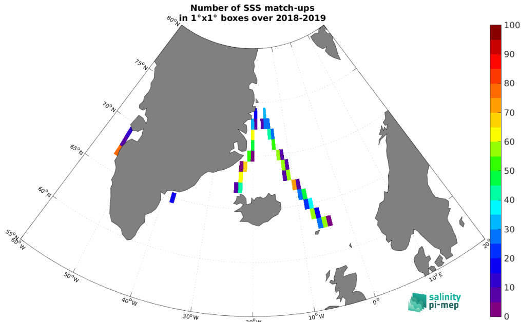
Figure 4: Number of SSS match-ups between TSG (Lauge-Koch) SSS and the SMOS SSS L3 Arctic v1.1 - 7-Day running mean (CATDS-CEC-LOCEAN) SSS product for the Arctic Ocean Pi-MEP region over 1^\circ \times 1^\circ boxes and for the full satellite product period.
