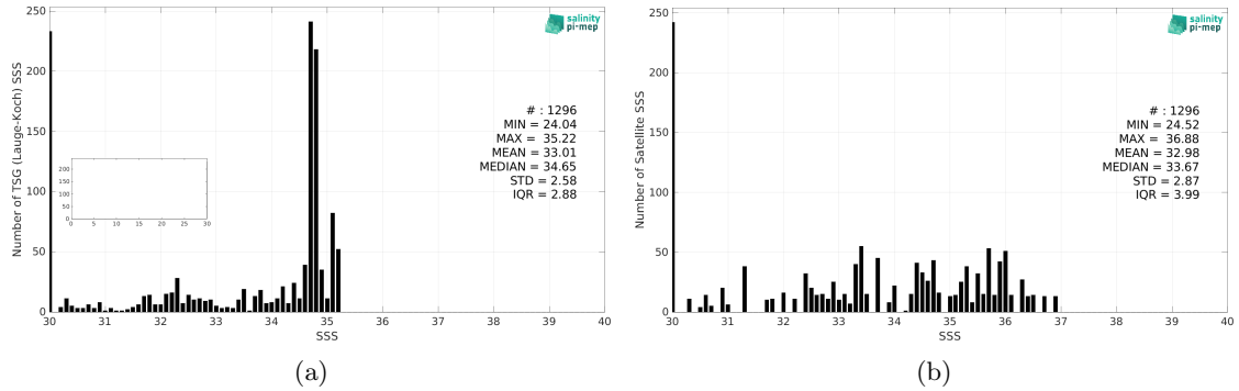
Figure 2: Histograms of SSS from TSG (Lauge-Koch) (a) and SMOS SSS L3 Arctic v1.1 - 7-Day running mean (CATDS-CEC-LOCEAN) (b) considering all match-up pairs per bins of 0.1 over the Arctic Ocean Pi-MEP region and for the full satellite product period.
