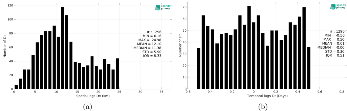
Figure 5: Histograms of the spatial (a) and temporal (b) lags between the location/time of the TSG (Lauge-Koch) measurement and the date of the corresponding SMOS SSS L3 Arctic v1.1 - 7-Day running mean (CATDS-CEC-LOCEAN) SSS pixel.
