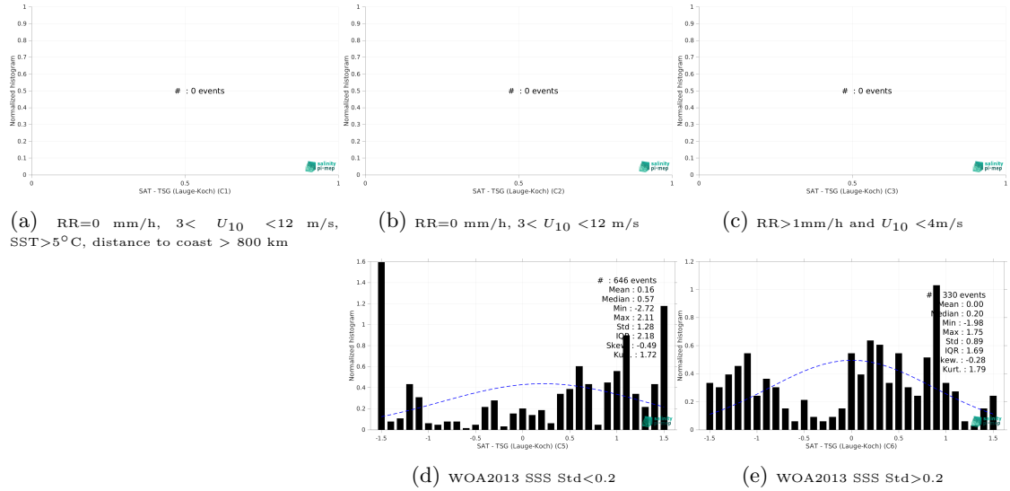
Figure 13: Normalized histogram of \Delta SSS (SMOS SSS L3 Arctic v1.1 - 7-Day runing mean (CATDS-CEC-LOCEAN) - TSG (Lauge-Koch)) for 5 different subdatasets corresponding to: RR=0 mm/h, 3 < U_{10} < 12 m/s, SST>5°C, distance to coast > 800 km (a), RR=0 mm/h, 3 < U_{10} < 12 m/s (b), RR>1mm/h and U_{10} < 4 m/s (c), WOA2013 SSS Std<0.2 (d), WOA2013 SSS Std>0.2 (e).
