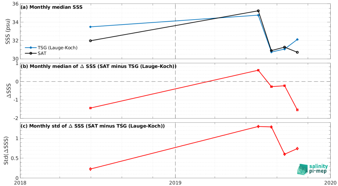
Figure 7: Time series of the monthly median SSS (top), median of \Delta\text{SSS} (Satellite - TSG (Lauge-Koch)) and Std of \Delta\text{SSS} (Satellite - TSG (Lauge-Koch)) over the Arctic Ocean Pi-MEP region considering all match-ups collected by the Pi-MEP.
