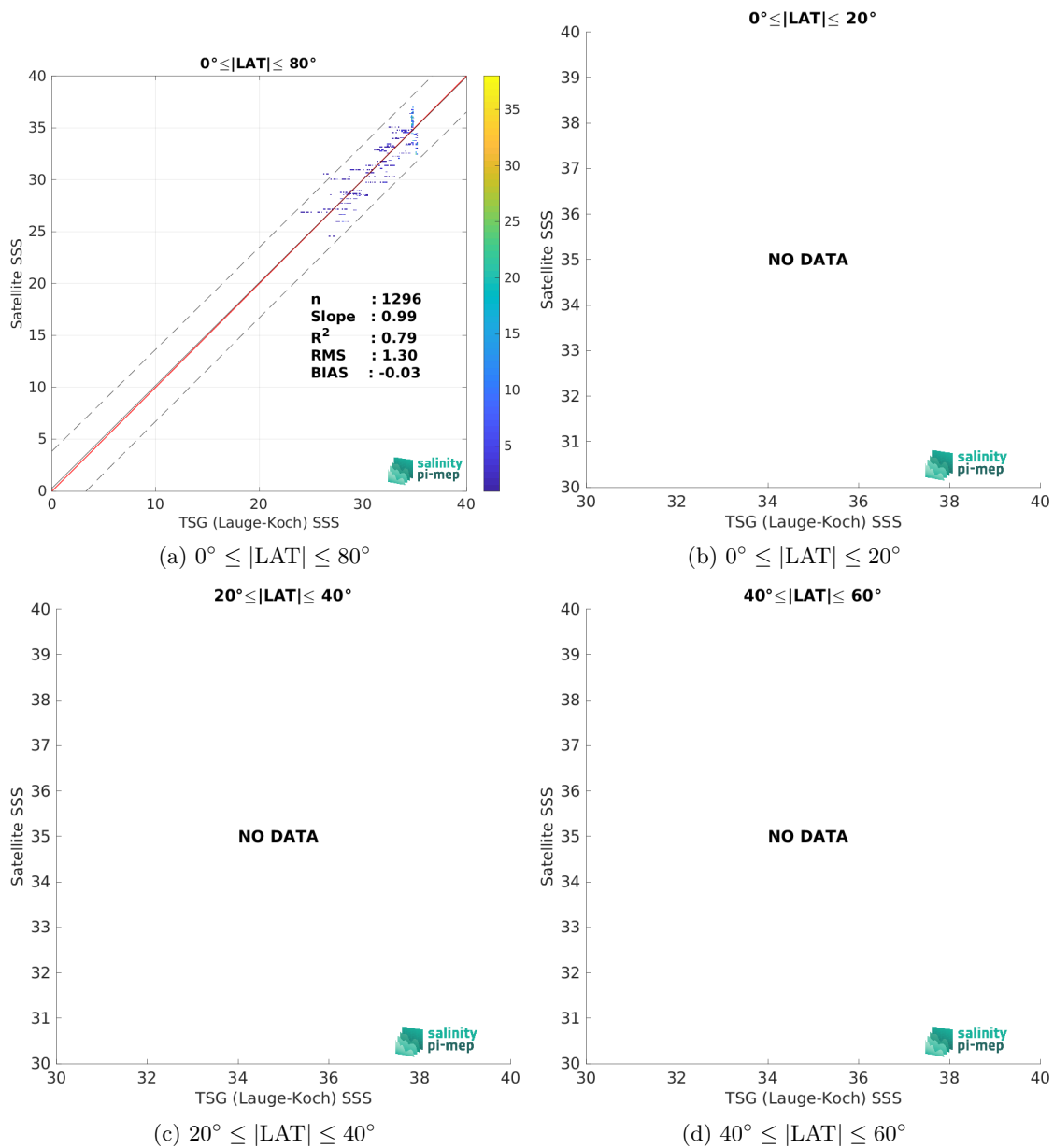
Figure 9: Contour maps of the concentration of SMOS SSS L3 Arctic v1.1 - 7-Day running mean (CATDS-CEC-LOCEAN) SSS (y-axis) versus TSG (Lauge-Koch) SSS (x-axis) at match-up pairs for different latitude bands. For each plot, the red line shows x=y . The black thin and dashed lines indicate a linear fit through the data cloud and the \pm 95\% confidence levels, respectively. The number match-up pairs n , the slope and R^2 coefficient of the linear fit, the root mean square (RMS) and the mean bias between satellite and in situ data are indicated for each latitude band in each plots.
