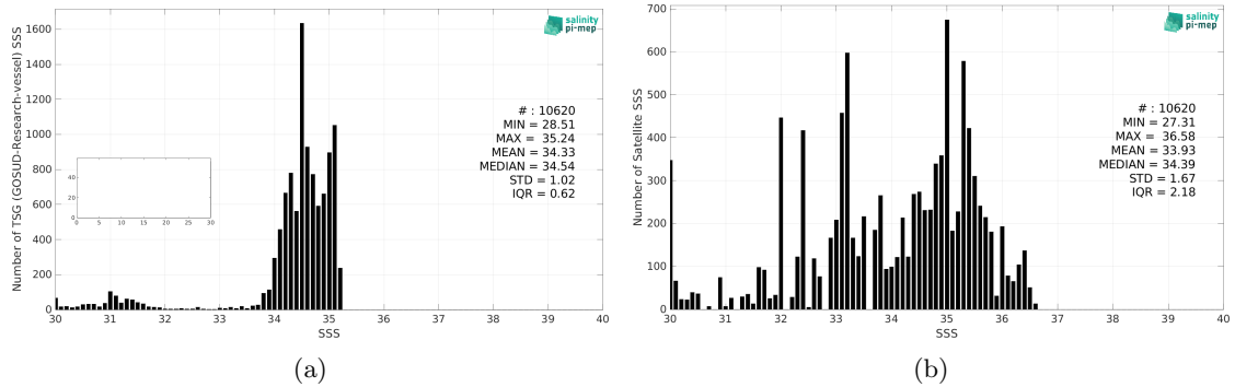
Figure 2: Histograms of SSS from TSG (GOSUD-Research-vessel) (a) and SMOS SSS L3 Arctic v1.1 - 7-Day running mean (CATDS-CEC-LOCEAN) (b) considering all match-up pairs per bins of 0.1 over the Arctic Ocean Pi-MEP region and for the full satellite product period.
