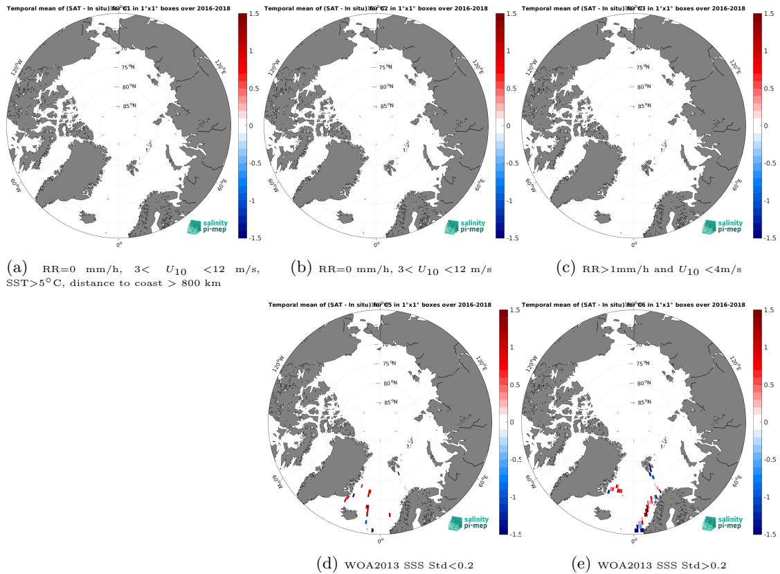
Figure 12: Temporal mean gridded over spatial boxes of size 1^\circ \times 1^\circ of \Delta SSS (SMOS SSS L3 Arctic v1.1 - 7-Day running mean (CATDS-CEC-LOCEAN) - TSG (GOSUD-Research-vessel)) for 5 different subdatasets corresponding to: RR=0 mm/h, 3 < U_{10} < 12 m/s, SST > 5°C, distance to coast > 800 km (a), RR=0 mm/h, 3 < U_{10} < 12 m/s (b), RR > 1mm/h and U_{10} < 4 m/s (c), WOA2013 SSS Std < 0.2 (d), WOA2013 SSS Std > 0.2 (e).
