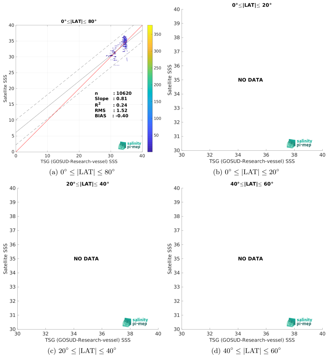
Figure 9: Contour maps of the concentration of SMOS SSS L3 Arctic v1.1 - 7-Day running mean (CATDS-CEC-LOCEAN) SSS (y-axis) versus TSG (GOSUD-Research-vessel) SSS (x-axis) at match-up pairs for different latitude bands. For each plot, the red line shows x=y . The black thin and dashed lines indicate a linear fit through the data cloud and the \pm 95\% confidence levels, respectively. The number match-up pairs n , the slope and R^2 coefficient of the linear fit, the root mean square (RMS) and the mean bias between satellite and in situ data are indicated for each latitude band in each plots.
