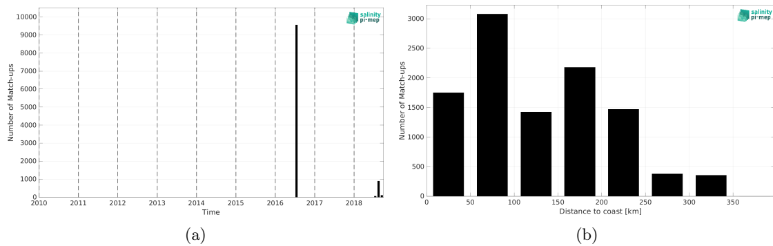
Figure 1: Number of match-ups between TSG (GOSUD-Research-vessel) and SMOS SSS L3 Arctic v1.1 - 7-Day running mean (CATDS-CEC-LOCEAN) SSS as a function of time (a) and as function of the distance to coast (b) over the Arctic Ocean Pi-MEP region and for the full satellite product period.
