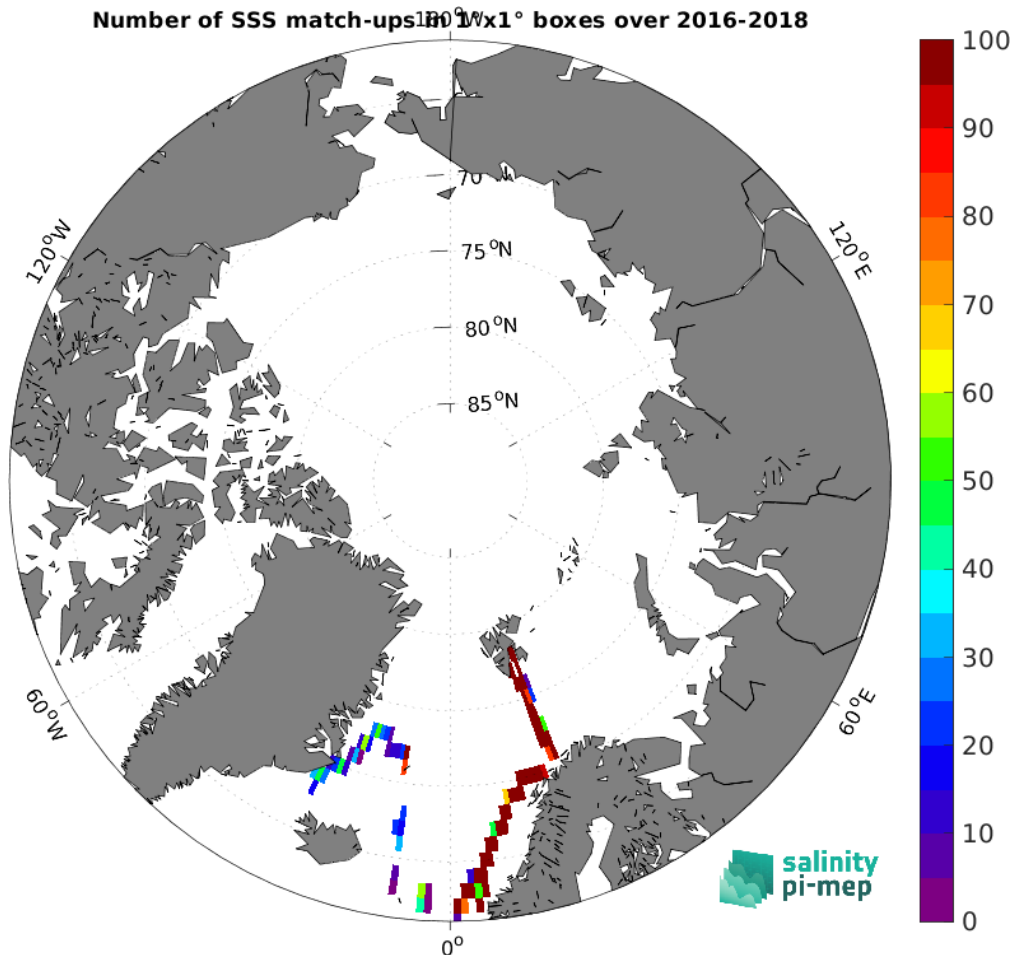
Figure 4: Number of SSS match-ups between TSG (GOSUD-Research-vessel) SSS and the SMOS SSS L3 Arctic v1.1 - 7-Day running mean (CATDS-CEC-LOCEAN) SSS product for the Arctic Ocean Pi-MEP region over 1^\circ \times 1^\circ boxes and for the full satellite product period.
