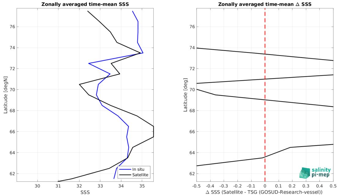
Figure 8: Left panel: Zonal mean SSS from SMOS SSS L3 Arctic v1.1 - 7-Day running mean (CATDS-CEC-LOCEAN) satellite product (black) and from TSG (GOSUD-Research-vessel) (blue). Right panel: Zonal mean of \Delta SSS (Satellite - TSG (GOSUD-Research-vessel)) for all the collected Pi-MEP match-up pairs estimated over the full satellite product period.
