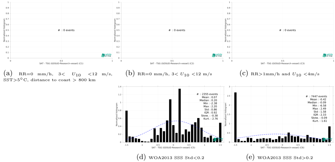
Figure 13: Normalized histogram of \Delta SSS (SMOS SSS L3 Arctic v1.1 - 7-Day runing mean (CATDS-CEC-LOCEAN) - TSG (GOSUD-Research-vessel)) for 5 different subdatasets corresponding to: RR=0 mm/h, 3 < U_{10} < 12 m/s, SST>5°C, distance to coast > 800 km (a), RR=0 mm/h, 3 < U_{10} < 12 m/s (b), RR>1mm/h and U_{10} < 4 m/s (c), WOA2013 SSS Std<0.2 (d), WOA2013 SSS Std>0.2 (e).
