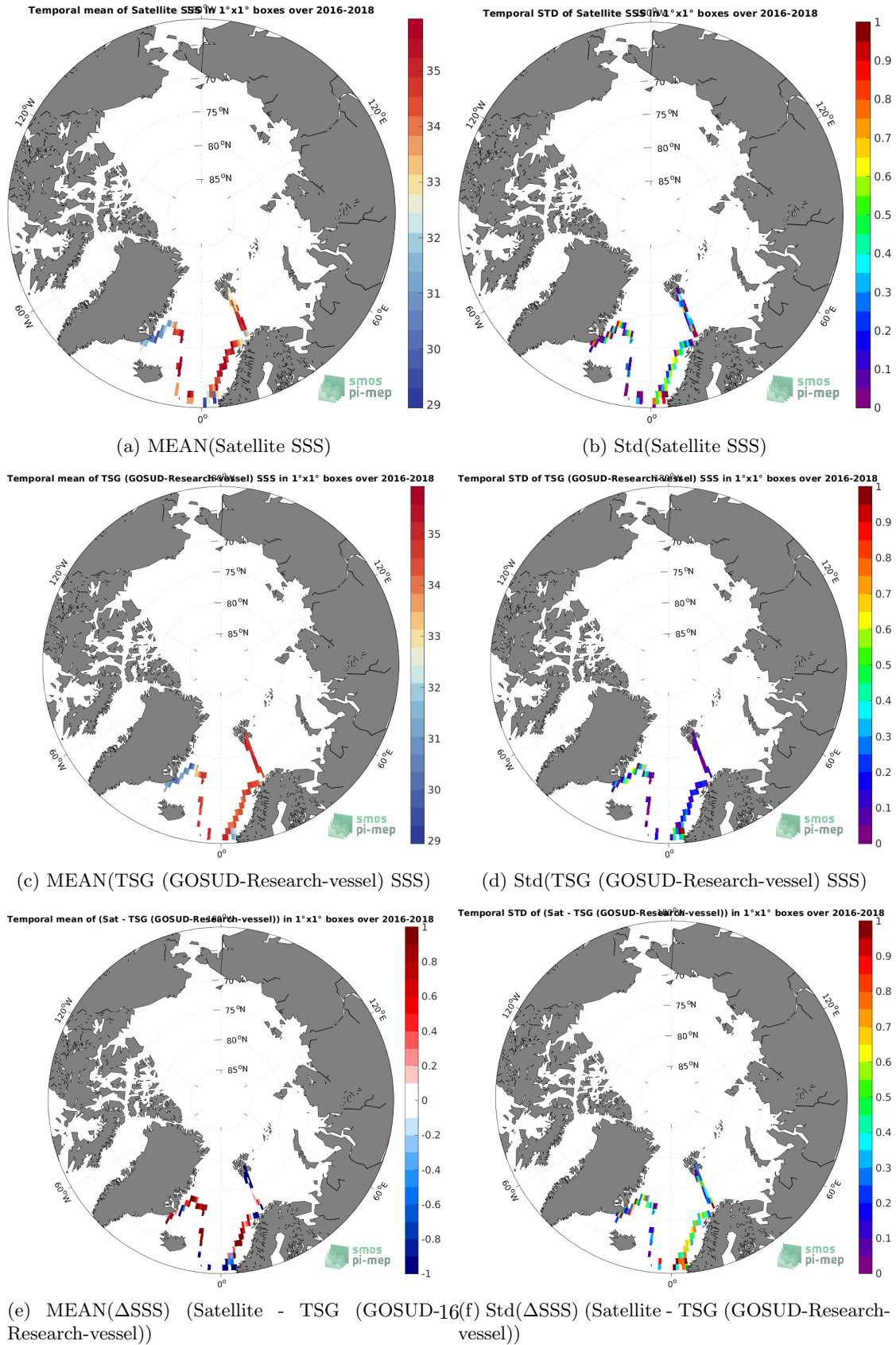
Figure 6: Temporal mean (left) and Std (right) of SSS from SMOS SSS L3 Arctic v1.1 - 7-Day running mean (CATDS-CECOS-LOCEAN) (top), TSG (GOSUD-Research-vessel) (middle), and of \Delta SSS (Satellite - TSG (GOSUD-Research-vessel)). Only match-up pairs are used to generate these maps.
