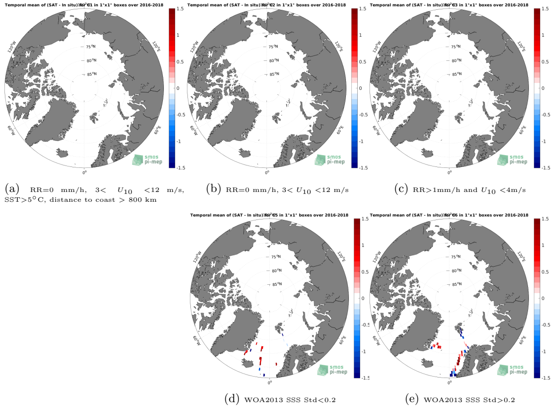
Figure 12: Temporal mean gridded over spatial boxes of size 1^\circ \times 1^\circ of \Delta SSS (SMOS SSS L3 Arctic v1.1 - 7-Day running mean (CATDS-CECOS-LOCEAN) - TSG (GOSUD-Research-vessel)) for 5 different subdatasets corresponding to: RR=0 mm/h, 3 < U_{10} < 12 m/s, SST > 5°C, distance to coast > 800 km (a), RR=0 mm/h, 3 < U_{10} < 12 m/s (b), RR > 1mm/h and U_{10} < 4 m/s (c), WOA2013 SSS Std < 0.2 (d), WOA2013 SSS Std > 0.2 (e).
