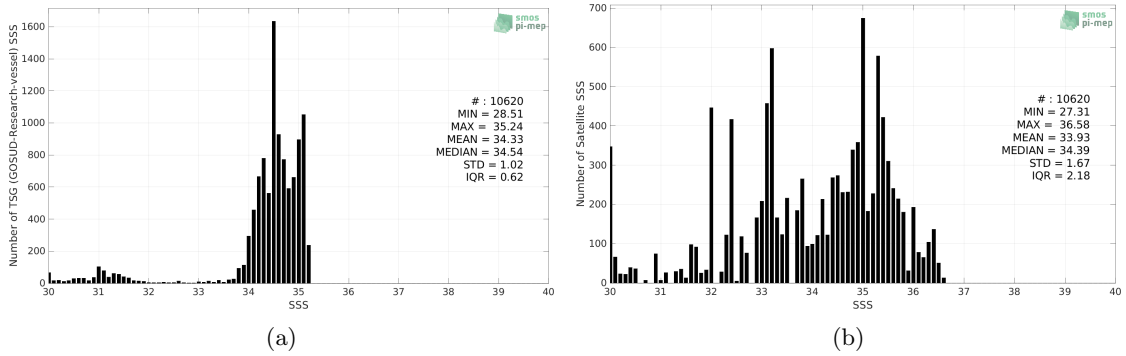
Figure 2: Histograms of SSS from TSG (GOSUD-Research-vessel) (a) and SMOS SSS L3 Arctic v1.1 - 7-Day running mean (CATDS-CECOS-LOCEAN) (b) considering all match-up pairs per bins of 0.1 over the Arctic Ocean Pi-MEP region and for the full satellite product period.
