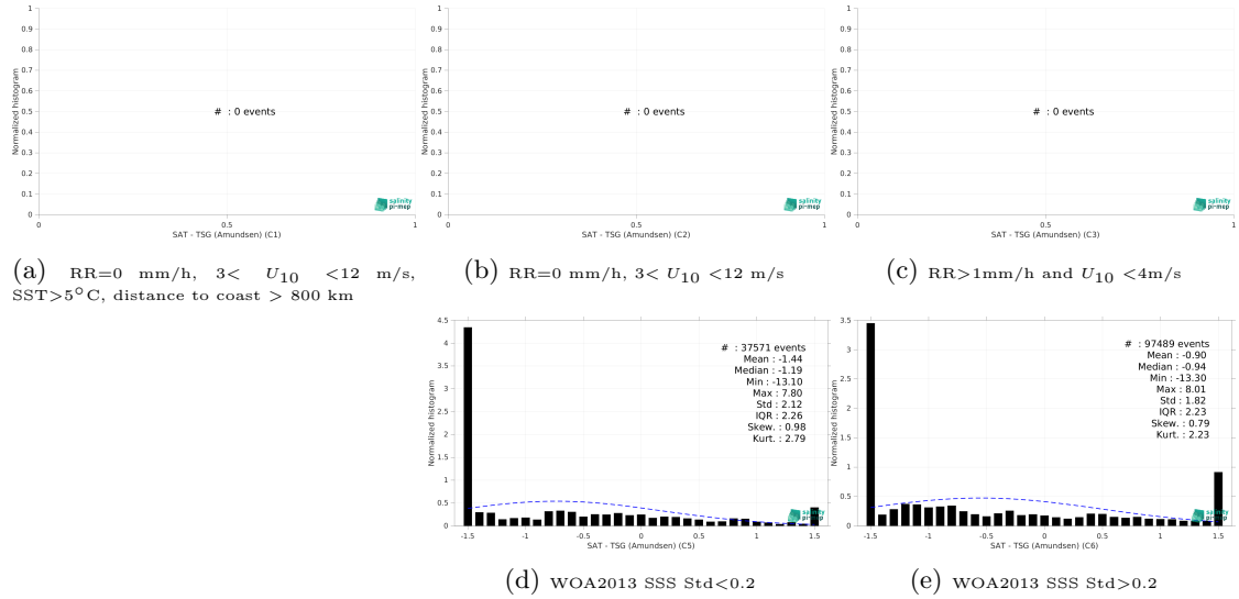
Figure 13: Normalized histogram of \Delta SSS (SMOS SSS L3 Arctic v1.1 - 7-Day runing mean (CATDS-CEC-LOCEAN) - TSG (Amundsen)) for 5 different subdatasets corresponding to: RR=0 mm/h, 3 < U_{10} < 12 m/s, SST>5°C, distance to coast > 800 km (a), RR=0 mm/h, 3 < U_{10} < 12 m/s (b), RR>1mm/h and U_{10} < 4 m/s (c), WOA2013 SSS Std<0.2 (d), WOA2013 SSS Std>0.2 (e).
