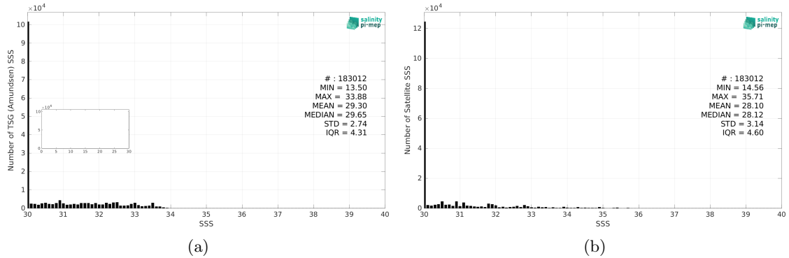
Figure 2: Histograms of SSS from TSG (Amundsen) (a) and SMOS SSS L3 Arctic v1.1 - 7-Day running mean (CATDS-CEC-LOCEAN) (b) considering all match-up pairs per bins of 0.1 over the Arctic Ocean Pi-MEP region and for the full satellite product period.
