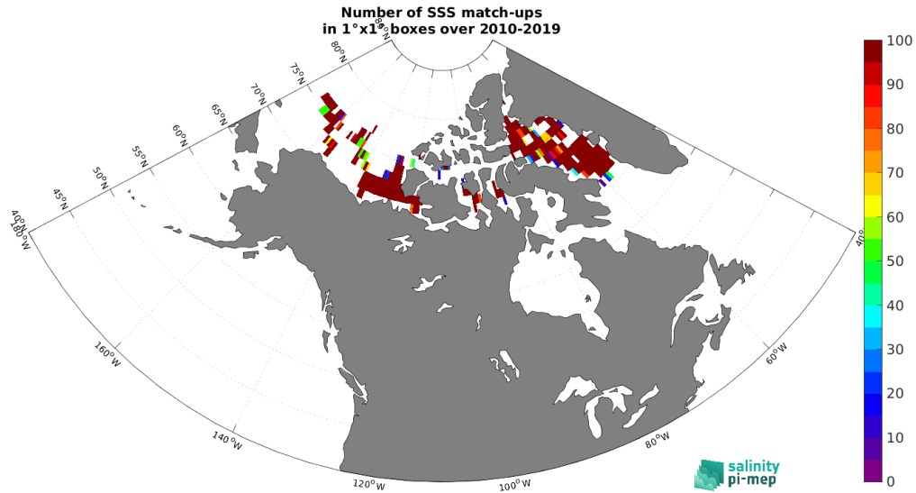
Figure 4: Number of SSS match-ups between TSG (Amundsen) SSS and the SMOS SSS L3 Arctic v1.1 - 7-Day running mean (CATDS-CEC-LOCEAN) SSS product for the Arctic Ocean Pi-MEP region over 1°x1° boxes and for the full satellite product period.
