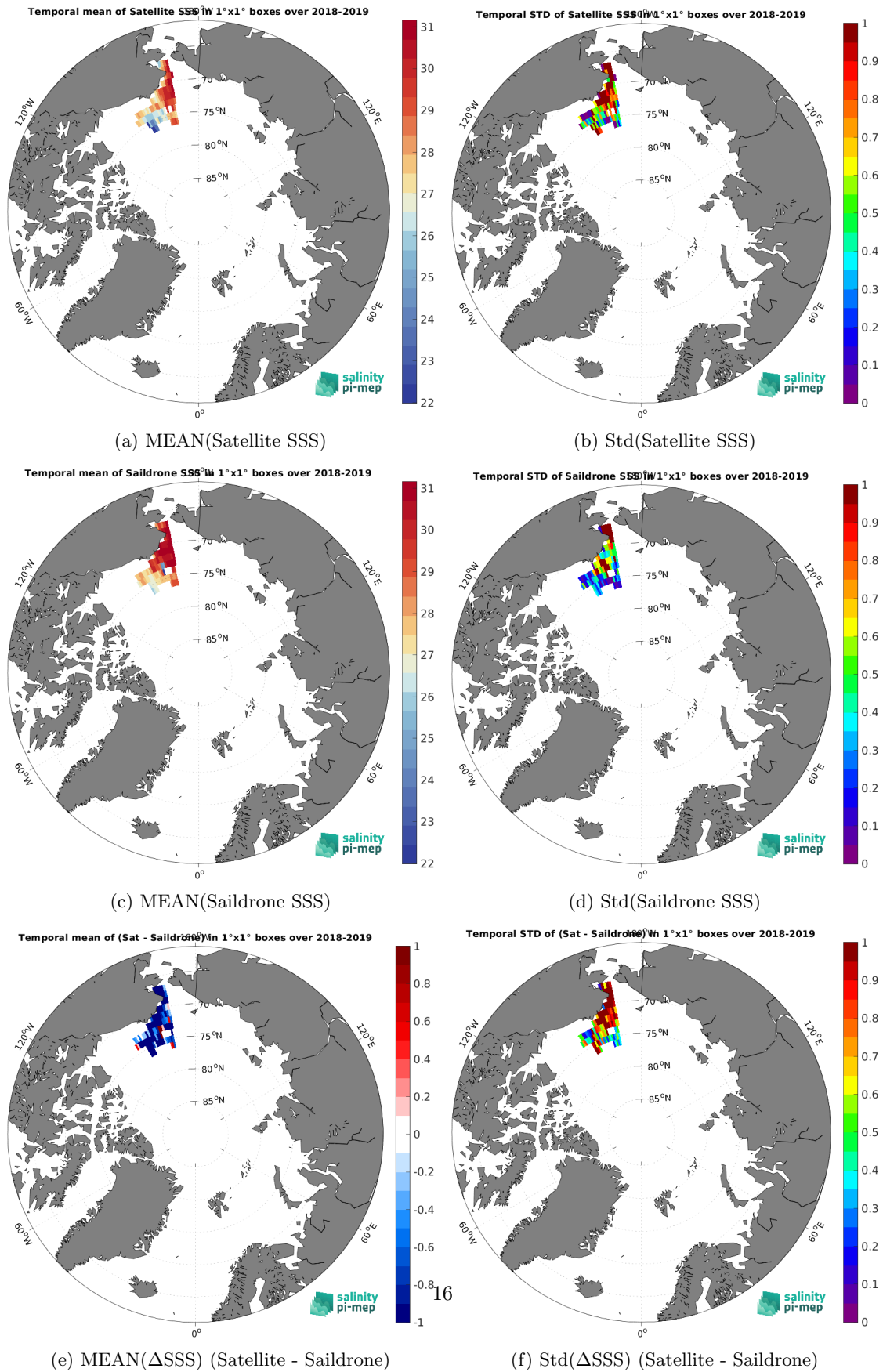
Figure 6: Temporal mean (left) and Std (right) of SSS from SMOS SSS L3 Arctic v1.1 - 7-Day running mean (CATDS-CEC-LOCEAN) (top), Saildrone (middle), and of \Delta SSS (Satellite - Saildrone). Only match-up pairs are used to generate these maps.
