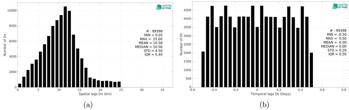
Figure 5: Histograms of the spatial (a) and temporal (b) lags between the location/time of the Sairdrone measurement and the date of the corresponding SMOS SSS L3 Arctic v1.1 - 7-Day running mean (CATDS-CEC-LOCEAN) SSS pixel.
