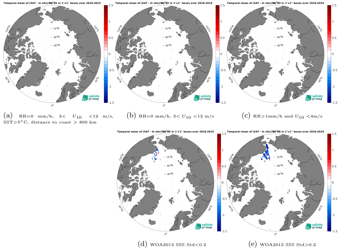
Figure 12: Temporal mean gridded over spatial boxes of size 1^{\circ}\times 1^{\circ} of \Delta\text{SSS} (SMOS SSS L3 Arctic v1.1 - 7-Day running mean (CATDS-CEC-LOCEAN) - Saildrone) for 5 different subdatasets corresponding to: RR=0 mm/h, 3 < U_{10} < 12 m/s, SST > 5^{\circ}\text{C} , distance to coast > 800 km (a), RR=0 mm/h, 3 < U_{10} < 12 m/s (b), RR > 1 mm/h and U_{10} < 4 m/s (c), WOA2013 SSS Std < 0.2 (d), WOA2013 SSS Std > 0.2 (e).
