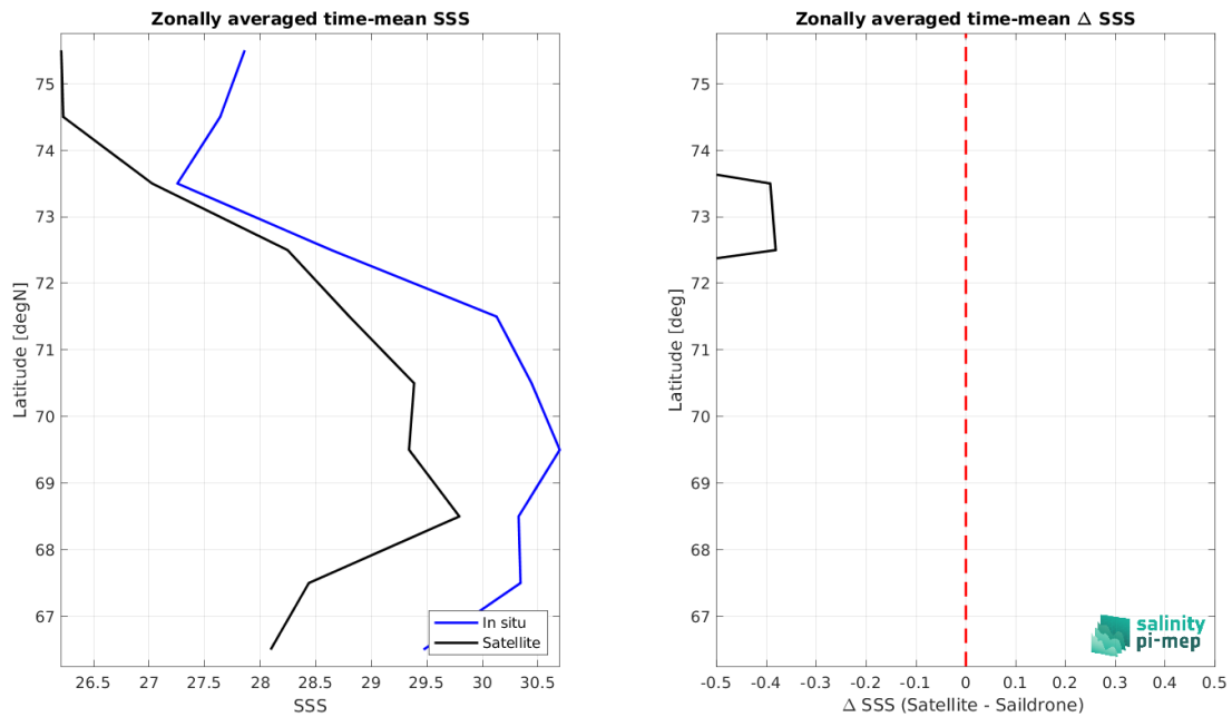
Figure 8: Left panel: Zonal mean SSS from SMOS SSS L3 Arctic v1.1 - 7-Day running mean (CATDS-CEC-LOCEAN) satellite product (black) and from Saildrone (blue). Right panel: Zonal mean of \Delta SSS (Satellite - Saildrone) for all the collected Pi-MEP match-up pairs estimated over the full satellite product period.
