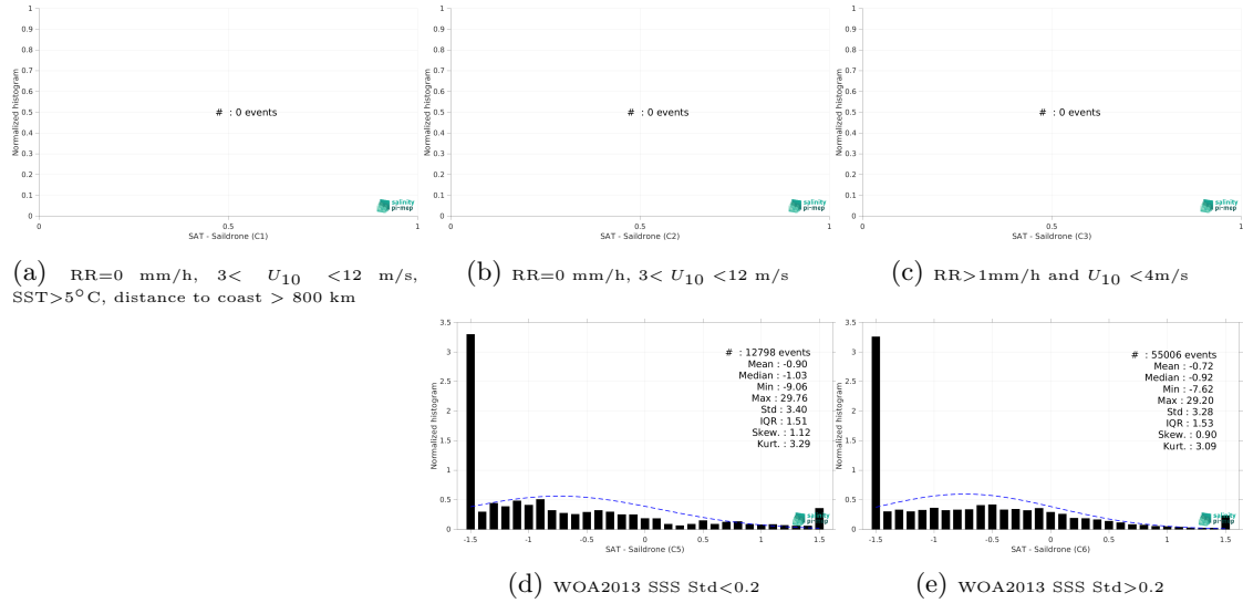
Figure 13: Normalized histogram of \Delta SSS (SMOS SSS L3 Arctic v1.1 - 7-Day runing mean (CATDS-CEC-LOCEAN) - Saildrone) for 5 different subdatasets corresponding to: RR=0 mm/h, 3 < U_{10} < 12 m/s, SST > 5°C, distance to coast > 800 km (a), RR=0 mm/h, 3 < U_{10} < 12 m/s (b), RR > 1mm/h and U_{10} < 4 m/s (c), WOA2013 SSS Std < 0.2 (d), WOA2013 SSS Std > 0.2 (e).
