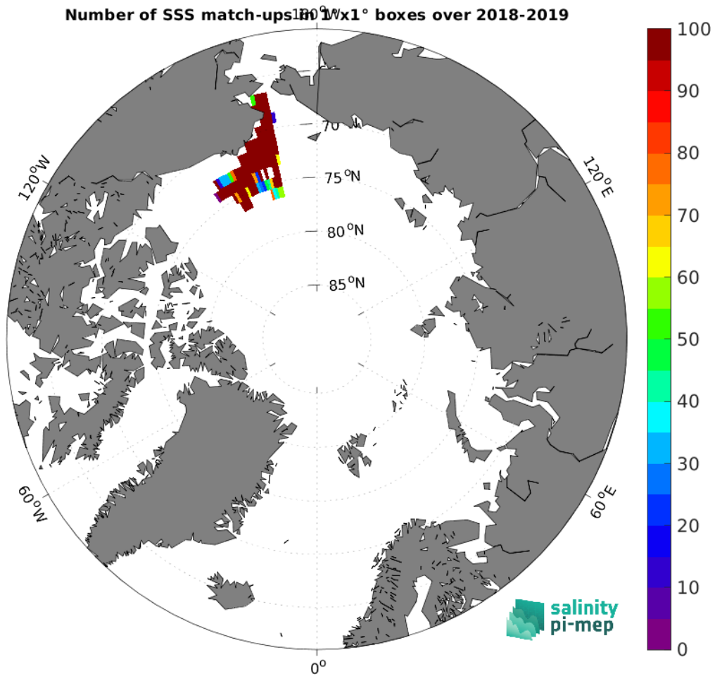
Figure 4: Number of SSS match-ups between Saildrone SSS and the SMOS SSS L3 Arctic v1.1 - 7-Day running mean (CATDS-CEC-LOCEAN) SSS product for the Arctic Ocean Pi-MEP region over 1^\circ \times 1^\circ boxes and for the full satellite product period.
