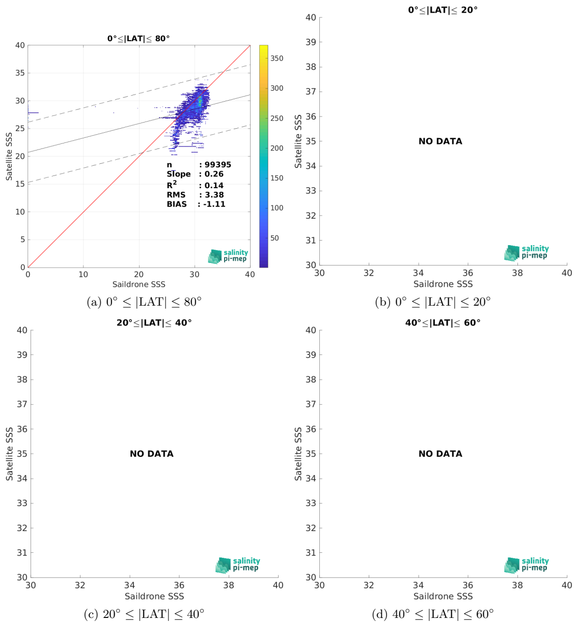
Figure 9: Contour maps of the concentration of SMOS SSS L3 Arctic v1.1 - 7-Day running mean (CATDS-CEC-LOCEAN) SSS (y-axis) versus Saildrone SSS (x-axis) at match-up pairs for different latitude bands. For each plot, the red line shows x=y . The black thin and dashed lines indicate a linear fit through the data cloud and the \pm 95\% confidence levels, respectively. The number match-up pairs n , the slope and R^2 coefficient of the linear fit, the root mean square (RMS) and the mean bias between satellite and in situ data are indicated for each latitude band in each plots.
