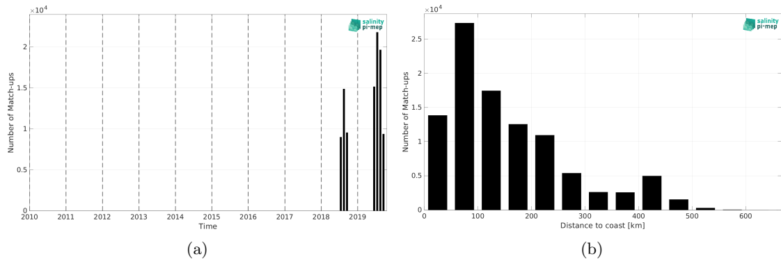
Figure 1: Number of match-ups between Saildrone and SMOS SSS L3 Arctic v1.1 - 7-Day running mean (CATDS-CEC-LOCEAN) SSS as a function of time (a) and as function of the distance to coast (b) over the Arctic Ocean Pi-MEP region and for the full satellite product period.
