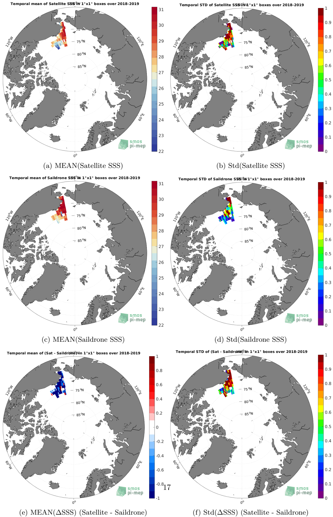
Figure 6: Temporal mean (left) and Std (right) of SSS from SMOS SSS L3 Arctic v1.1 - 7-Day running mean (CATDS-CECOS-LOCEAN) (top), Saildrone (middle), and of \Delta SSS (Satellite - Saildrone). Only match-up pairs are used to generate these maps.
