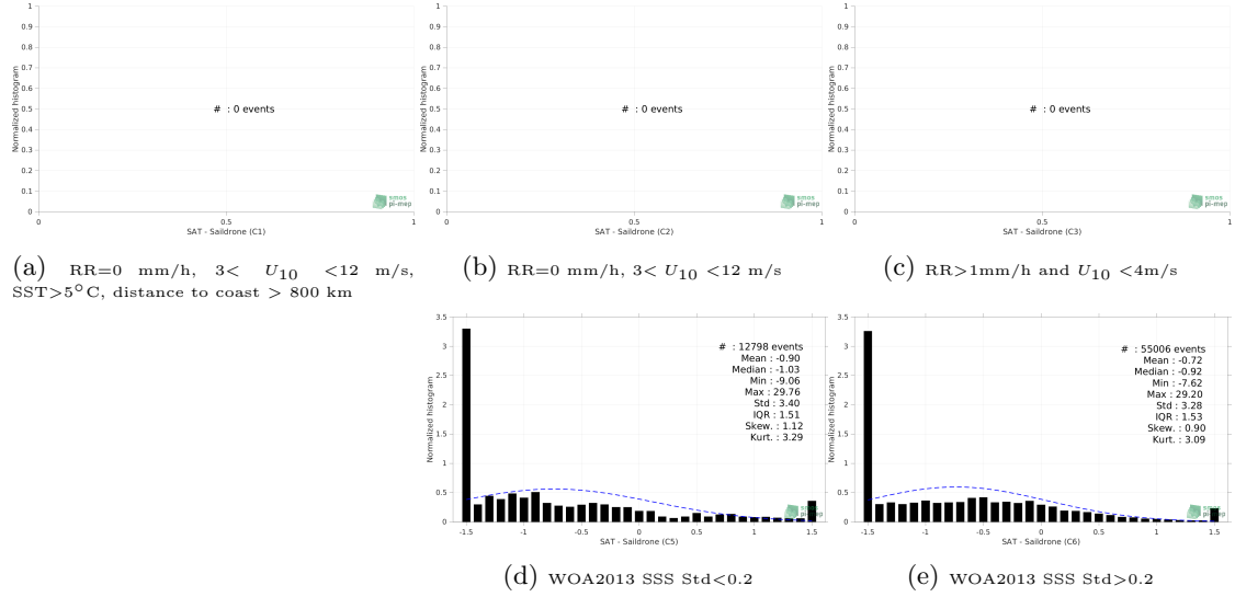
Figure 13: Normalized histogram of \Delta SSS (SMOS SSS L3 Arctic v1.1 - 7-Day running mean (CATDS-CECOS-LOCEAN) - Sairdrone) for 5 different subdatasets corresponding to: RR=0 mm/h, 3 < U_{10} < 12 m/s, SST > 5°C, distance to coast > 800 km (a), RR=0 mm/h, 3 < U_{10} < 12 m/s (b), RR > 1mm/h and U_{10} < 4 m/s (c), WOA2013 SSS Std < 0.2 (d), WOA2013 SSS Std > 0.2 (e).
