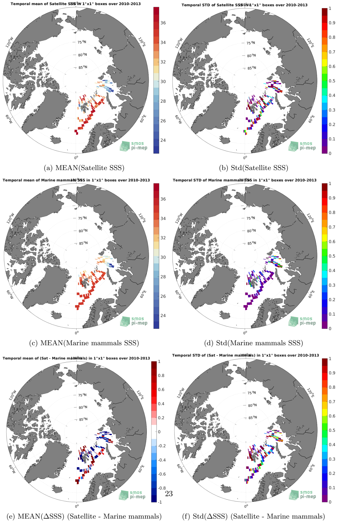
Figure 6: Temporal mean (left) and Std (right) of SSS from SMOS SSS L3 Arctic v1.1 - 7-Day running mean (CATDS-CECOS-LOCEAN) (top), Marine mammals (middle), and of \Delta SSS (Satellite - Marine mammals). Only match-up pairs are used to generate these maps.
