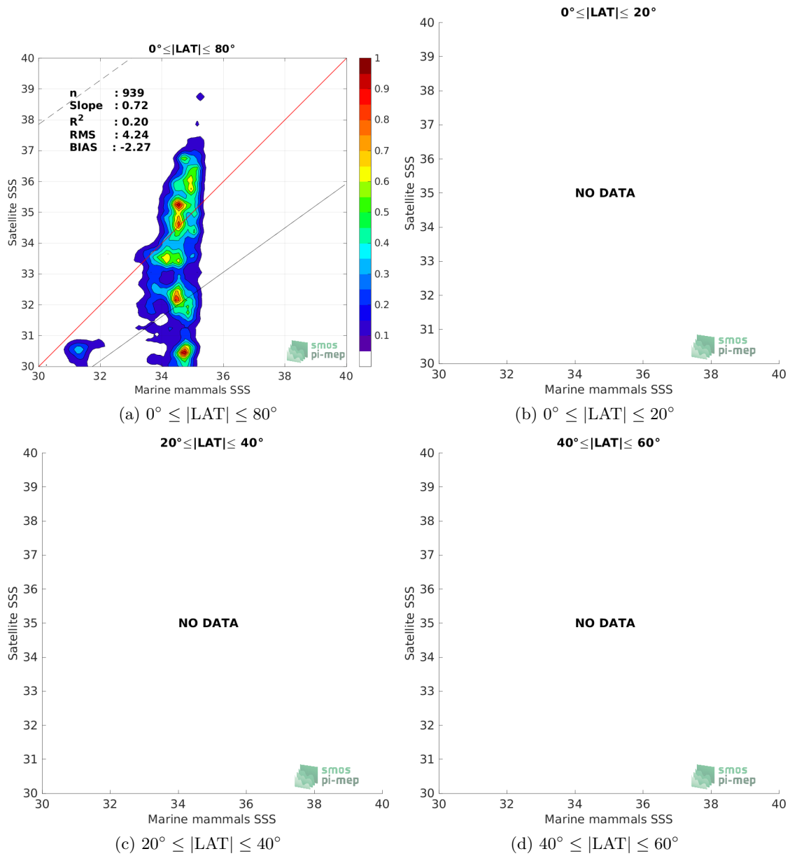
Figure 9: Contour maps of the concentration of SMOS SSS L3 Arctic v1.1 - 7-Day running mean (CATDS-CECOS-LOCEAN) SSS (y-axis) versus Marine mammals SSS (x-axis) at match-up pairs for different latitude bands. For each plot, the red line shows x=y . The black thin and dashed lines indicate a linear fit through the data cloud and the \pm 95\% confidence levels, respectively. The number match-up pairs n , the slope and R^2 coefficient of the linear fit, the root mean square (RMS) and the mean bias between satellite and in situ data are indicated for each latitude band in each plots.
