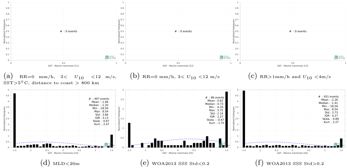
Figure 13: Normalized histogram of \Delta SSS (SMOS SSS L3 Arctic v1.1 - 7-Day running mean (CATDS-CECOS-LOCEAN) - Marine mammals) for 6 different subdatasets corresponding to: RR=0 mm/h, 3 < U_{10} < 12 m/s, SST>5°C, distance to coast > 800 km (a), RR=0 mm/h, 3 < U_{10} < 12 m/s (b), RR>1mm/h and U_{10} < 4 m/s (c), MLD<20m (d), WOA2013 SSS Std<0.2 (e), WOA2013 SSS Std>0.2 (f).
