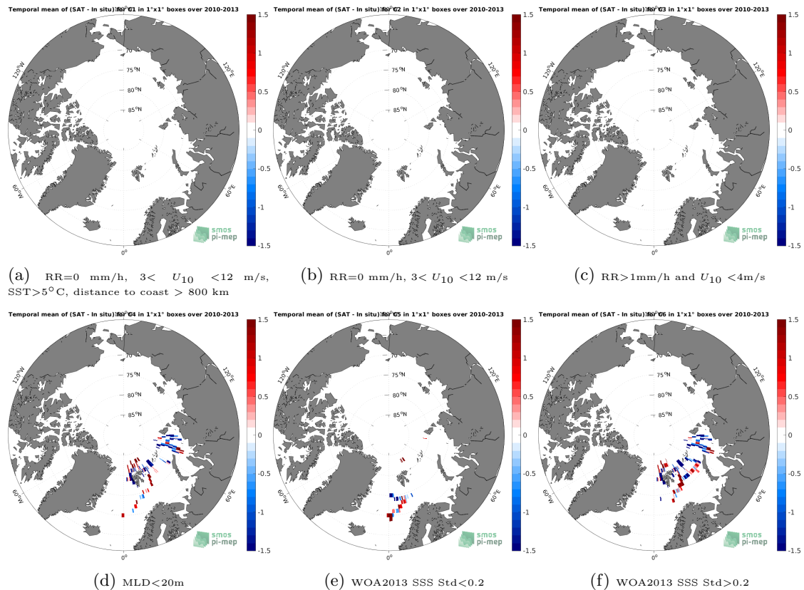
Figure 12: Temporal mean gridded over spatial boxes of size 1^{\circ}\times 1^{\circ} of \Delta\text{SSS} (SMOS SSS L3 Arctic v1.1 - 7-Day running mean (CATDS-CECOS-LOCEAN) - Marine mammals) for 6 different subdatasets corresponding to:RR=0 mm/h, 3 < U_{10} < 12 m/s, SST >5^{\circ}\text{C} , distance to coast > 800 km (a), RR=0 mm/h, 3 < U_{10} < 12 m/s (b), RR >1 mm/h and U_{10} < 4 m/s (c),MLD <20 m (d),WOA2013 SSS Std <0.2 (e),WOA2013 SSS Std >0.2 (f).
