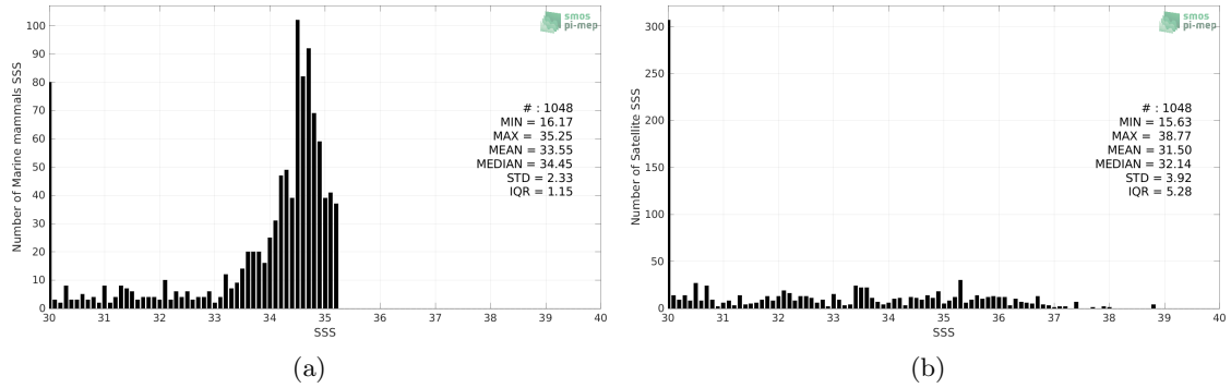
Figure 2: Histograms of SSS from Marine mammals (a) and SMOS SSS L3 Arctic v1.1 - 7-Day running mean (CATDS-CECOS-LOCEAN) (b) considering all match-up pairs per bins of 0.1 over the Arctic Ocean Pi-MEP region and for the full satellite product period.
