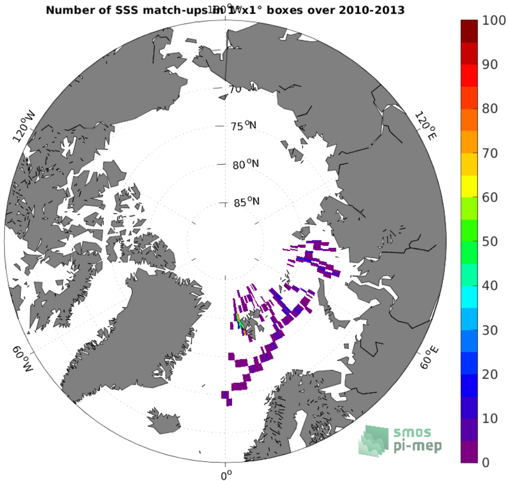
Figure 4: Number of SSS match-ups between Marine mammals SSS and the SMOS SSS L3 Arctic v1.1 - 7-Day running mean (CATDS-CECOS-LOCEAN) SSS product for the Arctic Ocean Pi-MEP region over 1^\circ \times 1^\circ boxes and for the full satellite product period.
