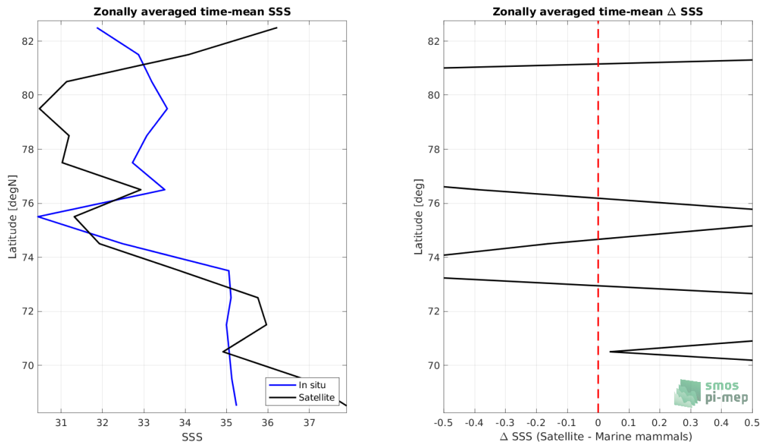
Figure 8: Left panel: Zonal mean SSS from SMOS SSS L3 Arctic v1.1 - 7-Day running mean (CATDS-CECOS-LOCEAN) satellite product (black) and from Marine mammals (blue). Right panel: Zonal mean of \Delta SSS (Satellite - Marine mammals) for all the collected Pi-MEP match-up pairs estimated over the full satellite product period.
