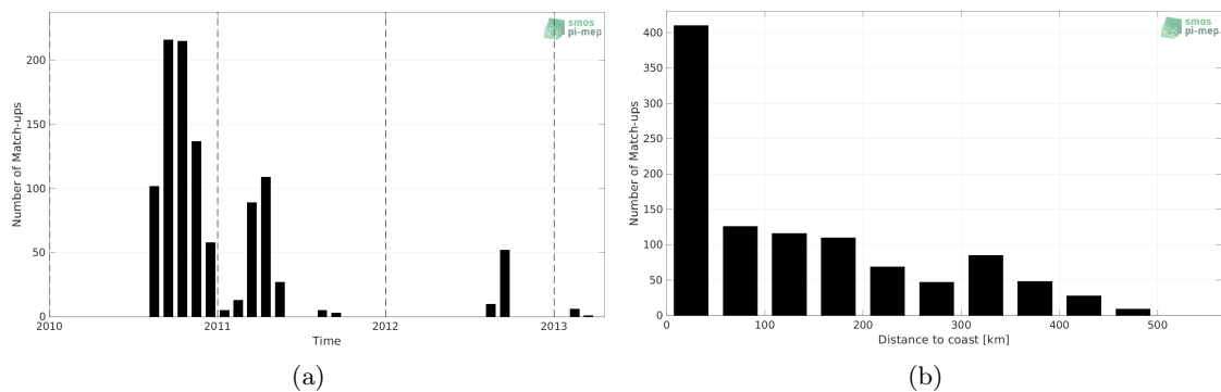
Figure 1: Number of match-ups between Marine mammals and SMOS SSS L3 Arctic v1.1 - 7-Day running mean (CATDS-CECOS-LOCEAN) SSS as a function of time (a) and as function of the distance to coast (b) over the Arctic Ocean Pi-MEP region and for the full satellite product period.
