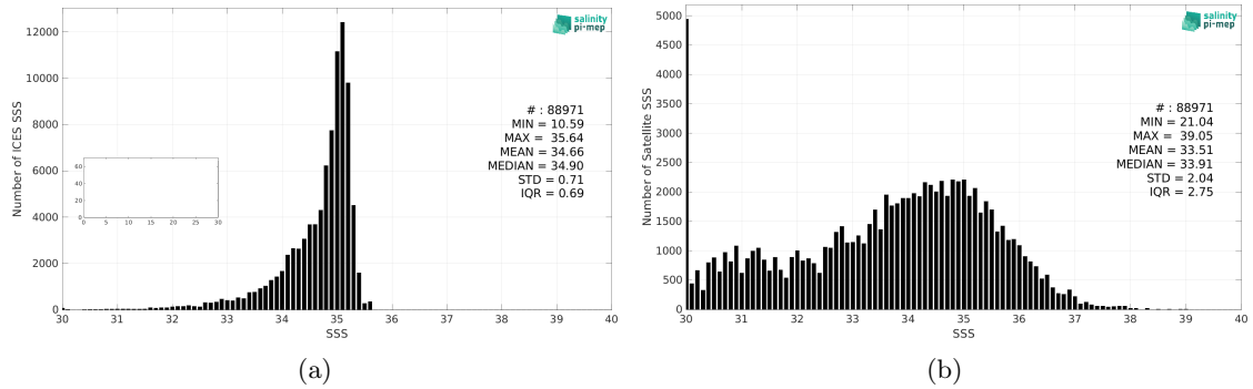
Figure 2: Histograms of SSS from ICES (a) and SMOS SSS L3 Arctic v1.1 - 7-Day running mean (CATDS-CEC-LOCEAN) (b) considering all match-up pairs per bins of 0.1 over the Arctic Ocean Pi-MEP region and for the full satellite product period.
