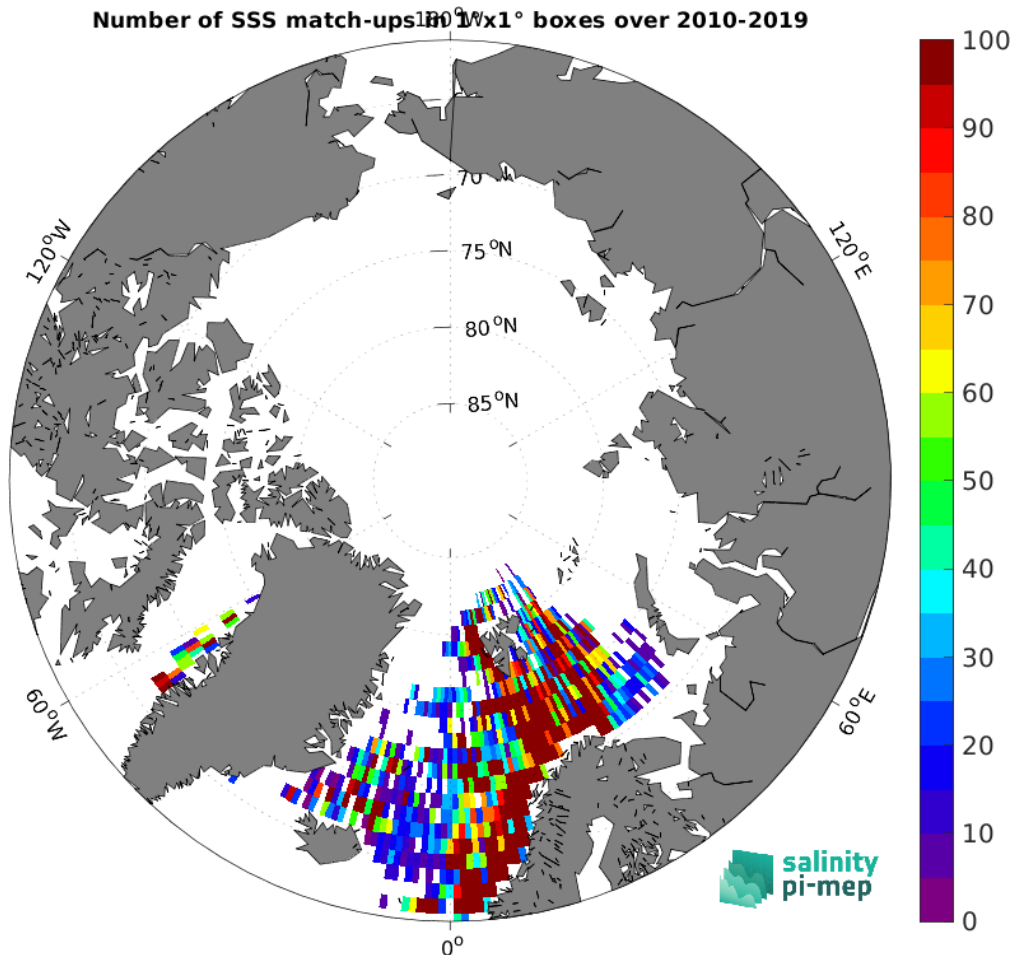
Figure 4: Number of SSS match-ups between ICES SSS and the SMOS SSS L3 Arctic v1.1 - 7-Day running mean (CATDS-CEC-LOCEAN) SSS product for the Arctic Ocean Pi-MEP region over 1^\circ \times 1^\circ boxes and for the full satellite product period.
