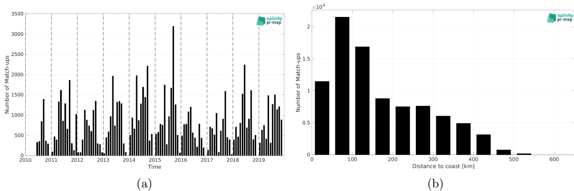
Figure 1: Number of match-ups between ICES and SMOS SSS L3 Arctic v1.1 - 7-Day running mean (CATDS-CEC-LOCEAN) SSS as a function of time (a) and as function of the distance to coast (b) over the Arctic Ocean Pi-MEP region and for the full satellite product period.
