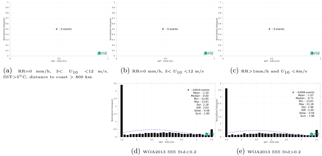
Figure 13: Normalized histogram of \Delta SSS (SMOS SSS L3 Arctic v1.1 - 7-Day runing mean (CATDS-CEC-LOCEAN) - ICES) for 5 different subdatasets corresponding to: RR=0 mm/h, 3 < U_{10} < 12 m/s, SST>5°C, distance to coast > 800 km (a), RR=0 mm/h, 3 < U_{10} < 12 m/s (b), RR>1mm/h and U_{10} < 4 m/s (c), WOA2013 SSS Std<0.2 (d), WOA2013 SSS Std>0.2 (e).
