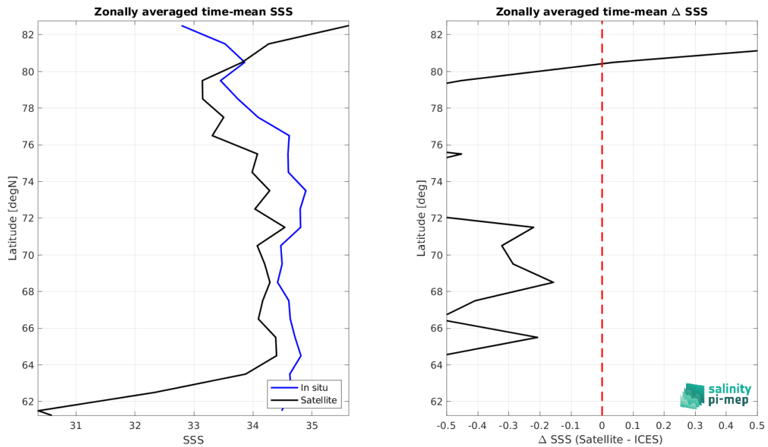
Figure 8: Left panel: Zonal mean SSS from SMOS SSS L3 Arctic v1.1 - 7-Day running mean (CATDS-CEC-LOCEAN) satellite product (black) and from ICES (blue). Right panel: Zonal mean of \Delta SSS (Satellite - ICES) for all the collected Pi-MEP match-up pairs estimated over the full satellite product period.
