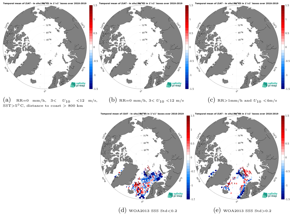
Figure 12: Temporal mean gridded over spatial boxes of size 1^{\circ}\times 1^{\circ} of \Delta\text{SSS} (SMOS SSS L3 Arctic v1.1 - 7-Day running mean (CATDS-CEC-LOCEAN) - ICES) for 5 different subdatasets corresponding to:RR=0 mm/h, 3 < U_{10} < 12 m/s, SST >5^{\circ}\text{C} , distance to coast > 800 km (a), RR=0 mm/h, 3 < U_{10} < 12 m/s (b), RR >1 mm/h and U_{10} < 4 m/s (c), WOA2013 SSS Std <0.2 (d), WOA2013 SSS Std >0.2 (e).
