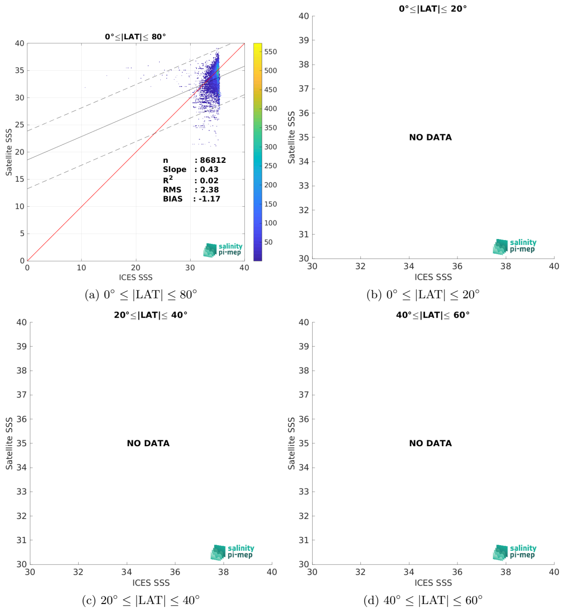
Figure 9: Contour maps of the concentration of SMOS SSS L3 Arctic v1.1 - 7-Day running mean (CATDS-CEC-LOCEAN) SSS (y-axis) versus ICES SSS (x-axis) at match-up pairs for different latitude bands. For each plot, the red line shows x=y . The black thin and dashed lines indicate a linear fit through the data cloud and the \pm 95\% confidence levels, respectively. The number match-up pairs n , the slope and R^2 coefficient of the linear fit, the root mean square (RMS) and the mean bias between satellite and in situ data are indicated for each latitude band in each plots.
