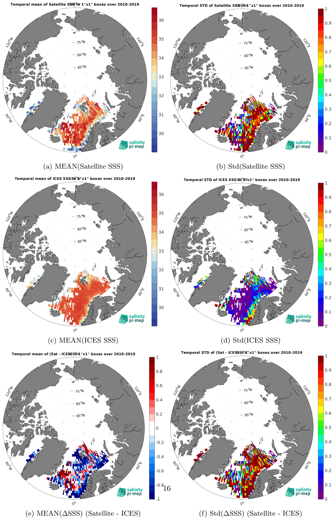
Figure 6: Temporal mean (left) and Std (right) of SSS from SMOS SSS L3 Arctic v1.1 - 7-Day running mean (CATDS-CEC-LOCEAN) (top), ICES (middle), and of \Delta SSS (Satellite - ICES). Only match-up pairs are used to generate these maps.
