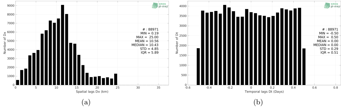
Figure 5: Histograms of the spatial (a) and temporal (b) lags between the location/time of the ICES measurement and the date of the corresponding SMOS SSS L3 Arctic v1.1 - 7-Day running mean (CATDS-CECOS-LOCEAN) SSS pixel.
