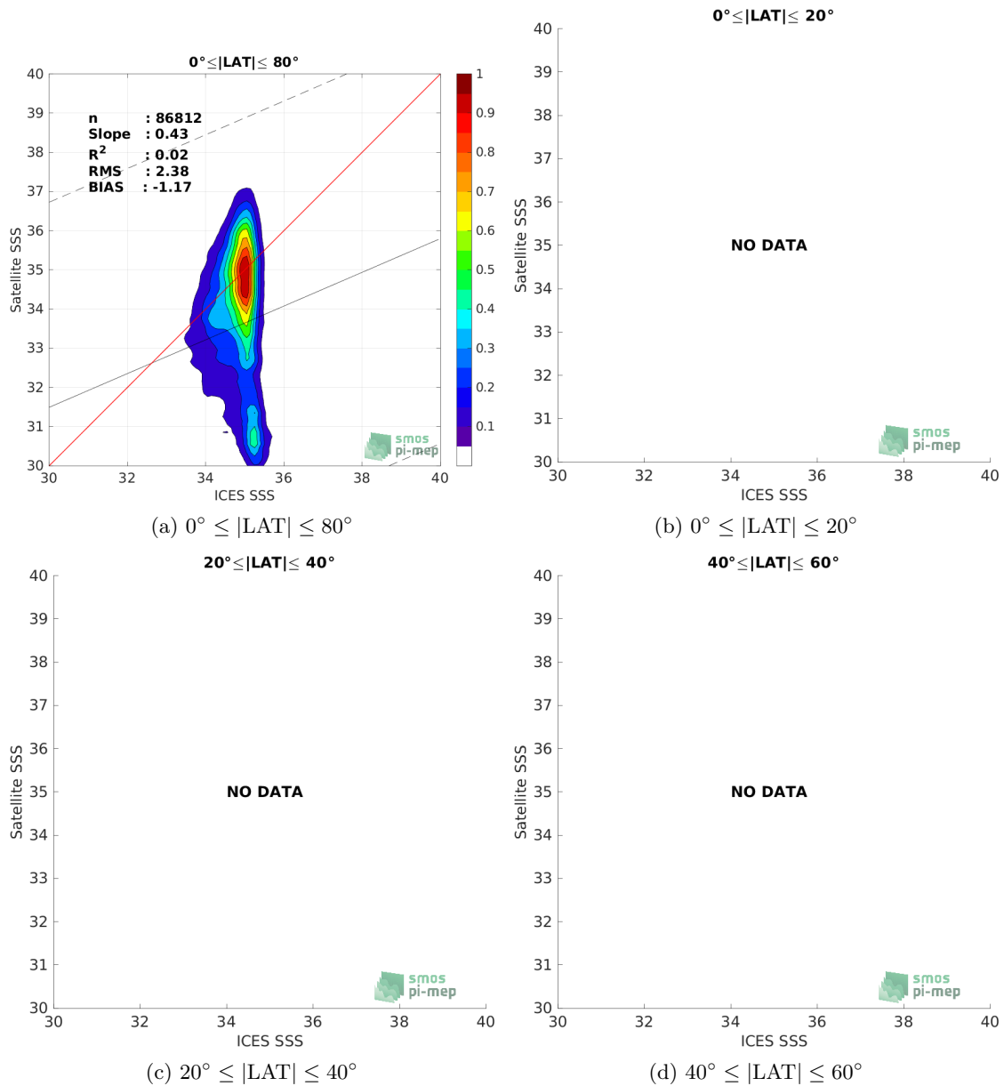
Figure 9: Contour maps of the concentration of SMOS SSS L3 Arctic v1.1 - 7-Day running mean (CATDS-CECOS-LOCEAN) SSS (y-axis) versus ICES SSS (x-axis) at match-up pairs for different latitude bands. For each plot, the red line shows x=y . The black thin and dashed lines indicate a linear fit through the data cloud and the \pm 95\% confidence levels, respectively. The number match-up pairs n , the slope and R^2 coefficient of the linear fit, the root mean square (RMS) and the mean bias between satellite and in situ data are indicated for each latitude band in each plots.
