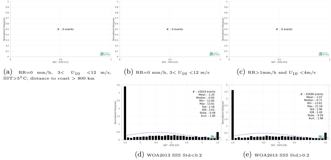
Figure 13: Normalized histogram of \Delta SSS (SMOS SSS L3 Arctic v1.1 - 7-Day running mean (CATDS-CECOS-LOCEAN) - ICES) for 5 different subdatasets corresponding to: RR=0 mm/h, 3 < U_{10} < 12 m/s, SST > 5°C, distance to coast > 800 km (a), RR=0 mm/h, 3 < U_{10} < 12 m/s (b), RR > 1mm/h and U_{10} < 4 m/s (c), WOA2013 SSS Std < 0.2 (d), WOA2013 SSS Std > 0.2 (e).
