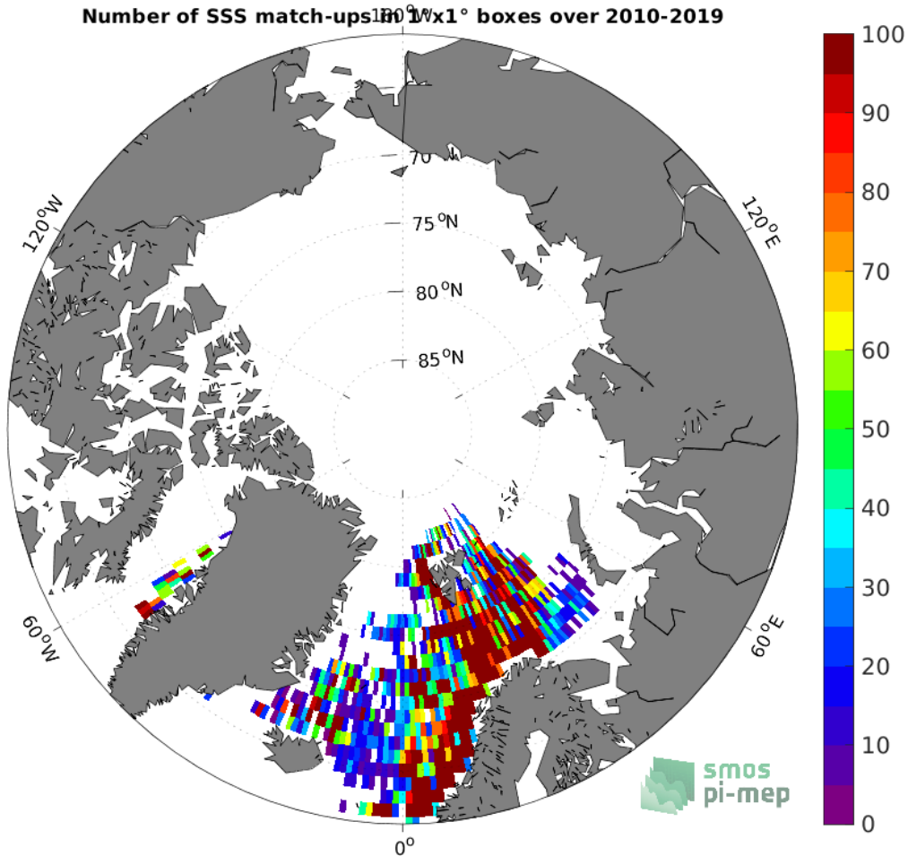
Figure 4: Number of SSS match-ups between ICES SSS and the SMOS SSS L3 Arctic v1.1 - 7-Day running mean (CATDS-CECOS-LOCEAN) SSS product for the Arctic Ocean Pi-MEP region over 1^\circ \times 1^\circ boxes and for the full satellite product period.
