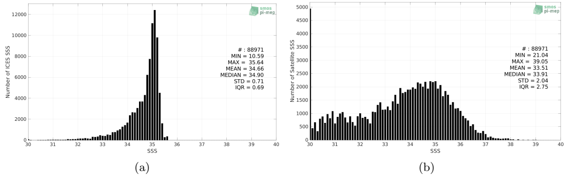
Figure 2: Histograms of SSS from ICES (a) and SMOS SSS L3 Arctic v1.1 - 7-Day running mean (CATDS-CECOS-LOCEAN) (b) considering all match-up pairs per bins of 0.1 over the Arctic Ocean Pi-MEP region and for the full satellite product period.
