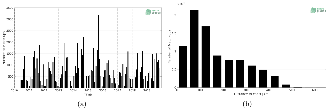
Figure 1: Number of match-ups between ICES and SMOS SSS L3 Arctic v1.1 - 7-Day running mean (CATDS-CECOS-LOCEAN) SSS as a function of time (a) and as function of the distance to coast (b) over the Arctic Ocean Pi-MEP region and for the full satellite product period.
