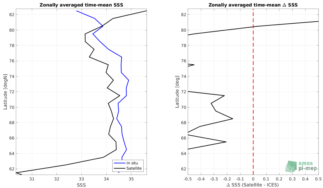
Figure 8: Left panel: Zonal mean SSS from SMOS SSS L3 Arctic v1.1 - 7-Day running mean (CATDS-CECOS-LOCEAN) satellite product (black) and from ICES (blue). Right panel: Zonal mean of \Delta SSS (Satellite - ICES) for all the collected Pi-MEP match-up pairs estimated over the full satellite product period.
