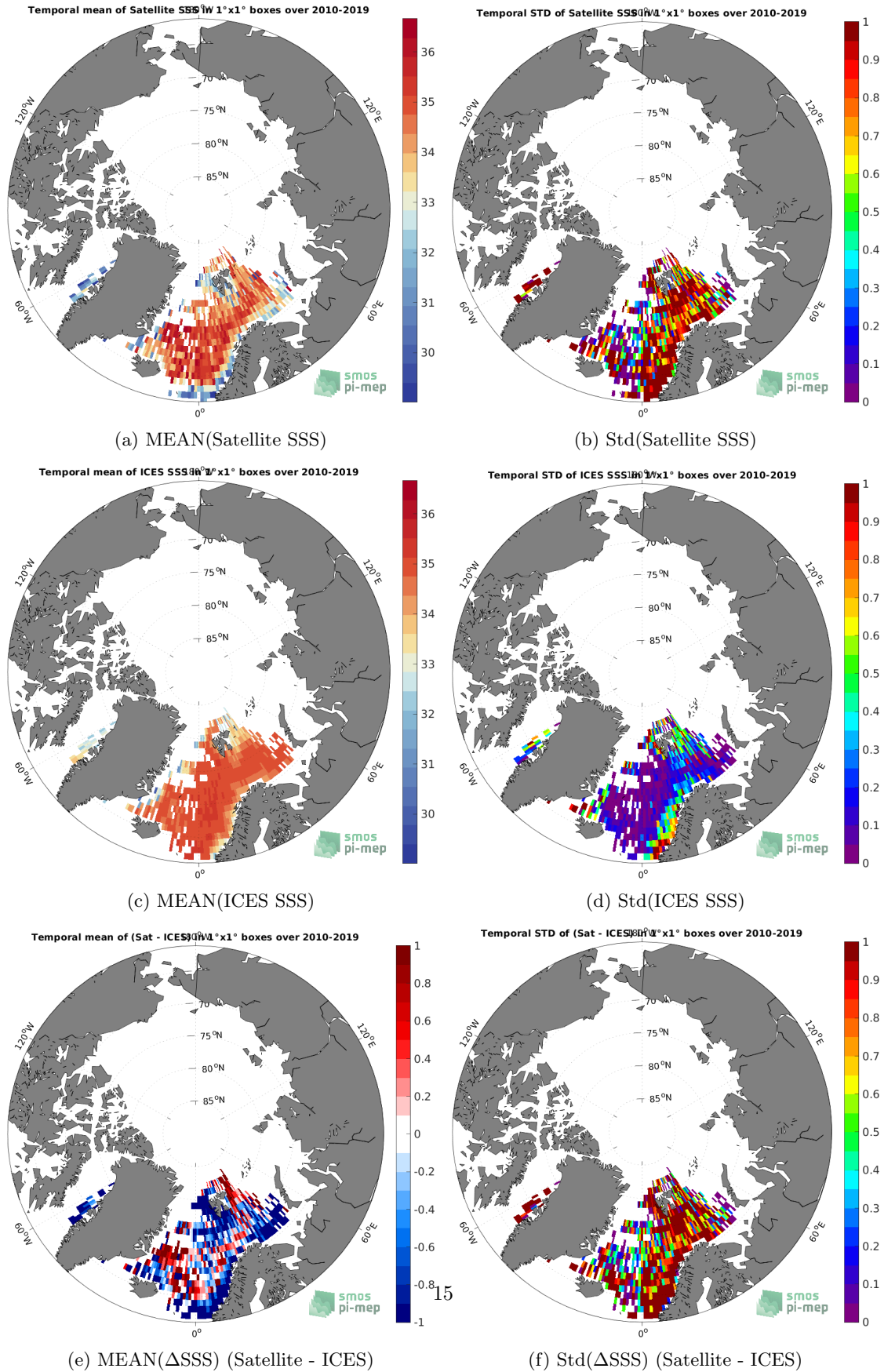
Figure 6: Temporal mean (left) and Std (right) of SSS from SMOS SSS L3 Arctic v1.1 - 7-Day running mean (CATDS-CECOS-LOCEAN) (top), ICES (middle), and of \Delta SSS (Satellite - ICES). Only match-up pairs are used to generate these maps.
