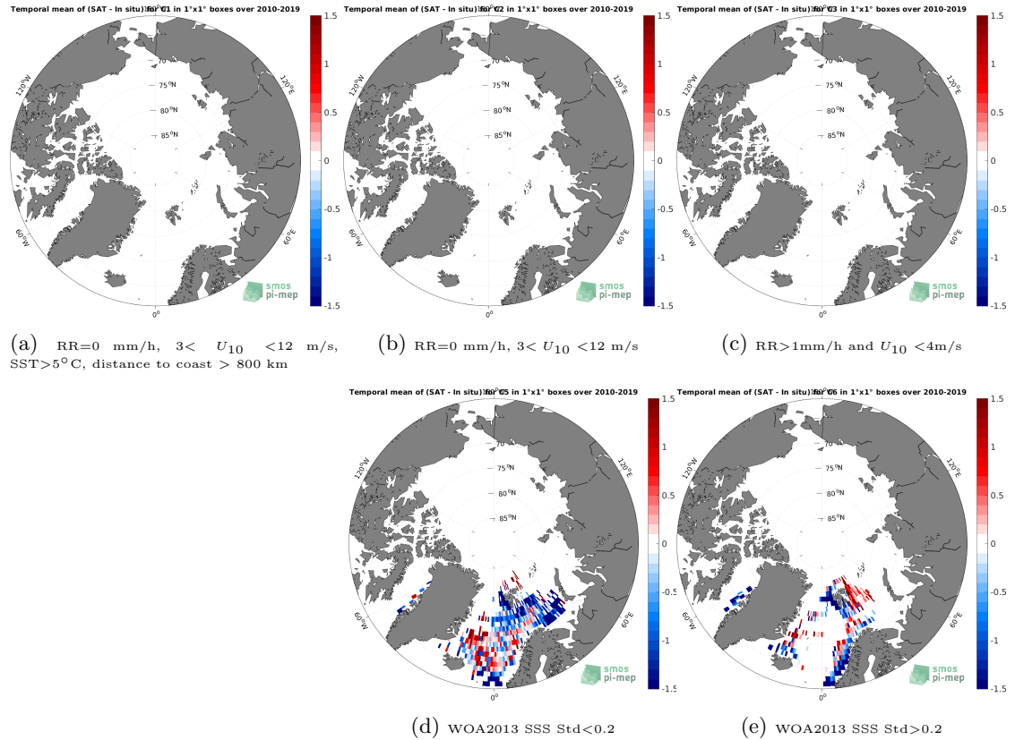
Figure 12: Temporal mean gridded over spatial boxes of size 1^{\circ}\times 1^{\circ} of \Delta\text{SSS} (SMOS SSS L3 Arctic v1.1 - 7-Day running mean (CATDS-CECOS-LOCEAN) - ICES) for 5 different subdatasets corresponding to:RR=0 mm/h, 3 < U_{10} < 12 m/s, SST >5^{\circ}\text{C} , distance to coast > 800 km (a), RR=0 mm/h, 3 < U_{10} < 12 m/s (b), RR >1 mm/h and U_{10} < 4 m/s (c), WOA2013 SSS Std <0.2 (d), WOA2013 SSS Std >0.2 (e).
