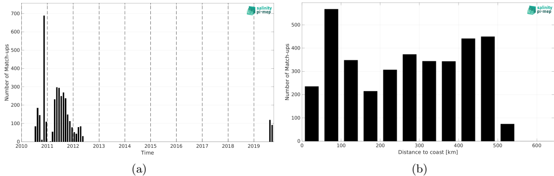
Figure 1: Number of match-ups between Surface drifters and SMOS SSS L3 Arctic v1.1 - 7-Day running mean (CATDS-CEC-LOCEAN) SSS as a function of time (a) and as function of the distance to coast (b) over the Arctic Ocean Pi-MEP region and for the full satellite product period.
