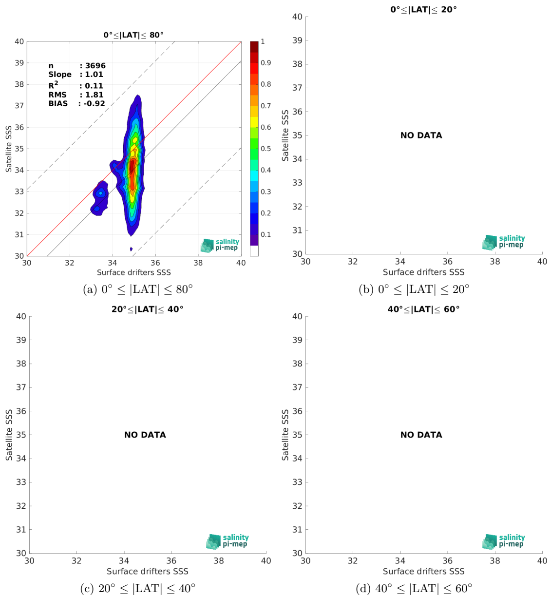
Figure 8: Contour maps of the concentration of SMOS SSS L3 Arctic v1.1 - 7-Day running mean (CATDS-CEC-LOCEAN) SSS (y-axis) versus Surface drifters SSS (x-axis) at match-up pairs for different latitude bands. For each plot, the red line shows x=y . The black thin and dashed lines indicate a linear fit through the data cloud and the \pm 95\% confidence levels, respectively. The number match-up pairs n , the slope and R^2 coefficient of the linear fit, the root mean square (RMS) and the mean bias between satellite and in situ data are indicated for each latitude band in each plots.
