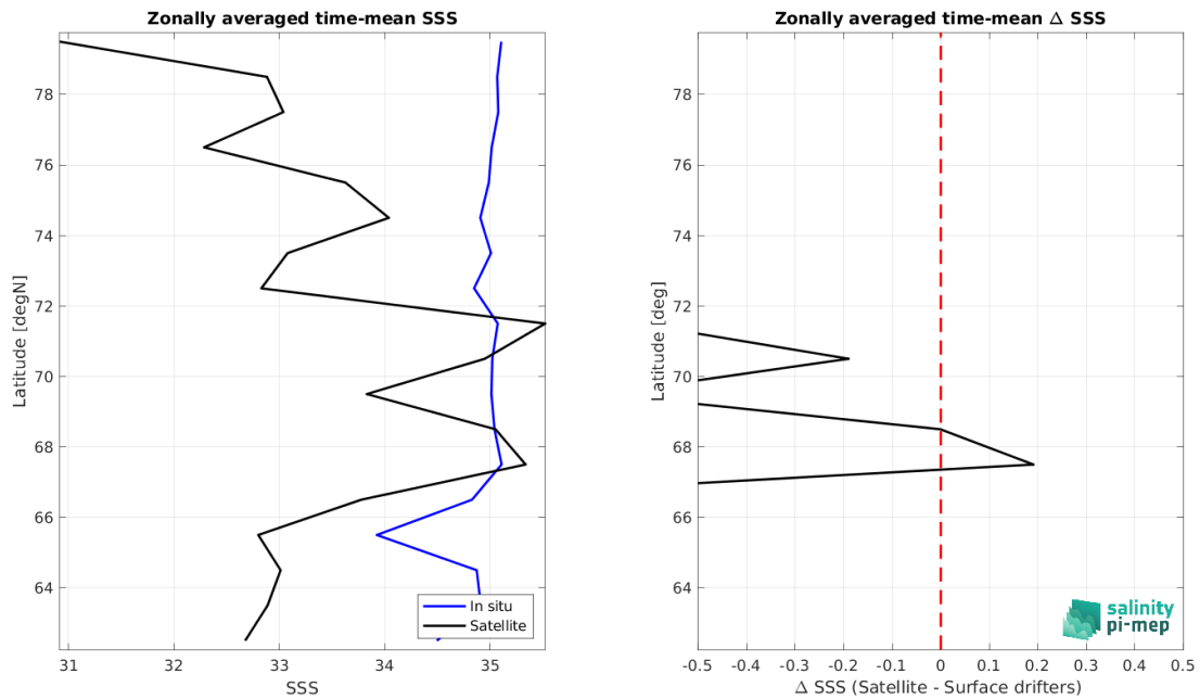
Figure 7: Left panel: Zonal mean SSS from SMOS SSS L3 Arctic v1.1 - 7-Day running mean (CATDS-CEC-LOCEAN) satellite product (black) and from Surface drifters (blue). Right panel: Zonal mean of \Delta SSS (Satellite - Surface drifters) for all the collected Pi-MEP match-up pairs estimated over the full satellite product period.
