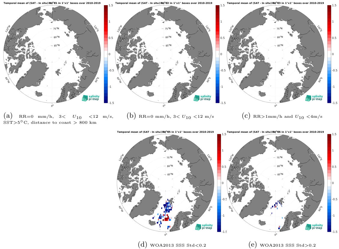
Figure 11: Temporal mean gridded over spatial boxes of size 1^{\circ}\times 1^{\circ} of \Delta\text{SSS} (SMOS SSS L3 Arctic v1.1 - 7-Day running mean (CATDS-CEC-LOCEAN) - Surface drifters) for 5 different subdatasets corresponding to:RR=0 mm/h, 3 < U_{10} < 12 m/s, SST > 5^{\circ}\text{C} , distance to coast > 800 km (a), RR=0 mm/h, 3 < U_{10} < 12 m/s (b), RR > 1 mm/h and U_{10} < 4 m/s (c), WOA2013 SSS Std < 0.2 (d), WOA2013 SSS Std > 0.2 (e).
