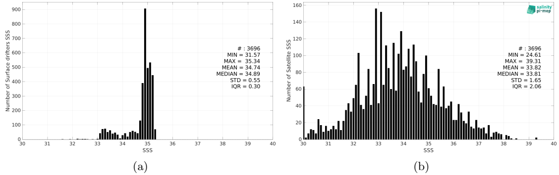
Figure 2: Histograms of SSS from Surface drifters (a) and SMOS SSS L3 Arctic v1.1 - 7-Day running mean (CATDS-CEC-LOCEAN) (b) considering all match-up pairs per bins of 0.1 over the Arctic Ocean Pi-MEP region and for the full satellite product period.
