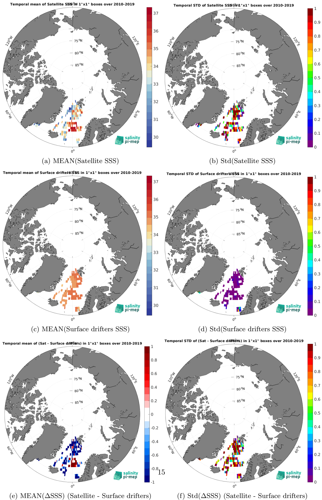
Figure 5: Temporal mean (left) and Std (right) of SSS from SMOS SSS L3 Arctic v1.1 - 7-Day running mean (CATDS-CEC-LOCEAN) (top), Surface drifters (middle), and of \Delta SSS (Satellite - Surface drifters). Only match-up pairs are used to generate these maps.
