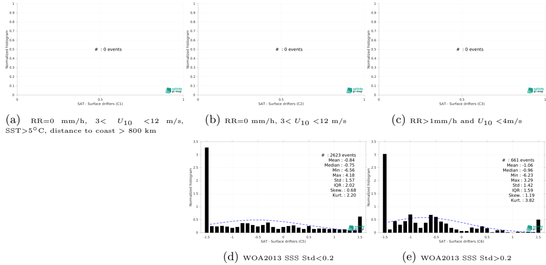
Figure 12: Normalized histogram of \Delta SSS (SMOS SSS L3 Arctic v1.1 - 7-Day running mean (CATDS-CEC-LOCEAN) - Surface drifters) for 5 different subdatasets corresponding to: RR=0 mm/h, 3 < U_{10} < 12 m/s, SST > 5°C, distance to coast > 800 km (a), RR=0 mm/h, 3 < U_{10} < 12 m/s (b), RR > 1mm/h and U_{10} < 4 m/s (c), WOA2013 SSS Std < 0.2 (d), WOA2013 SSS Std > 0.2 (e).
