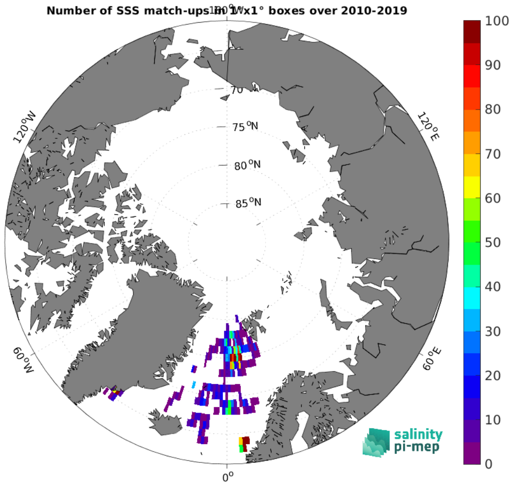
Figure 3: Number of SSS match-ups between Surface drifters SSS and the SMOS SSS L3 Arctic v1.1 - 7-Day running mean (CATDS-CEC-LOCEAN) SSS product for the Arctic Ocean Pi-MEP region over 1^\circ \times 1^\circ boxes and for the full satellite product period.
