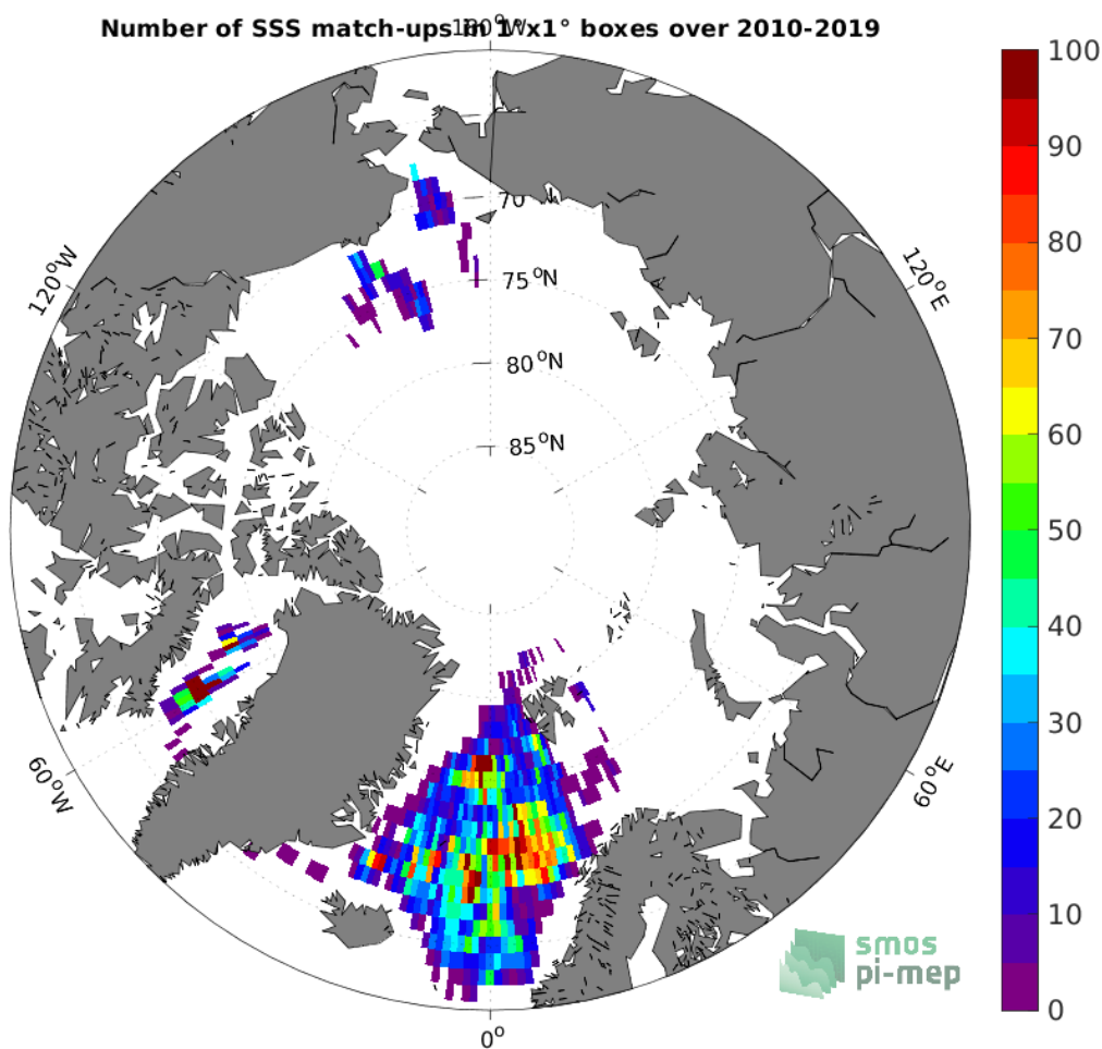
Figure 4: Number of SSS match-ups between Argo SSS and the SMOS SSS L3 Arctic v1.1 - 7-Day running mean (CATDS-CECOS-LOCEAN) SSS product for the Arctic Ocean Pi-MEP region over 1^\circ \times 1^\circ boxes and for the full satellite product period.
