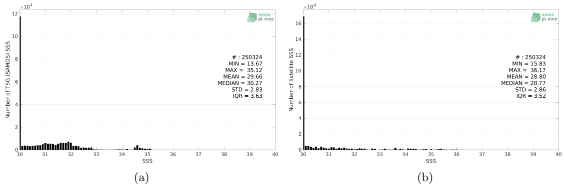
Figure 2: Histograms of SSS from TSG (SAMOS) (a) and SMOS SSS L3 Arctic v1.1 - Monthly (CATDS-CECOS-LOCEAN) (b) considering all match-up pairs per bins of 0.1 over the Arctic Ocean Pi-MEP region and for the full satellite product period.
