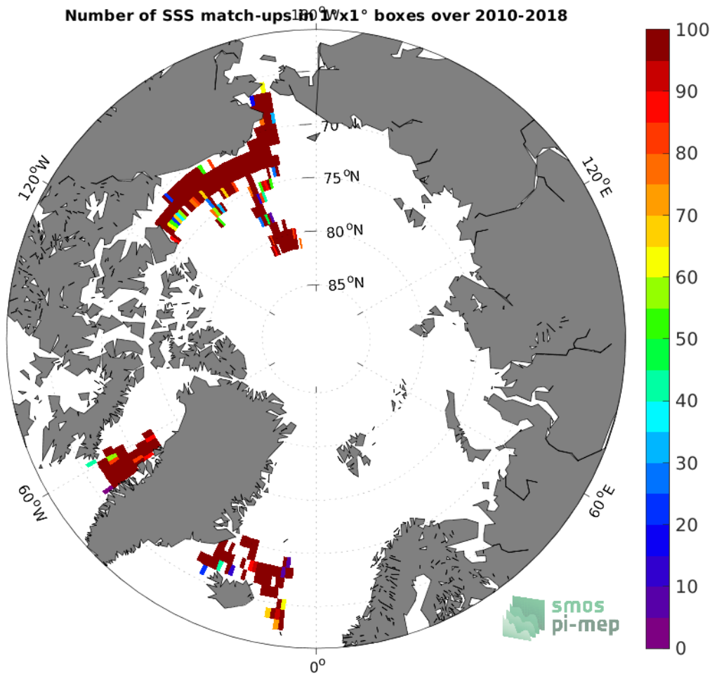
Figure 4: Number of SSS match-ups between TSG (SAMOS) SSS and the SMOS SSS L3 Arctic v1.1 - Monthly (CATDS-CECOS-LOCEAN) SSS product for the Arctic Ocean Pi-MEP region over 1^\circ \times 1^\circ boxes and for the full satellite product period.
