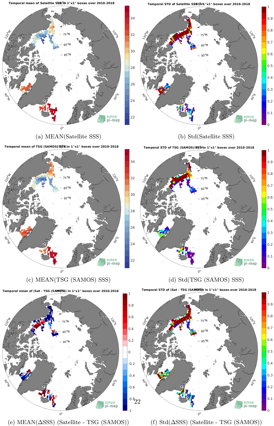
Figure 6: Temporal mean (left) and Std (right) of SSS from SMOS SSS L3 Arctic v1.1 - Monthly (CATDS-CECOS-LOCEAN) (top), TSG (SAMOS) (middle), and of \Delta SSS (Satellite - TSG (SAMOS)). Only match-up pairs are used to generate these maps.
