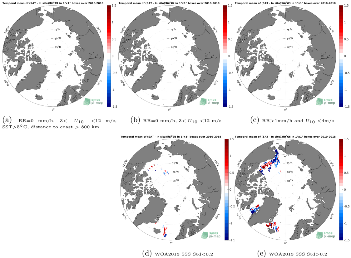
Figure 12: Temporal mean gridded over spatial boxes of size 1^{\circ}\times 1^{\circ} of \Delta\text{SSS} (SMOS SSS L3 Arctic v1.1 - Monthly (CATDS-CECOS-LOCEAN) - TSG (SAMOS)) for 5 different subdatasets corresponding to:RR=0 mm/h, 3 < U_{10} < 12 m/s, SST > 5^{\circ}\text{C} , distance to coast > 800 km (a), RR=0 mm/h, 3 < U_{10} < 12 m/s (b), RR > 1 mm/h and U_{10} < 4 m/s (c), WOA2013 SSS Std < 0.2 (d), WOA2013 SSS Std > 0.2 (e).
