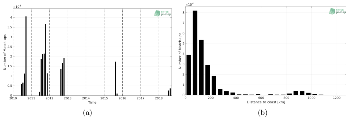
Figure 1: Number of match-ups between TSG (SAMOS) and SMOS SSS L3 Arctic v1.1 - Monthly (CATDS-CECOS-LOCEAN) SSS as a function of time (a) and as function of the distance to coast (b) over the Arctic Ocean Pi-MEP region and for the full satellite product period.
