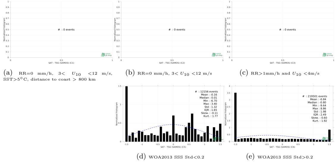
Figure 13: Normalized histogram of \Delta SSS (SMOS SSS L3 Arctic v1.1 - Monthly (CATDS-CECOS-LOCEAN) - TSG (SAMOS)) for 5 different subdatasets corresponding to: RR=0 mm/h, 3 < U_{10} < 12 m/s, SST > 5°C, distance to coast > 800 km (a), RR=0 mm/h, 3 < U_{10} < 12 m/s (b), RR > 1mm/h and U_{10} < 4 m/s (c), WOA2013 SSS Std < 0.2 (d), WOA2013 SSS Std > 0.2 (e).
