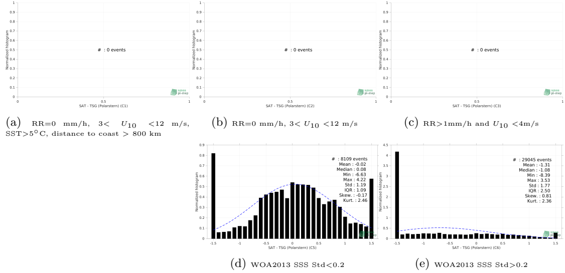
Figure 13: Normalized histogram of \Delta SSS (SMOS SSS L3 Arctic v1.1 - Monthly (CATDS-CECOS-LOCEAN) - TSG (Polarstern)) for 5 different subdatasets corresponding to: RR=0 mm/h, 3 < U_{10} < 12 m/s, SST > 5°C, distance to coast > 800 km (a), RR=0 mm/h, 3 < U_{10} < 12 m/s (b), RR > 1mm/h and U_{10} < 4 m/s (c), WOA2013 SSS Std < 0.2 (d), WOA2013 SSS Std > 0.2 (e).
