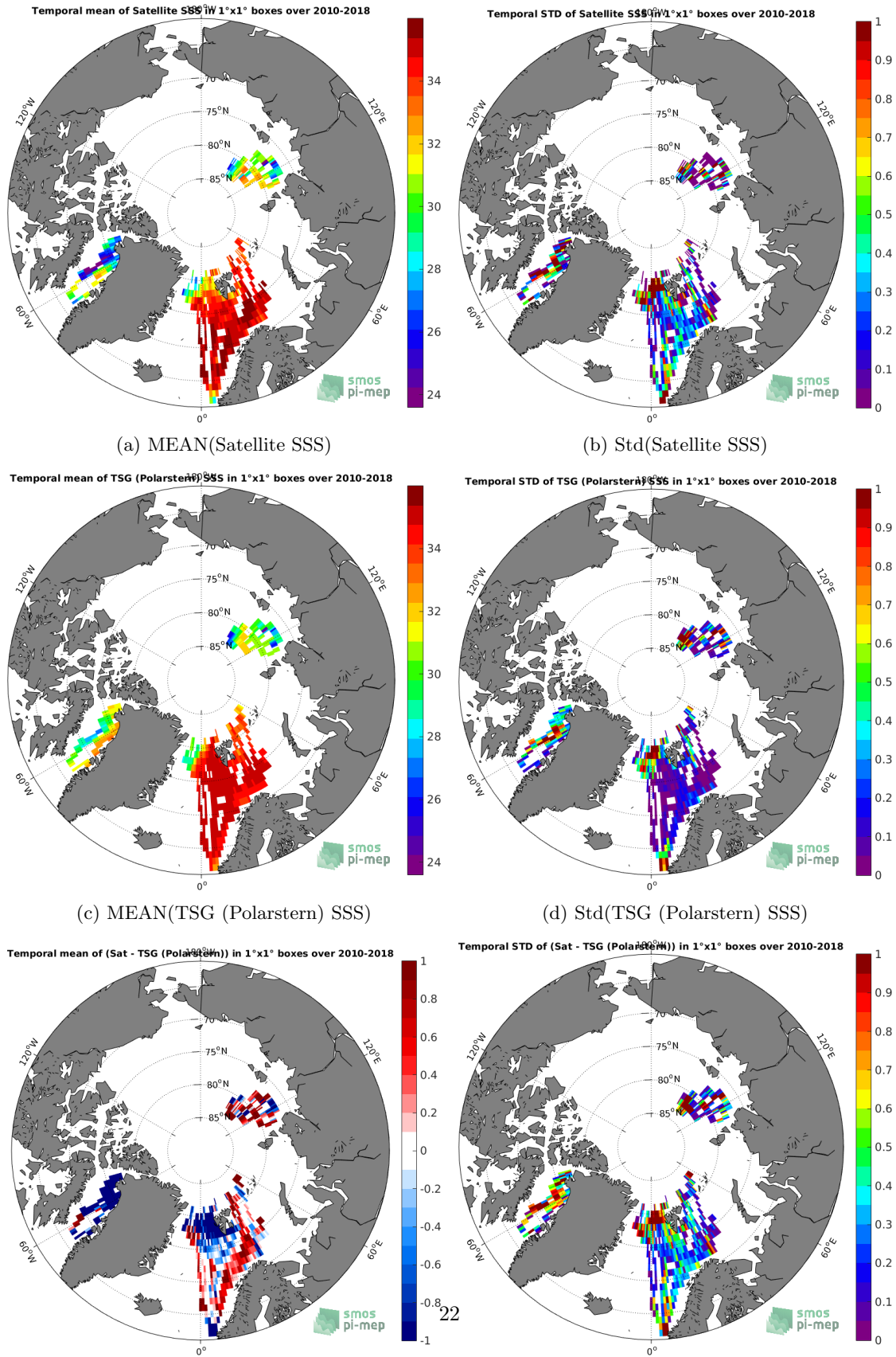
Figure 6: Temporal mean (left) and Std (right) of SSS from SMOS SSS L3 ARCTIC v1.1 - Monthly (CATDS-CECOS-LOCEAN) (top), TSG (Polarstern) (middle), and of \Delta SSS (Satellite - TSG (Polarstern)). Only match-up pairs are used to generate these maps.
