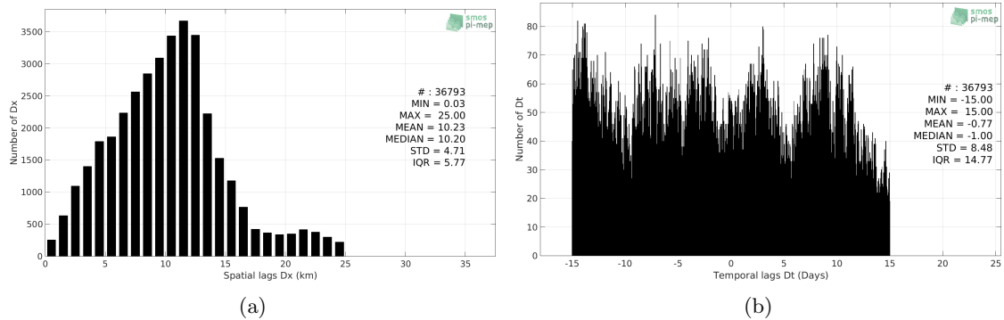
Figure 5: Histograms of the spatial (a) and temporal (b) lags between the time of the TSG (Polarstern) measurements and the date of the corresponding SMOS SSS L3 ARCTIC v1.1 - Monthly (CATDS-CECOS-LOCEAN) SSS product.
