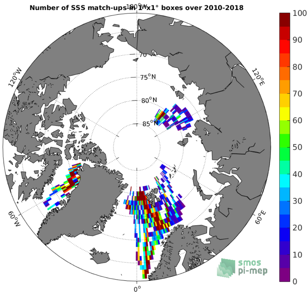
Figure 4: Number of SSS match-ups between TSG (Polarstern) SSS and the SMOS SSS L3 ARCTIC v1.1 - Monthly (CATDS-CECOS-LOCEAN) SSS product for the Arctic Ocean Pi-MEP region over 1°x1° boxes and for the full satellite product period.
