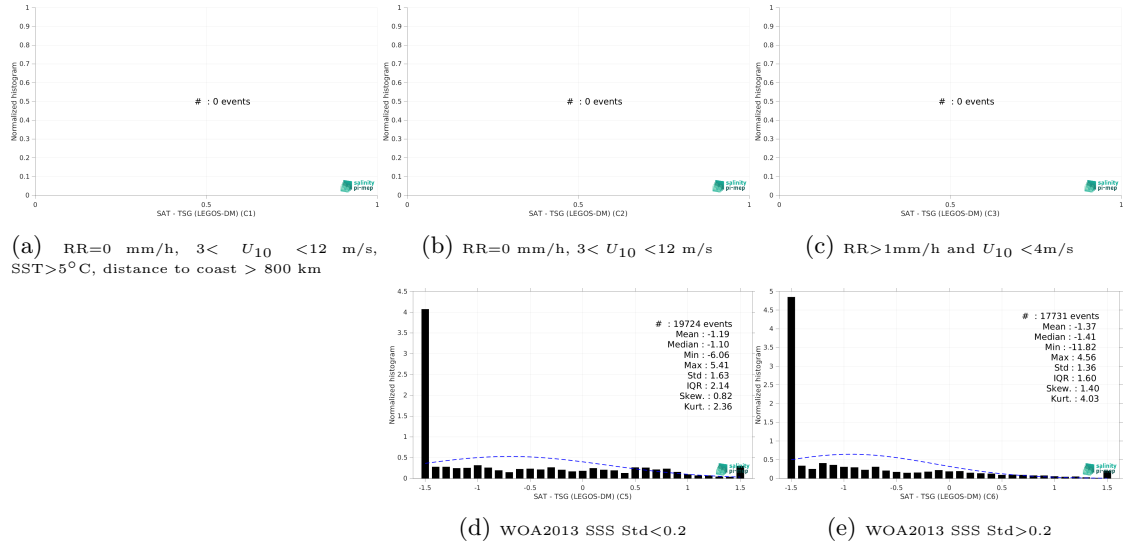
Figure 13: Normalized histogram of \Delta SSS (SMOS SSS L3 Arctic v1.1 - Monthly (CATDS-CECOS-LOCEAN) - TSG (LEGOS-DM)) for 5 different subdatasets corresponding to: RR=0 mm/h, 3 < U_{10} < 12 m/s, SST > 5°C, distance to coast > 800 km (a), RR=0 mm/h, 3 < U_{10} < 12 m/s (b), RR > 1mm/h and U_{10} < 4 m/s (c), WOA2013 SSS Std < 0.2 (d), WOA2013 SSS Std > 0.2 (e).
