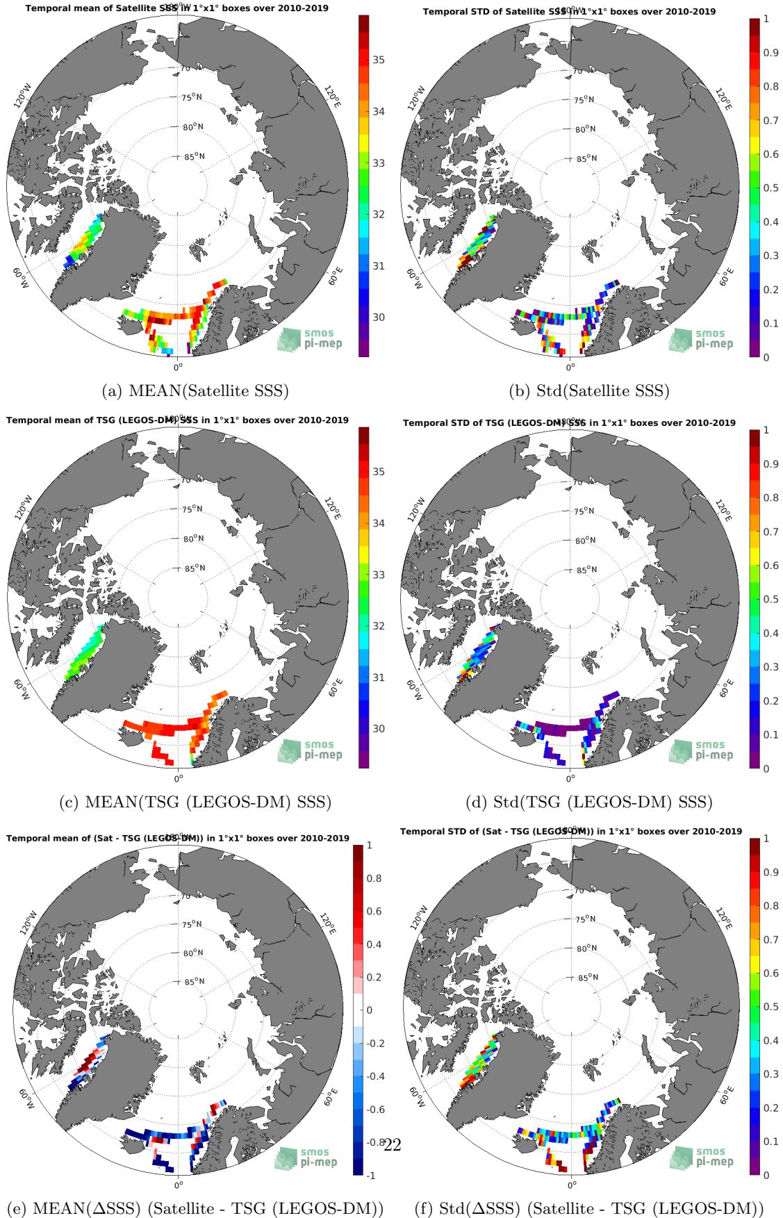
Figure 6: Temporal mean (left) and Std (right) of SSS from SMOS SSS L3 Arctic v1.1 - Monthly (CATDS-CECOS-LOCEAN) (top), TSG (LEGOS-DM) (middle), and of \Delta SSS (Satellite - TSG (LEGOS-DM)). Only match-up pairs are used to generate these maps.
