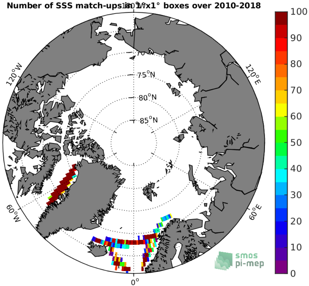
Figure 4: Number of SSS match-ups between TSG (LEGOS-DM) SSS and the SMOS SSS L3 Arctic v1.1 - Monthly (CATDS-CECOS-LOCEAN) SSS product for the Arctic Ocean Pi-MEP region over 1°x1° boxes and for the full satellite product period.
