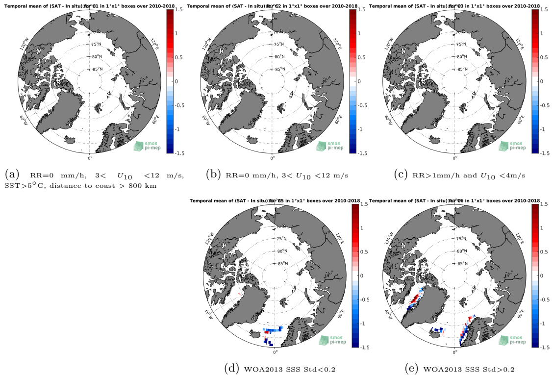
Figure 12: Temporal mean gridded over spatial boxes of size 1^{\circ}\times 1^{\circ} of \Delta\text{SSS} (SMOS SSS L3 Arctic v1.1 - Monthly (CATDS-CECOS-LOCEAN) - TSG (LEGOS-DM)) for 5 different subdatasets corresponding to:RR=0 mm/h, 3 < U_{10} < 12 m/s, SST >5^{\circ}\text{C} , distance to coast > 800 km (a), RR=0 mm/h, 3 < U_{10} < 12 m/s (b), RR >1 mm/h and U_{10} < 4 m/s (c), WOA2013 SSS Std <0.2 (d), WOA2013 SSS Std >0.2 (e).
