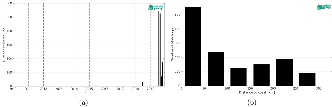
Figure 1: Number of match-ups between TSG (Lauge-Koch) and SMOS SSS L3 Arctic v1.1 - Monthly (CATDS-CECOS-LOCEAN) SSS as a function of time (a) and as function of the distance to coast (b) over the Arctic Ocean Pi-MEP region and for the full satellite product period.
