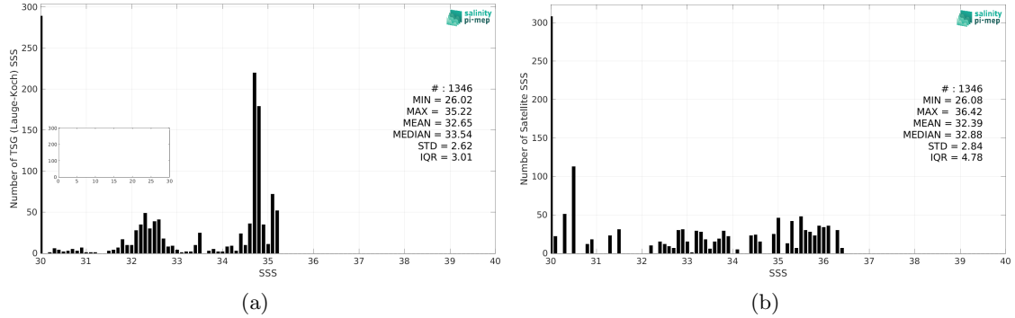
Figure 2: Histograms of SSS from TSG (Lauge-Koch) (a) and SMOS SSS L3 Arctic v1.1 - Monthly (CATDS-CECOS-LOCEAN) (b) considering all match-up pairs per bins of 0.1 over the Arctic Ocean Pi-MEP region and for the full satellite product period.
