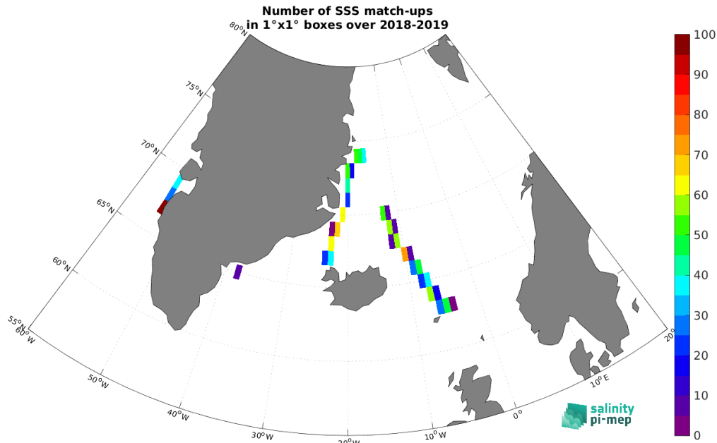
Figure 4: Number of SSS match-ups between TSG (Lauge-Koch) SSS and the SMOS SSS L3 Arctic v1.1 - Monthly (CATDS-CECOS-LOCEAN) SSS product for the Arctic Ocean Pi-MEP region over 1^\circ \times 1^\circ boxes and for the full satellite product period.
