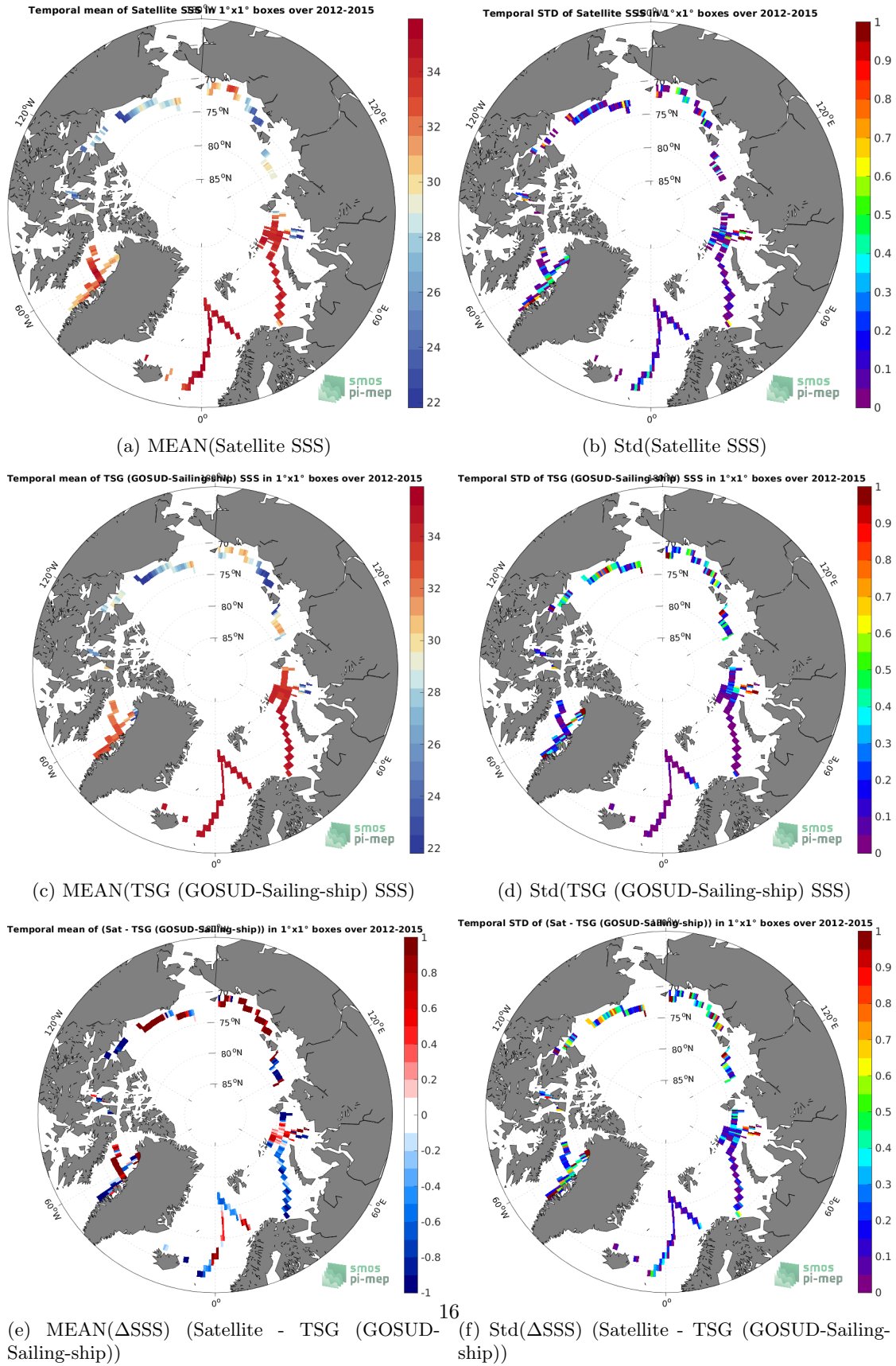
Figure 6: Temporal mean (left) and Std (right) of SSS from SMOS SSS L3 Arctic v1.1 - Monthly (CATDS-CECOS-LOCEAN) (top), TSG (GOSUD-Sailing-ship) (middle), and of \Delta SSS (Satellite - TSG (GOSUD-Sailing-ship)). Only match-up pairs are used to generate these maps.
