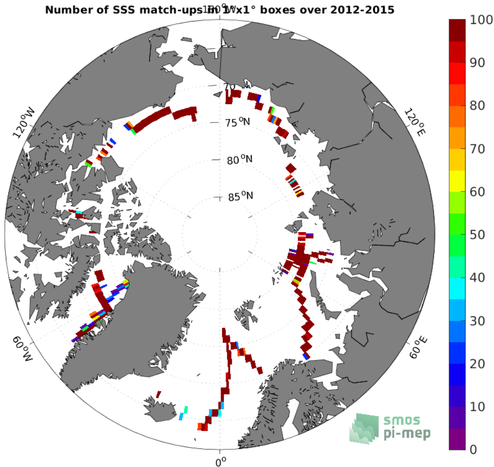
Figure 4: Number of SSS match-ups between TSG (GOSUD-Sailing-ship) SSS and the SMOS SSS L3 Arctic v1.1 - Monthly (CATDS-CECOS-LOCEAN) SSS product for the Arctic Ocean Pi-MEP region over 1^\circ \times 1^\circ boxes and for the full satellite product period.
