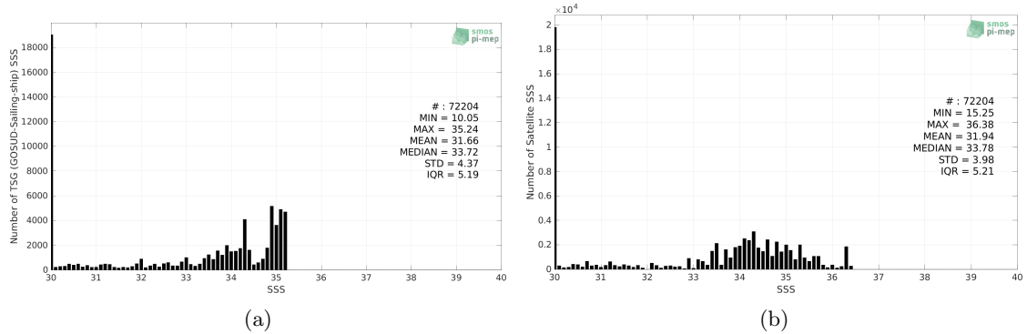
Figure 2: Histograms of SSS from TSG (GOSUD-Sailing-ship) (a) and SMOS SSS L3 Arctic v1.1 - Monthly (CATDS-CECOS-LOCEAN) (b) considering all match-up pairs per bins of 0.1 over the Arctic Ocean Pi-MEP region and for the full satellite product period.
