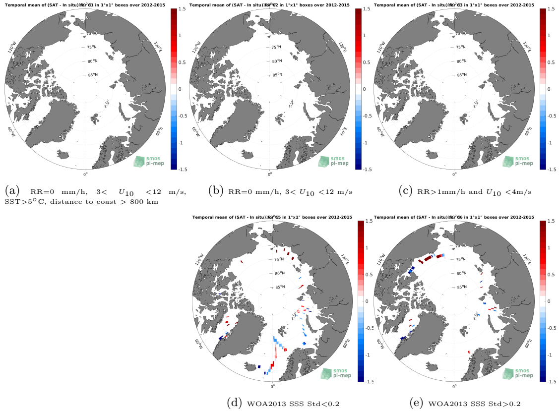
Figure 12: Temporal mean gridded over spatial boxes of size 1^\circ \times 1^\circ of \Delta SSS (SMOS SSS L3 Arctic v1.1 - Monthly (CATDS-CECOS-LOCEAN) - TSG (GOSUD-Sailing-ship)) for 5 different subdatasets corresponding to: RR=0 mm/h, 3 < U_{10} < 12 m/s, SST > 5°C, distance to coast > 800 km (a), RR=0 mm/h, 3 < U_{10} < 12 m/s (b), RR > 1mm/h and U_{10} < 4 m/s (c), WOA2013 SSS Std < 0.2 (d), WOA2013 SSS Std > 0.2 (e).
