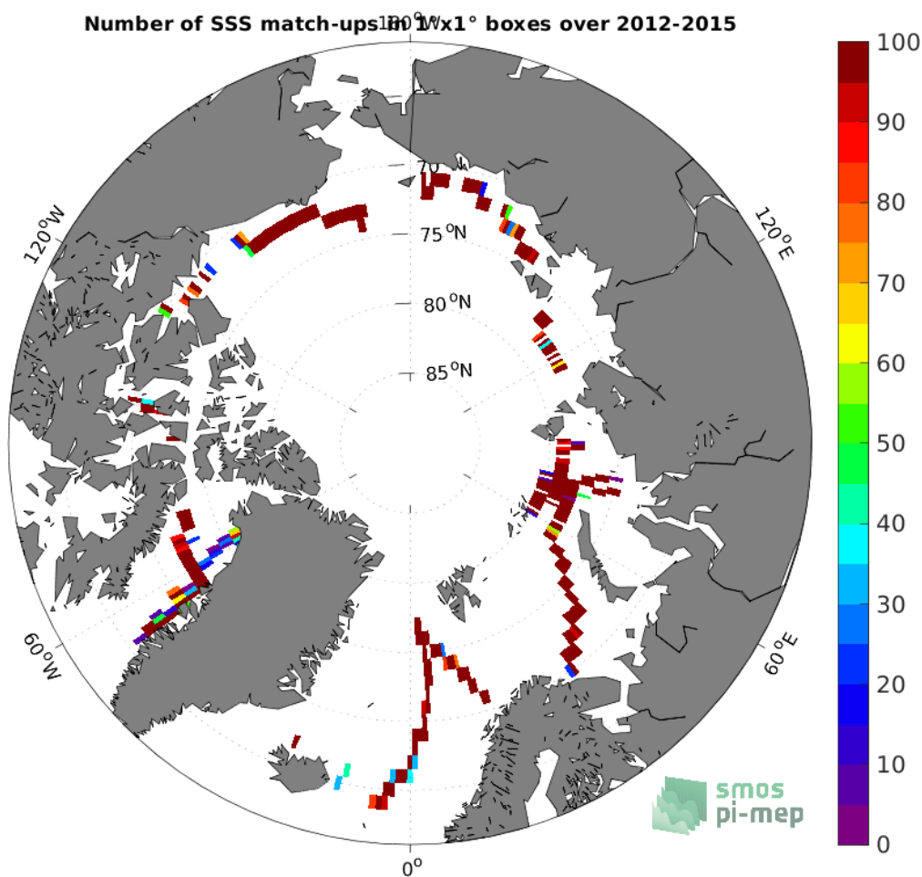
Figure 4: Number of SSS match-ups between TSG (GOSUD-Sailing-ship) SSS and the SMOS SSS L3 Arctic v1.1 - Monthly (CATDS-CECOS-LOCEAN) SSS product for the Arctic Ocean Pi-MEP region over 1^{\circ} \times 1^{\circ} boxes and for the full satellite product period.
