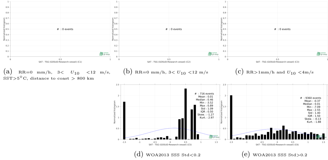
Figure 13: Normalized histogram of \Delta\text{SSS} (SMOS SSS L3 Arctic v1.1 - Monthly (CATDS-CECOS-LOCEAN) - TSG (GOSUD-Research-vessel)) for 5 different subdatasets corresponding to: RR=0 mm/h, 3 < U_{10} < 12 m/s, SST > 5^\circ\text{C} , distance to coast > 800 km (a), RR=0 mm/h, 3 < U_{10} < 12 m/s (b), RR > 1\text{mm/h} and U_{10} < 4\text{m/s} (c), WOA2013 SSS Std < 0.2 (d), WOA2013 SSS Std > 0.2 (e).
