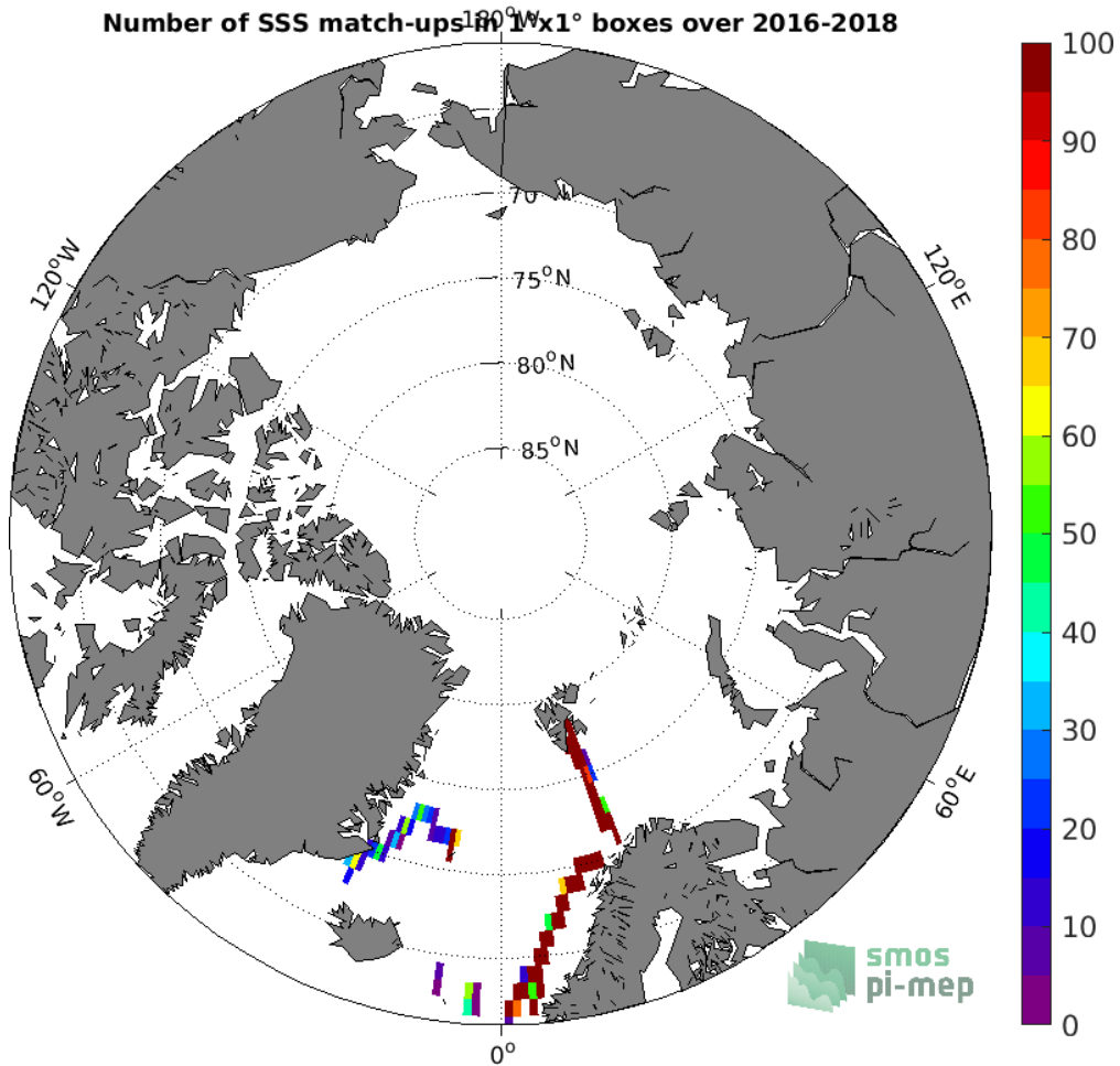
Figure 4: Number of SSS match-ups between TSG (GOSUD-Research-vessel) SSS and the SMOS SSS L3 Arctic v1.1 - Monthly (CATDS-CECOS-LOCEAN) SSS product for the Arctic Ocean Pi-MEP region over 1^\circ \times 1^\circ boxes and for the full satellite product period.
