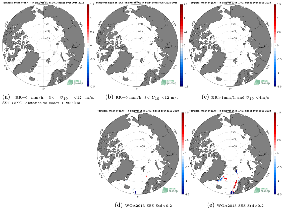
Figure 12: Temporal mean gridded over spatial boxes of size 1^\circ \times 1^\circ of \Delta SSS (SMOS SSS L3 Arctic v1.1 - Monthly (CATDS-CECOS-LOCEAN) - TSG (GOSUD-Research-vessel)) for 5 different subdatasets corresponding to:RR=0 mm/h, 3 < U_{10} < 12 m/s, SST>5°C, distance to coast > 800 km (a), RR=0 mm/h, 3 < U_{10} < 12 m/s (b), RR>1mm/h and U_{10} < 4 m/s (c), WOA2013 SSS Std<0.2 (d), WOA2013 SSS Std>0.2 (e).
