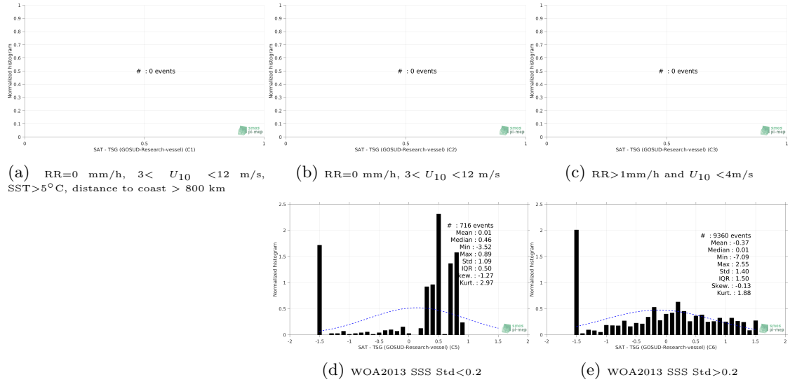
Figure 13: Normalized histogram of \Delta SSS (SMOS SSS L3 ARCTIC v1.1 - Monthly (CATDS-CECOS-LOCEAN) - TSG (GOSUD-Research-vessel)) for 5 different subdatasets corresponding to: RR=0 mm/h, 3 < U_{10} < 12 m/s, SST > 5°C, distance to coast > 800 km (a), RR=0 mm/h, 3 < U_{10} < 12 m/s (b), RR > 1mm/h and U_{10} < 4 m/s (c), WOA2013 SSS Std < 0.2 (d), WOA2013 SSS Std > 0.2 (e).
