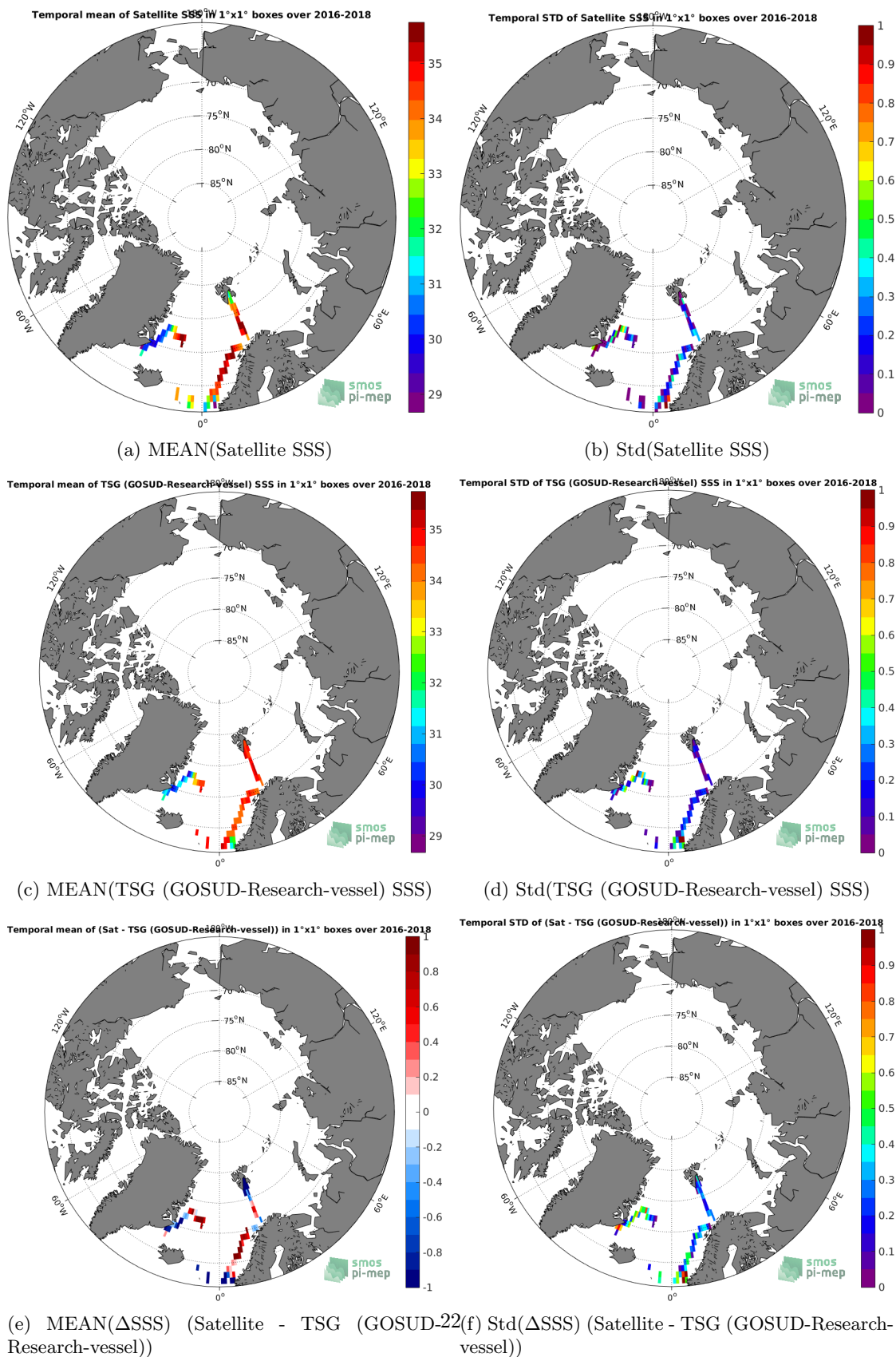
Figure 6: Temporal mean (left) and Std (right) of SSS from SMOS SSS L3 ARCTIC v1.1 - Monthly (CATDS-CECOS-LOCEAN) (top), TSG (GOSUD-Research-vessel) (middle), and of \Delta SSS (Satellite - TSG (GOSUD-Research-vessel)). Only match-up pairs are used to generate these maps.
