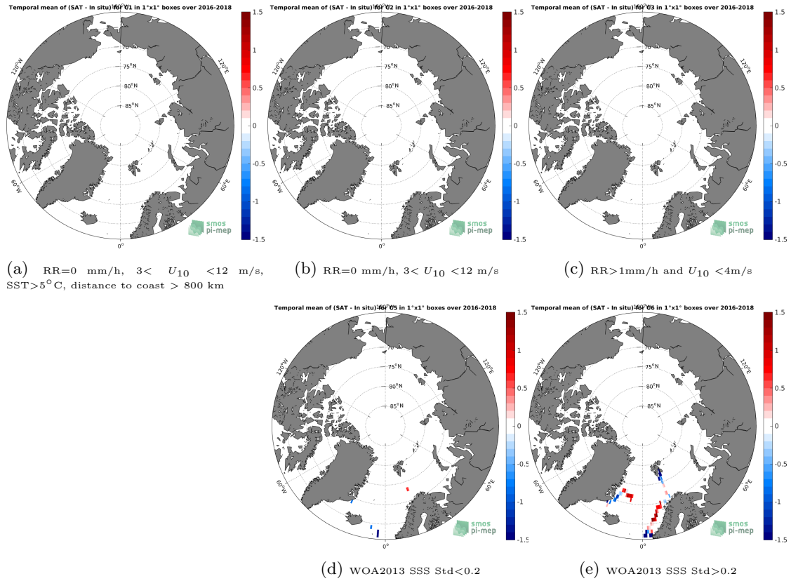
Figure 12: Temporal mean gridded over spatial boxes of size 1°x1° of \Delta SSS (SMOS SSS L3 ARCTIC v1.1 - Monthly (CATDS-CECOS-LOCEAN) - TSG (GOSUD-Research-vessel)) for 5 different subdatasets corresponding to:RR=0 mm/h, 3 < U_{10} < 12 m/s, SST>5°C, distance to coast > 800 km (a), RR=0 mm/h, 3 < U_{10} < 12 m/s (b), RR>1mm/h and U_{10} < 4 m/s (c), WOA2013 SSS Std<0.2 (d), WOA2013 SSS Std>0.2 (e).
