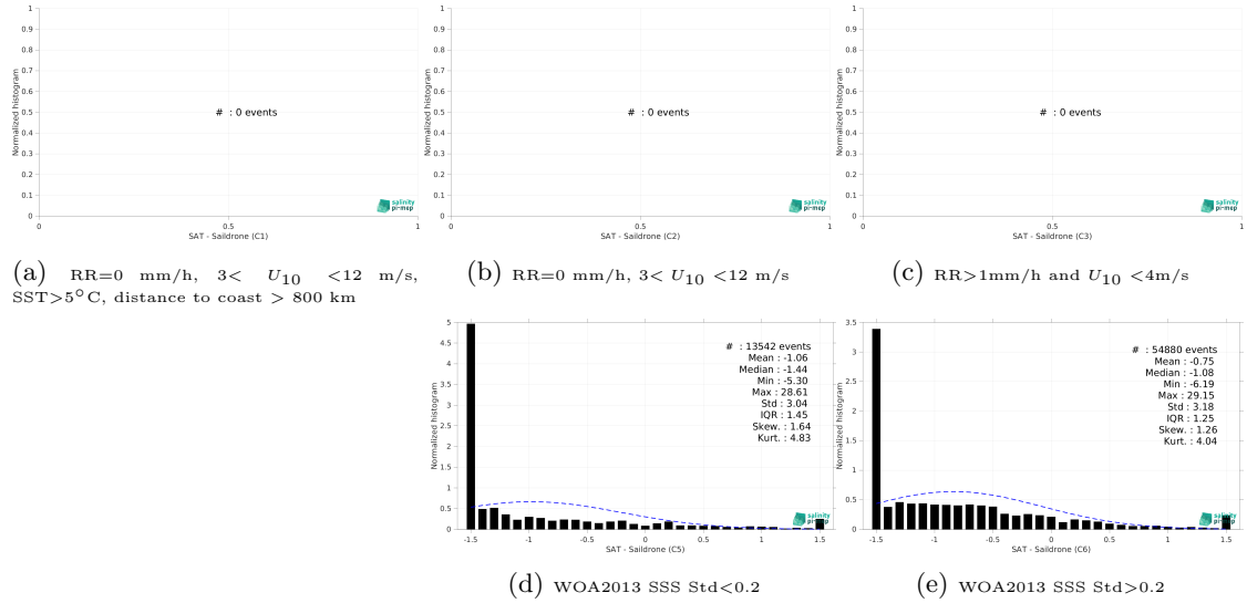
Figure 13: Normalized histogram of \Delta SSS (SMOS SSS L3 Arctic v1.1 - Monthly (CATDS-CECOS-LOCEAN) - Sairdrone) for 5 different subdatasets corresponding to: RR=0 mm/h, 3 < U_{10} < 12 m/s, SST > 5°C, distance to coast > 800 km (a), RR=0 mm/h, 3 < U_{10} < 12 m/s (b), RR > 1mm/h and U_{10} < 4 m/s (c), WOA2013 SSS Std < 0.2 (d), WOA2013 SSS Std > 0.2 (e).
