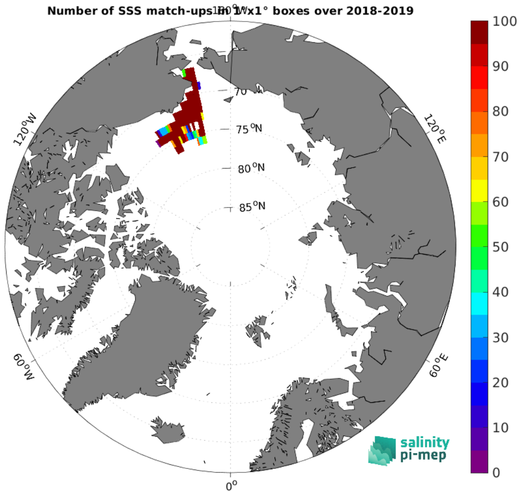
Figure 4: Number of SSS match-ups between Saildrone SSS and the SMOS SSS L3 Arctic v1.1 - Monthly (CATDS-CECOS-LOCEAN) SSS product for the Arctic Ocean Pi-MEP region over 1^{\circ} \times 1^{\circ} boxes and for the full satellite product period.
