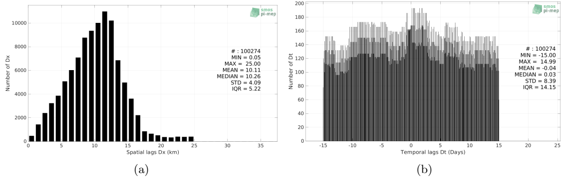
Figure 5: Histograms of the spatial (a) and temporal (b) lags between the location/time of the Saildrone measurement and the date of the corresponding SMOS SSS L3 Arctic v1.1 - Monthly (CATDS-CECOS-LOCEAN) SSS pixel.
