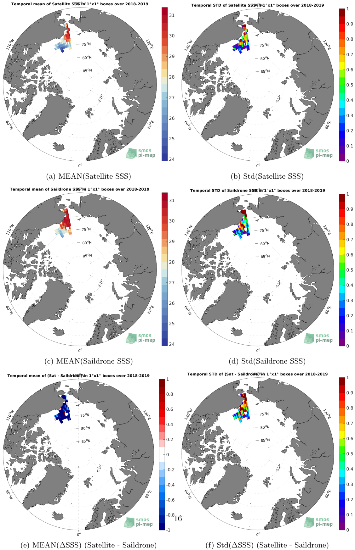
Figure 6: Temporal mean (left) and Std (right) of SSS from SMOS SSS L3 Arctic v1.1 - Monthly (CATDS-CECOS-LOCEAN) (top), Saildrone (middle), and of \Delta SSS (Satellite - Saildrone). Only match-up pairs are used to generate these maps.
