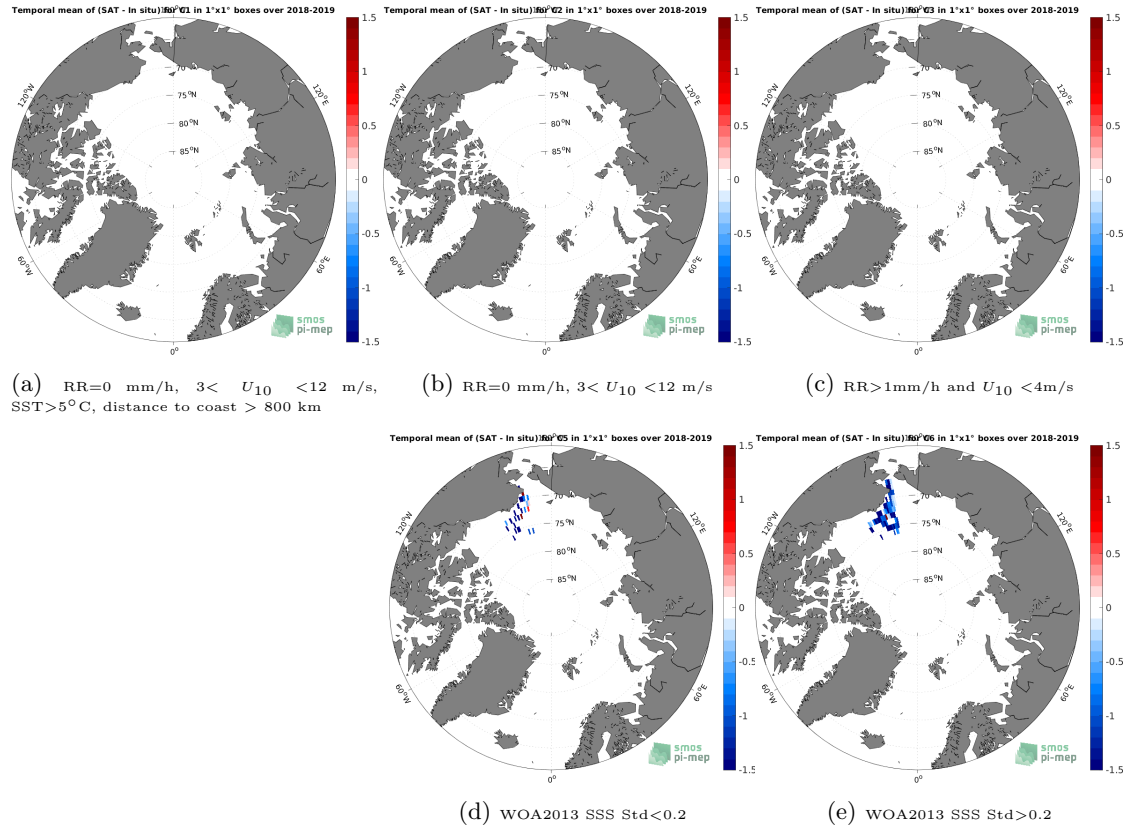
Figure 12: Temporal mean gridded over spatial boxes of size 1^{\circ}\times 1^{\circ} of \Delta\text{SSS} (SMOS SSS L3 Arctic v1.1 - Monthly (CATDS-CECOS-LOCEAN) - Saildrone) for 5 different subdatasets corresponding to:RR=0 mm/h, 3 < U_{10} < 12 m/s, SST >5^{\circ}\text{C} , distance to coast > 800 km (a), RR=0 mm/h, 3 < U_{10} < 12 m/s (b), RR >1 mm/h and U_{10} < 4 m/s (c), WOA2013 SSS Std <0.2 (d), WOA2013 SSS Std >0.2 (e).
