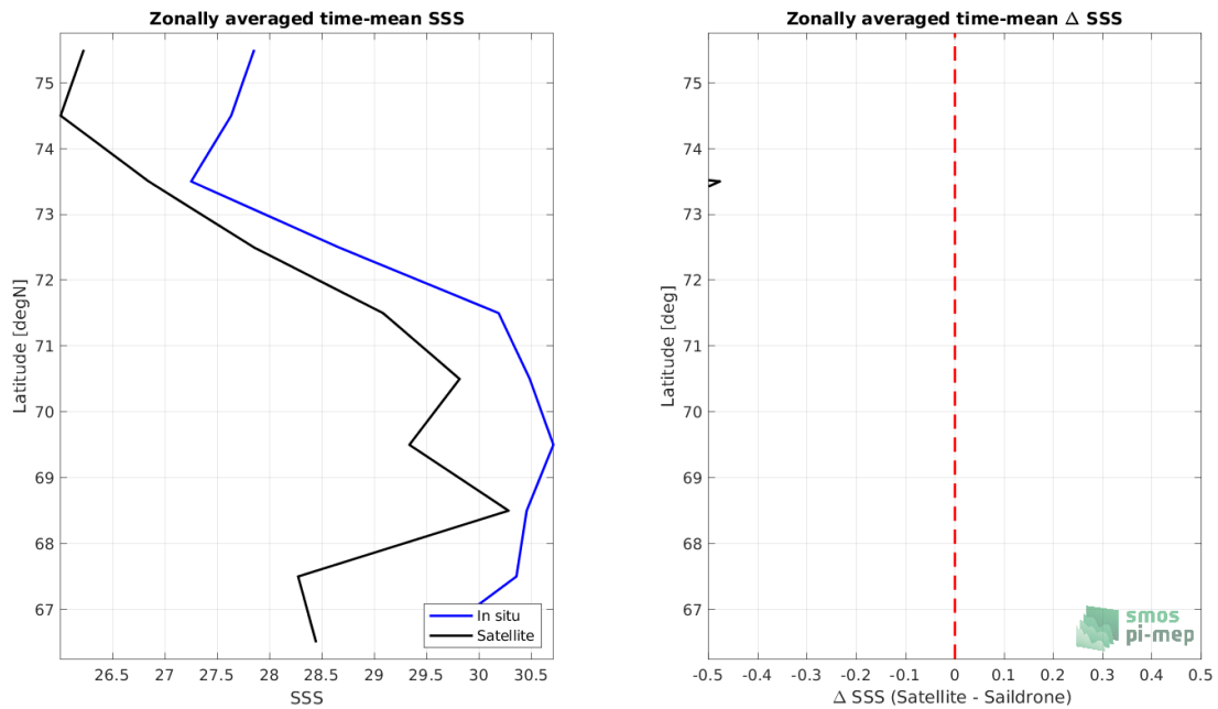
Figure 8: Left panel: Zonal mean SSS from SMOS SSS L3 Arctic v1.1 - Monthly (CATDS-CECOS-LOCEAN) satellite product (black) and from Sairdron (blue). Right panel: Zonal mean of \Delta SSS (Satellite - Sairdron) for all the collected Pi-MEP match-up pairs estimated over the full satellite product period.
