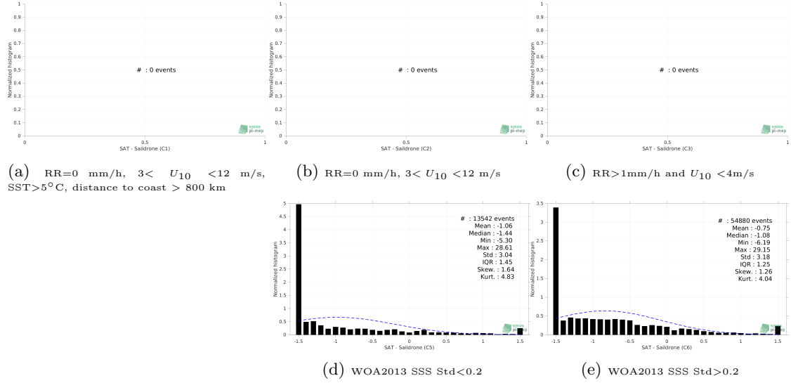
Figure 13: Normalized histogram of \Delta\text{SSS} (SMOS SSS L3 Arctic v1.1 - Monthly (CATDS-CECOS-LOCEAN) - Sairdrone) for 5 different subdatasets corresponding to: RR=0 mm/h, 3 < U_{10} < 12 m/s, SST > 5^\circ\text{C} , distance to coast > 800 km (a), RR=0 mm/h, 3 < U_{10} < 12 m/s (b), RR > 1\text{mm/h} and U_{10} < 4\text{m/s} (c), WOA2013 SSS Std < 0.2 (d), WOA2013 SSS Std > 0.2 (e).
