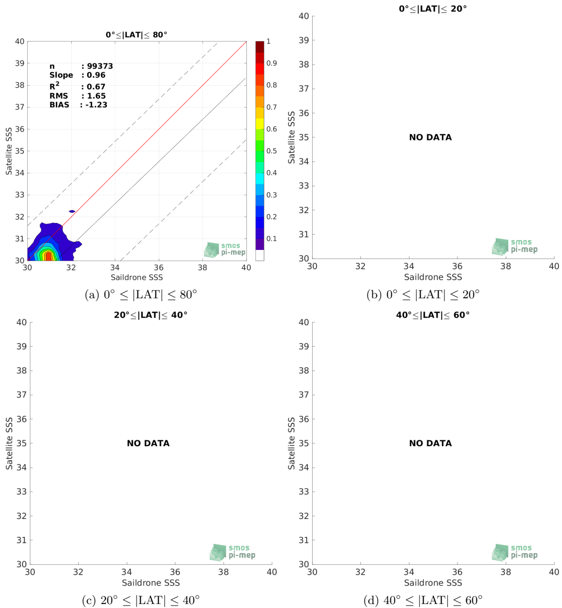
Figure 9: Contour maps of the concentration of SMOS SSS L3 Arctic v1.1 - Monthly (CATDS-CECOS-LOCEAN) SSS (y-axis) versus Saildrone SSS (x-axis) at match-up pairs for different latitude bands. For each plot, the red line shows x=y . The black thin and dashed lines indicate a linear fit through the data cloud and the \pm 95\% confidence levels, respectively. The number match-up pairs n , the slope and R^2 coefficient of the linear fit, the root mean square (RMS) and the mean bias between satellite and in situ data are indicated for each latitude band in each plots.
