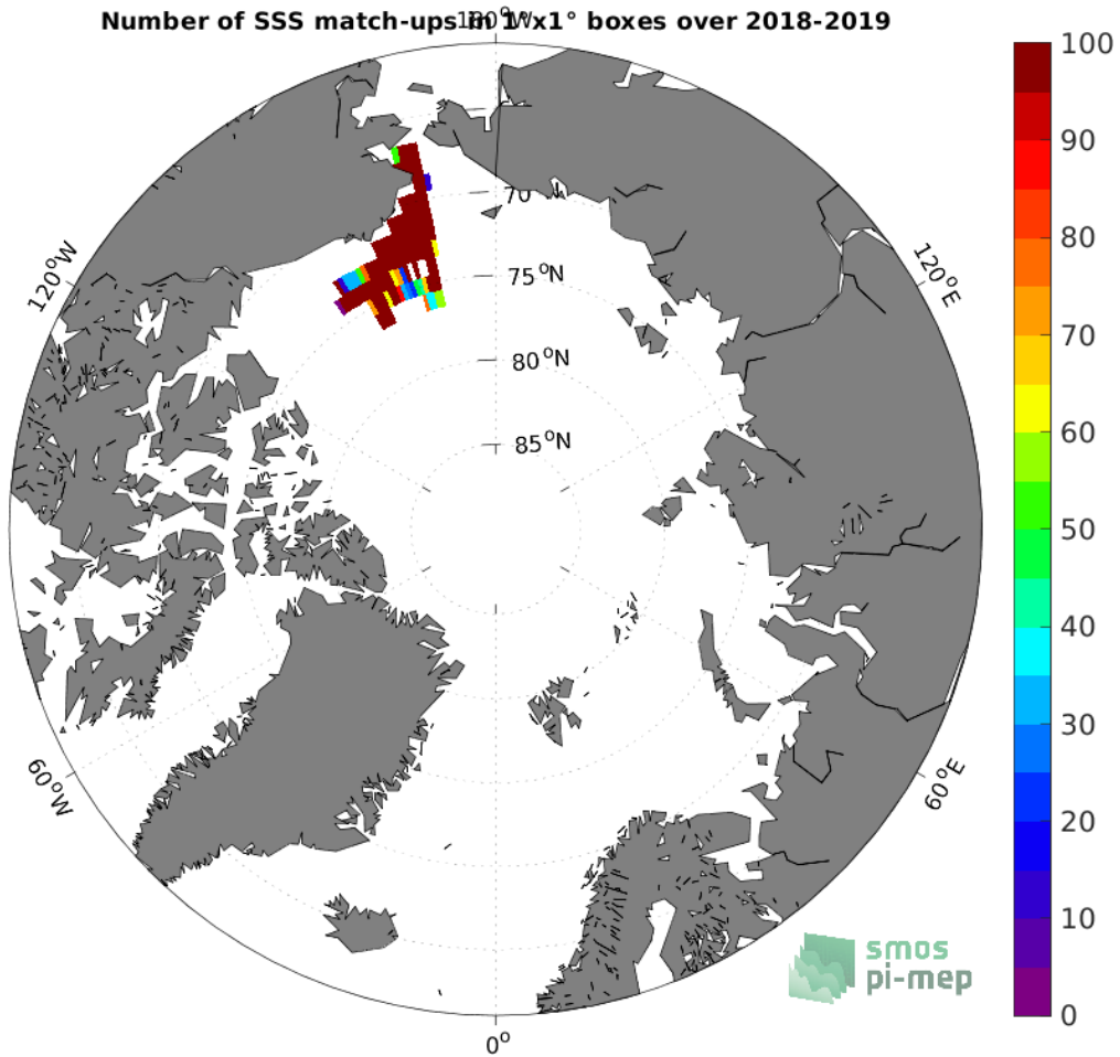
Figure 4: Number of SSS match-ups between Sailldrone SSS and the SMOS SSS L3 Arctic v1.1 - Monthly (CATDS-CECOS-LOCEAN) SSS product for the Arctic Ocean Pi-MEP region over 1^\circ \times 1^\circ boxes and for the full satellite product period.
