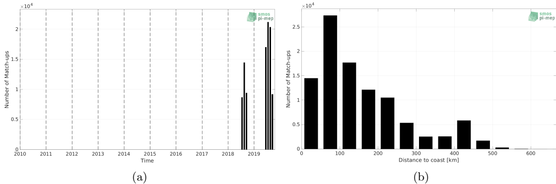
Figure 1: Number of match-ups between Saildrone and SMOS SSS L3 Arctic v1.1 - Monthly (CATDS-CECOS-LOCEAN) SSS as a function of time (a) and as function of the distance to coast (b) over the Arctic Ocean Pi-MEP region and for the full satellite product period.
