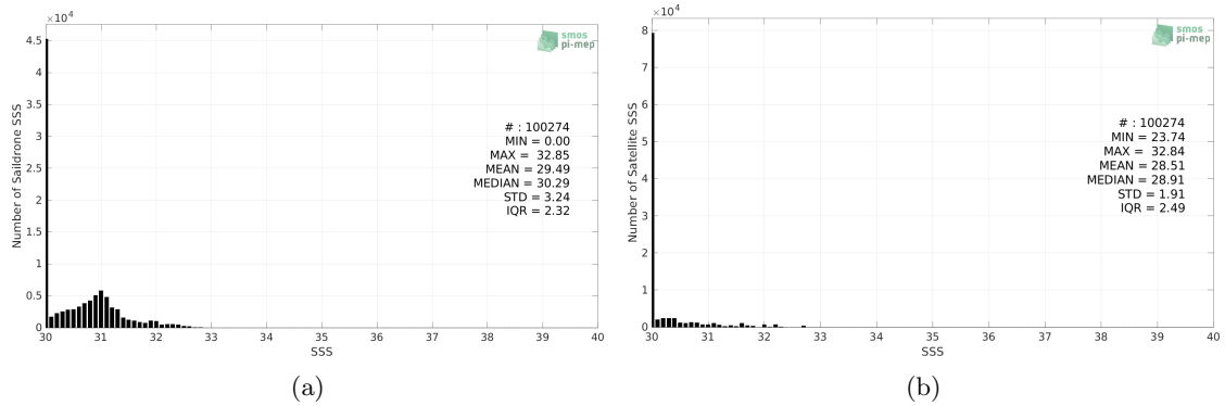
Figure 2: Histograms of SSS from Saildrone (a) and SMOS SSS L3 Arctic v1.1 - Monthly (CATDS-CECOS-LOCEAN) (b) considering all match-up pairs per bins of 0.1 over the Arctic Ocean Pi-MEP region and for the full satellite product period.
