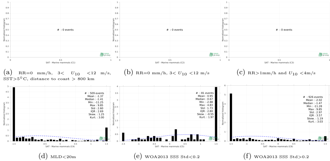
Figure 13: Normalized histogram of \Delta\text{SSS} (SMOS SSS L3 Arctic v1.1 - Monthly (CATDS-CECOS-LOCEAN) - Marine mammals) for 6 different subdatasets corresponding to: RR=0 mm/h, 3 < U_{10} < 12 m/s, SST > 5^\circ\text{C} , distance to coast > 800 km (a), RR=0 mm/h, 3 < U_{10} < 12 m/s (b), RR > 1\text{mm/h} and U_{10} < 4\text{m/s} (c), MLD < 20\text{m} (d), WOA2013 SSS Std < 0.2 (e), WOA2013 SSS Std > 0.2 (f).
