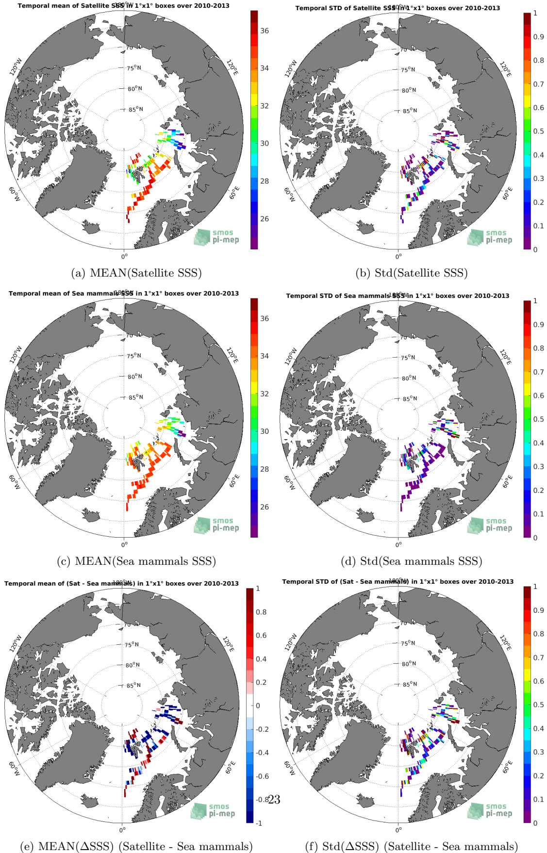
Figure 6: Temporal mean (left) and Std (right) of SSS from SMOS SSS L3 Arctic v1.1 - Monthly (CATDS-CECOS-LOCEAN) (top), Sea mammals (middle), and of \Delta SSS (Satellite - Sea mammals). Only match-up pairs are used to generate these maps.
