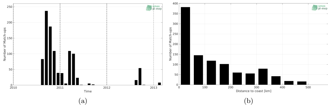
Figure 1: Number of match-ups between Sea mammals and SMOS SSS L3 Arctic v1.1 - Monthly (CATDS-CECOS-LOCEAN) SSS as a function of time (a) and as function of the distance to coast (b) over the Arctic Ocean Pi-MEP region and for the full satellite product period.
