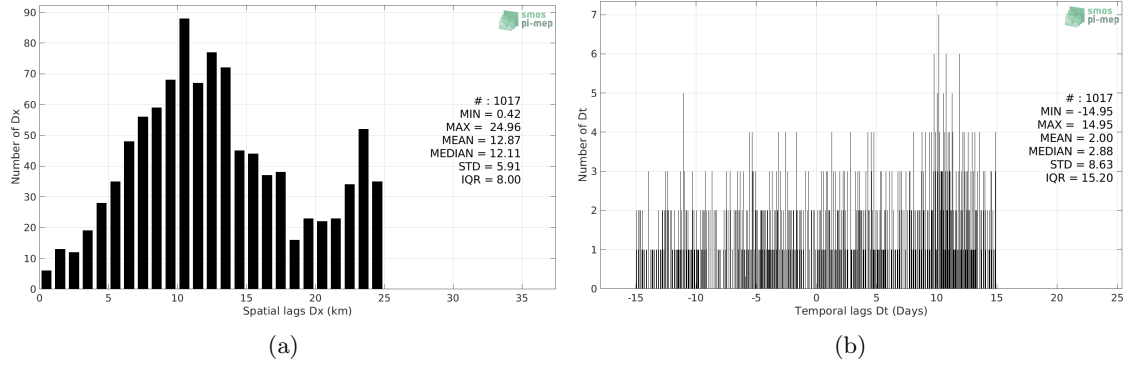
Figure 5: Histograms of the spatial (a) and temporal (b) lags between the location/time of the Sea mammals measurement and the date of the corresponding SMOS SSS L3 Arctic v1.1 - Monthly (CATDS-CECOS-LOCEAN) SSS pixel.
