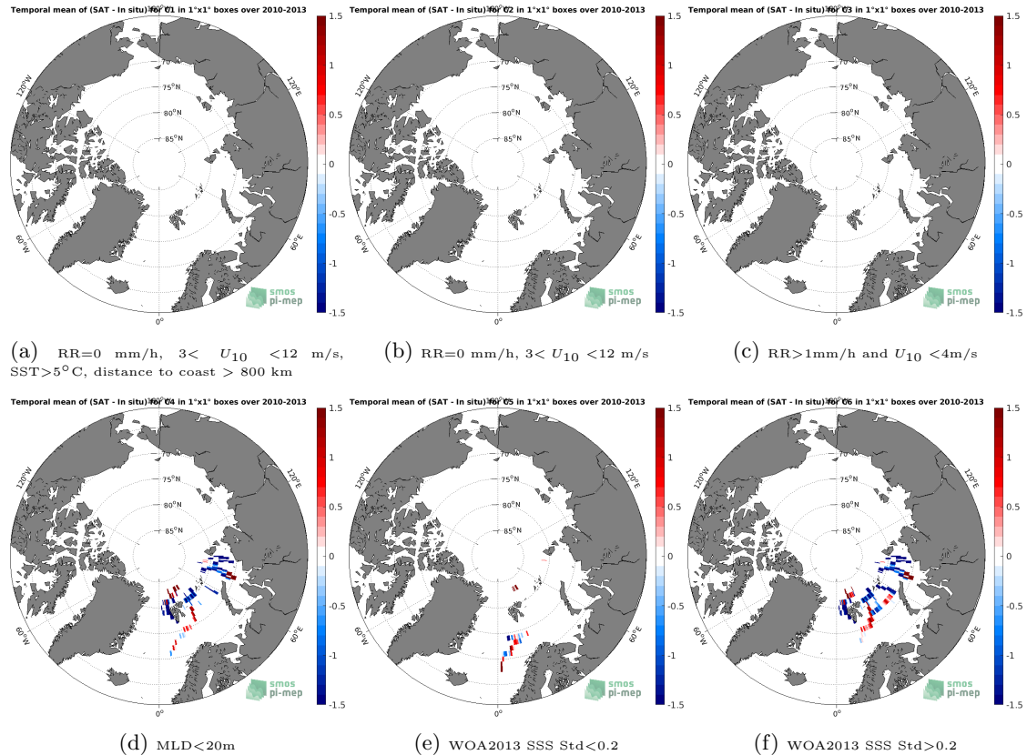
Figure 12: Temporal mean gridded over spatial boxes of size 1^{\circ}\times 1^{\circ} of \Delta\text{SSS} (SMOS SSS L3 Arctic v1.1 - Monthly (CATDS-CECOS-LOCEAN) - Sea mammals) for 6 different subdatasets corresponding to: RR=0 mm/h, 3 < U_{10} < 12 m/s, SST > 5^{\circ}\text{C} , distance to coast > 800 km (a), RR=0 mm/h, 3 < U_{10} < 12 m/s (b), RR > 1 mm/h and U_{10} < 4 m/s (c), MLD < 20 m (d), WOA2013 SSS Std < 0.2 (e), WOA2013 SSS Std > 0.2 (f).
