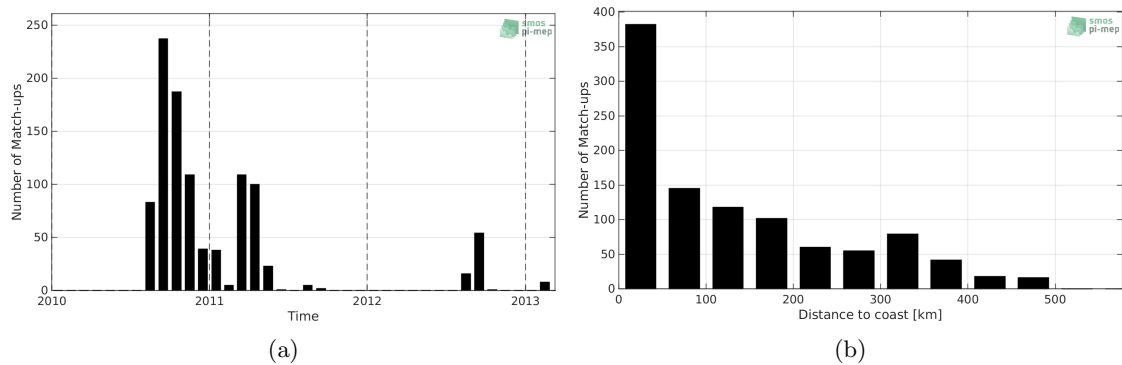
Figure 1: Number of match-ups between Sea mammals and SMOS SSS L3 Arctic v1.1 - Monthly (CATDS-CECOS-LOCEAN) SSS as a function of time (a) and as function of the distance to coast (b) over the Arctic Ocean Pi-MEP region and for the full satellite product period.
