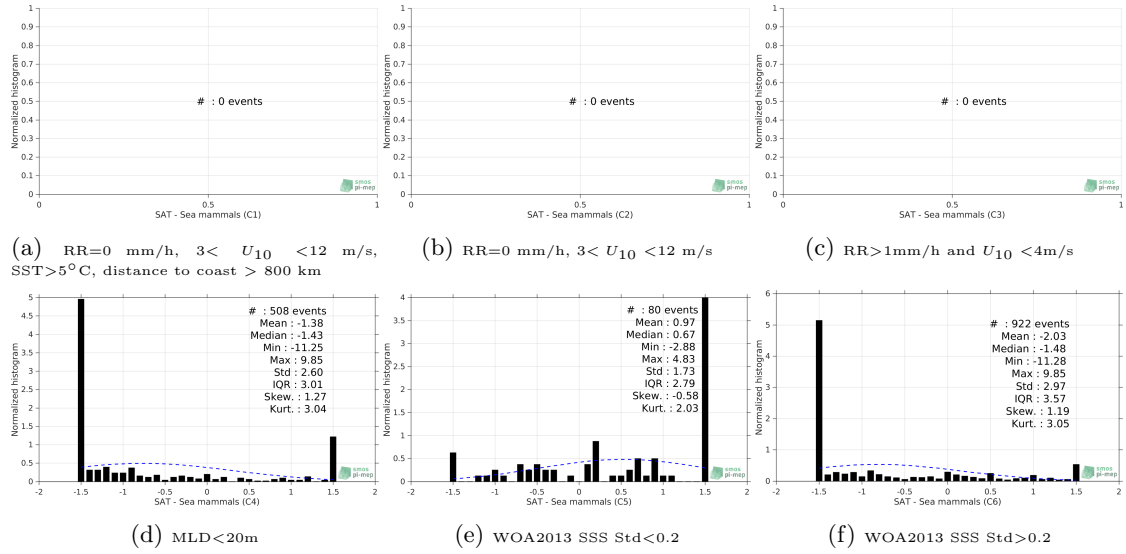
Figure 13: Normalized histogram of \Delta SSS (SMOS SSS L3 Arctic v1.1 - Monthly (CATDS-CECOS-LOCEAN) - Sea mammals) for 6 different subdatasets corresponding to: RR=0 mm/h, 3 < U_{10} < 12 m/s, SST > 5°C, distance to coast > 800 km (a), RR=0 mm/h, 3 < U_{10} < 12 m/s (b), RR > 1mm/h and U_{10} < 4 m/s (c), MLD < 20m (d), WOA2013 SSS Std < 0.2 (e), WOA2013 SSS Std > 0.2 (f).
