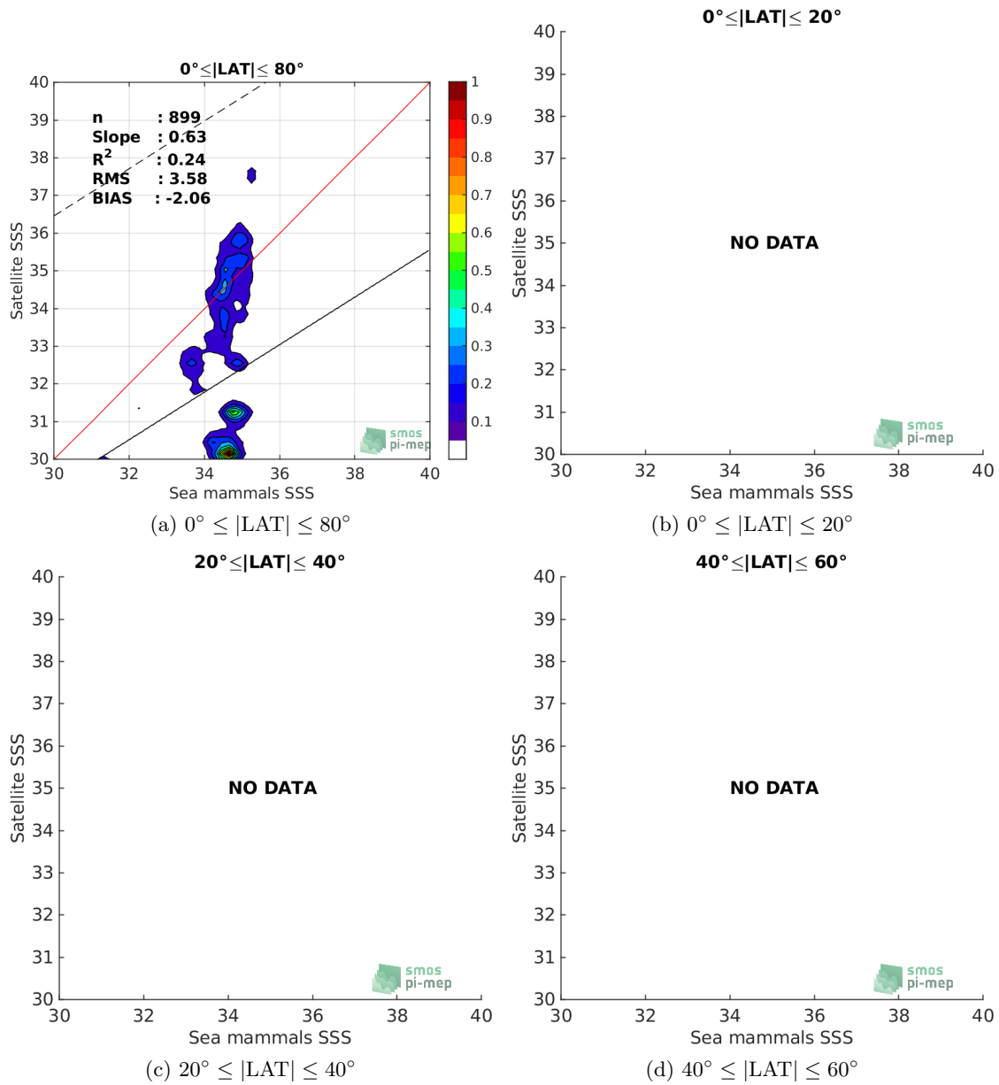
Figure 9: Contour maps of the concentration of SMOS SSS L3 Arctic v1.1 - Monthly (CATDS-CECOS-LOCEAN) SSS (y-axis) versus Sea mammals SSS (x-axis) at match-up pairs for different latitude bands. For each plot, the red line shows x=y . The black thin and dashed lines indicate a linear fit through the data cloud and the \pm 95\% confidence levels, respectively. The number match-up pairs n , the slope and R^2 coefficient of the linear fit, the root mean square (RMS) and the mean bias between satellite and in situ data are indicated for each latitude band in each plots.
