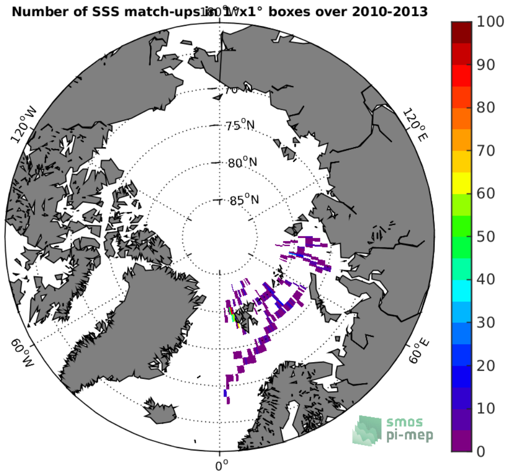
Figure 4: Number of SSS match-ups between Sea mammals SSS and the SMOS SSS L3 Arctic v1.1 - Monthly (CATDS-CECOS-LOCEAN) SSS product for the Arctic Ocean Pi-MEP region over 1°x1° boxes and for the full satellite product period.
