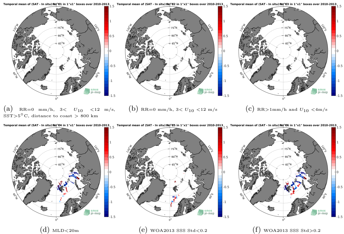
Figure 12: Temporal mean gridded over spatial boxes of size 1^{\circ}\times 1^{\circ} of \Delta\text{SSS} (SMOS SSS L3 Arctic v1.1 - Monthly (CATDS-CECOS-LOCEAN) - Sea mammals) for 6 different subdatasets corresponding to:RR=0 mm/h, 3 < U_{10} < 12 m/s, SST >5^{\circ}\text{C} , distance to coast > 800 km (a), RR=0 mm/h, 3 < U_{10} < 12 m/s (b), RR >1 mm/h and U_{10} < 4 m/s (c),MLD <20 m (d),WOA2013 SSS Std <0.2 (e),WOA2013 SSS Std >0.2 (f).
