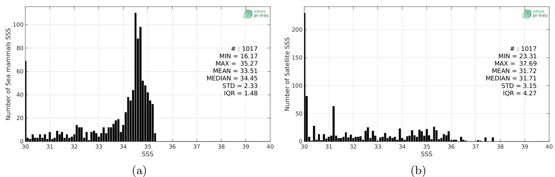
Figure 2: Histograms of SSS from Sea mammals (a) and SMOS SSS L3 Arctic v1.1 - Monthly (CATDS-CECOS-LOCEAN) (b) considering all match-up pairs per bins of 0.1 over the Arctic Ocean Pi-MEP region and for the full satellite product period.
