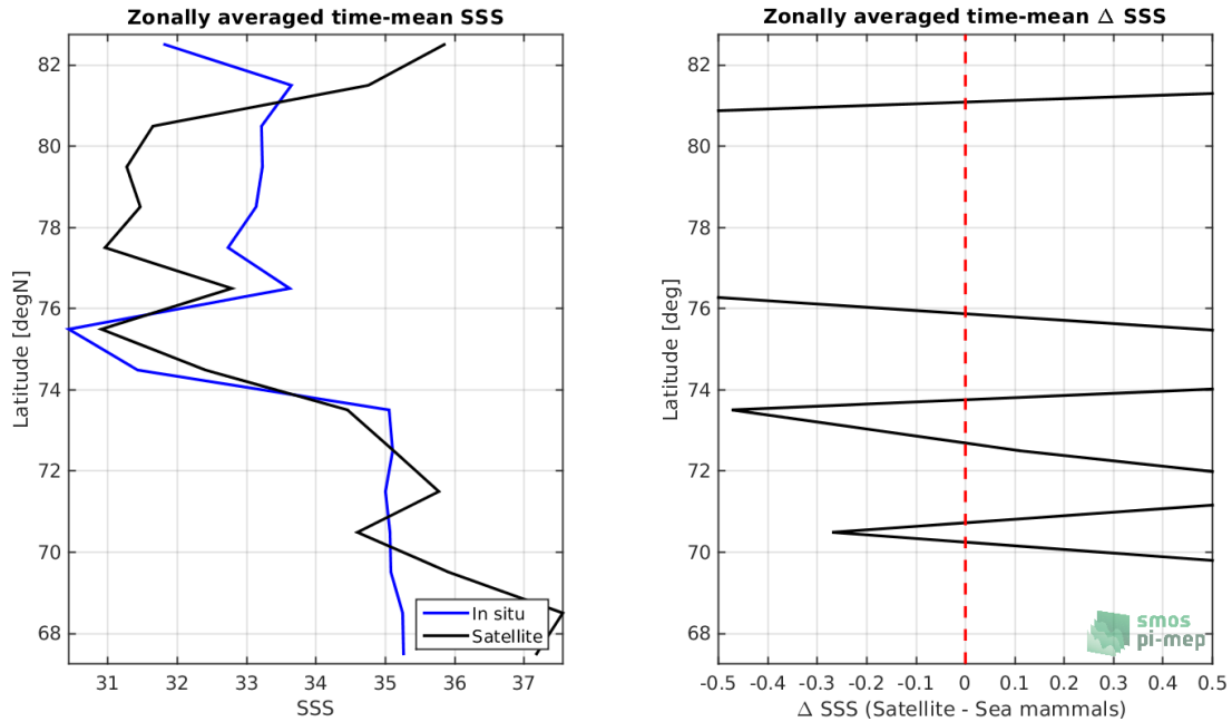
Figure 8: Left panel: Zonal mean SSS from SMOS SSS L3 Arctic v1.1 - Monthly (CATDS-CECOS-LOCEAN) satellite product (black) and from Sea mammals (blue). Right panel: Zonal mean of \Delta SSS (Satellite - Sea mammals) for all the collected Pi-MEP match-up pairs estimated over the full satellite product period.
