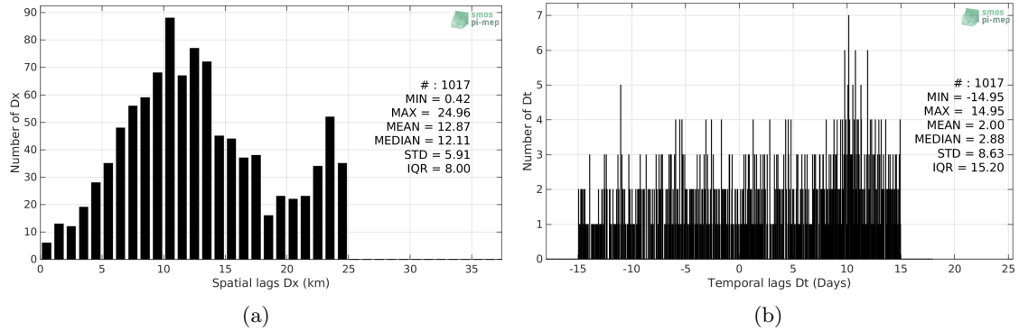
Figure 5: Histograms of the spatial (a) and temporal (b) lags between the time of the Sea mammals measurements and the date of the corresponding SMOS SSS L3 Arctic v1.1 - Monthly (CATDS-CECOS-LOCEAN) SSS product.
