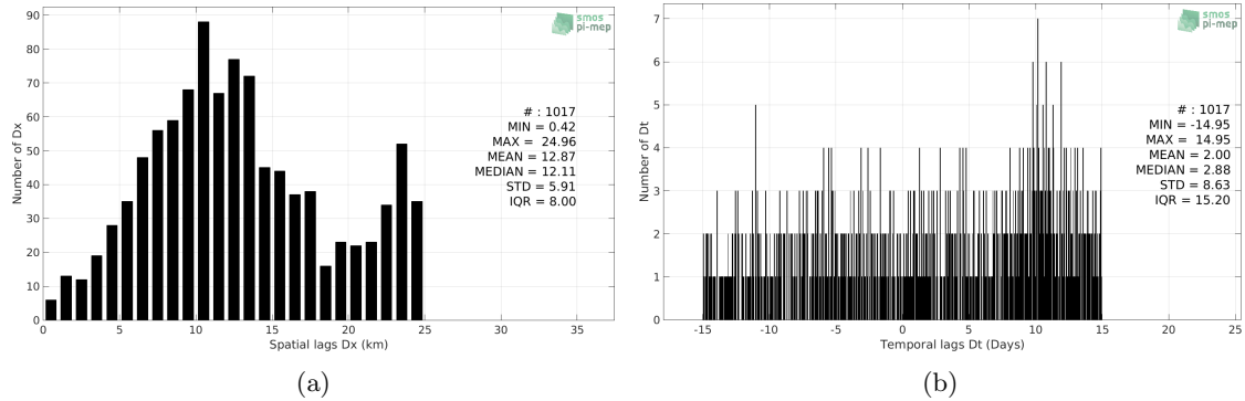
Figure 5: Histograms of the spatial (a) and temporal (b) lags between the time of the Sea mammals measurements and the date of the corresponding SMOS SSS L3 ARCTIC v1.1 - Monthly (CATDS-CECOS-LOCEAN) SSS product.
