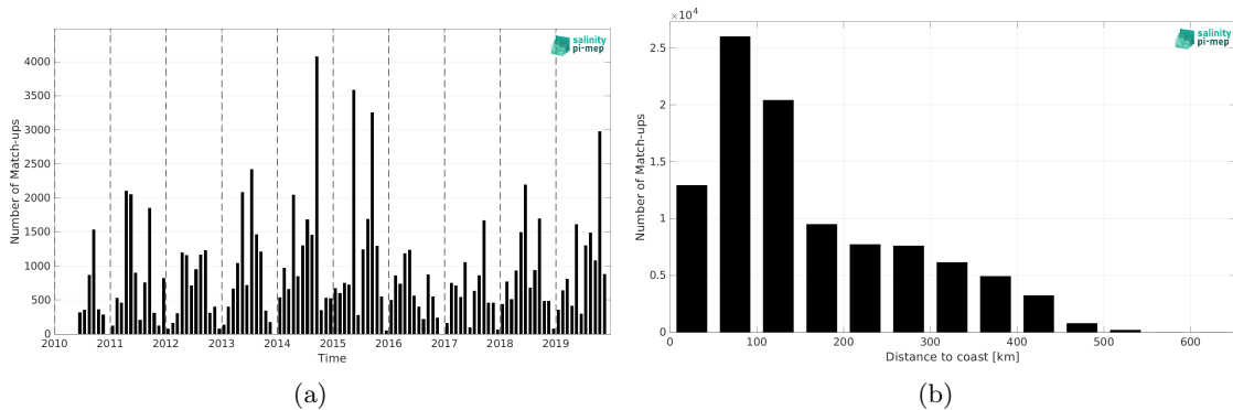
Figure 1: Number of match-ups between ICES and SMOS SSS L3 Arctic v1.1 - Monthly (CATDS-CECOS-LOCEAN) SSS as a function of time (a) and as function of the distance to coast (b) over the Arctic Ocean Pi-MEP region and for the full satellite product period.
