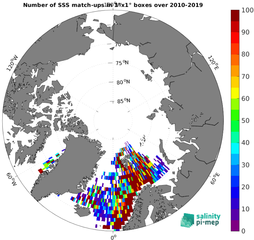
Figure 4: Number of SSS match-ups between ICES SSS and the SMOS SSS L3 Arctic v1.1 - Monthly (CATDS-CECOS-LOCEAN) SSS product for the Arctic Ocean Pi-MEP region over 1^\circ \times 1^\circ boxes and for the full satellite product period.
