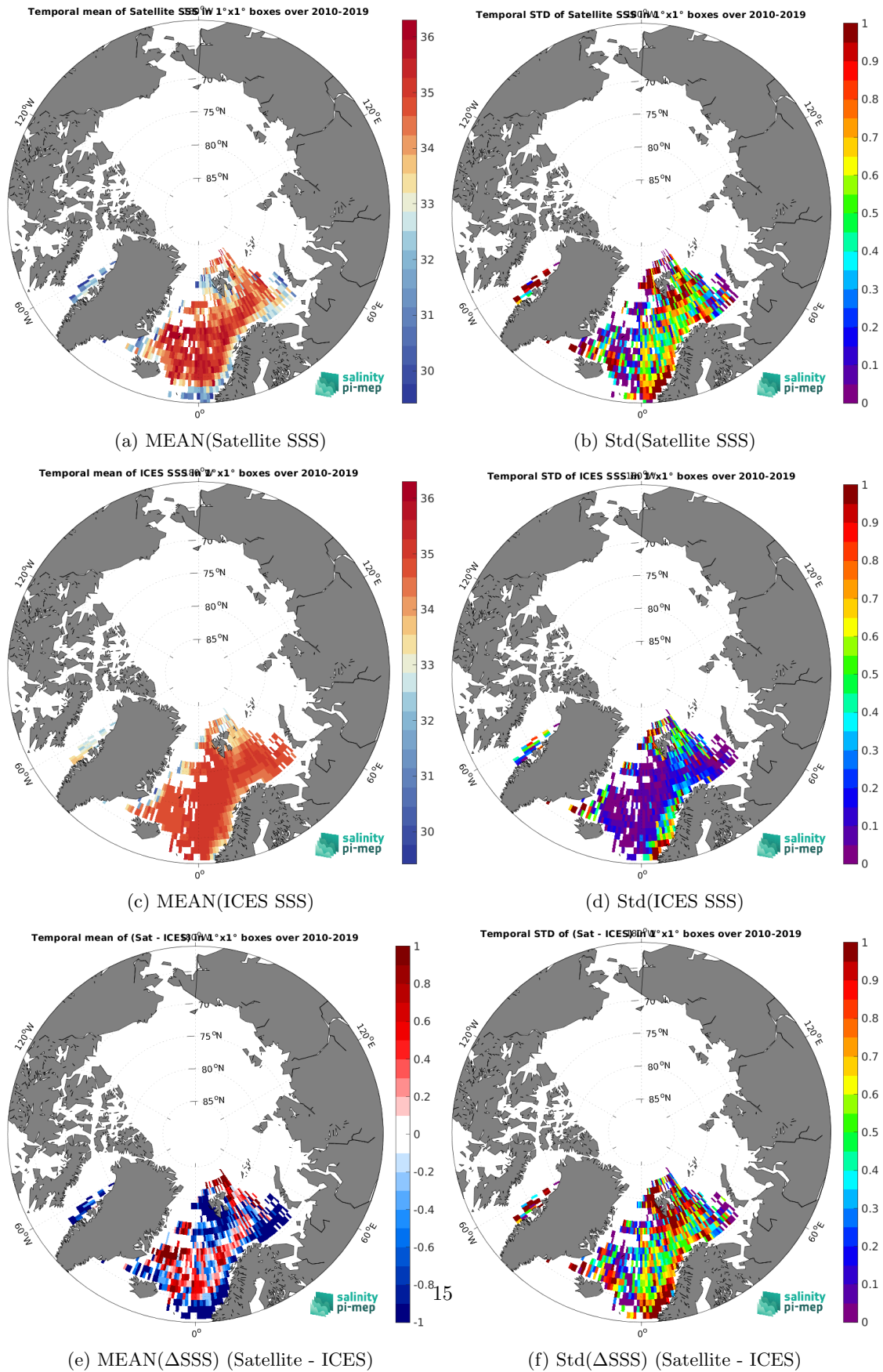
Figure 6: Temporal mean (left) and Std (right) of SSS from SMOS SSS L3 Arctic v1.1 - Monthly (CATDS-CECOS-LOCEAN) (top), ICES (middle), and of \Delta SSS (Satellite - ICES). Only match-up pairs are used to generate these maps.
