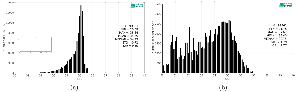
Figure 2: Histograms of SSS from ICES (a) and SMOS SSS L3 Arctic v1.1 - Monthly (CATDS-CECOS-LOCEAN) (b) considering all match-up pairs per bins of 0.1 over the Arctic Ocean Pi-MEP region and for the full satellite product period.
