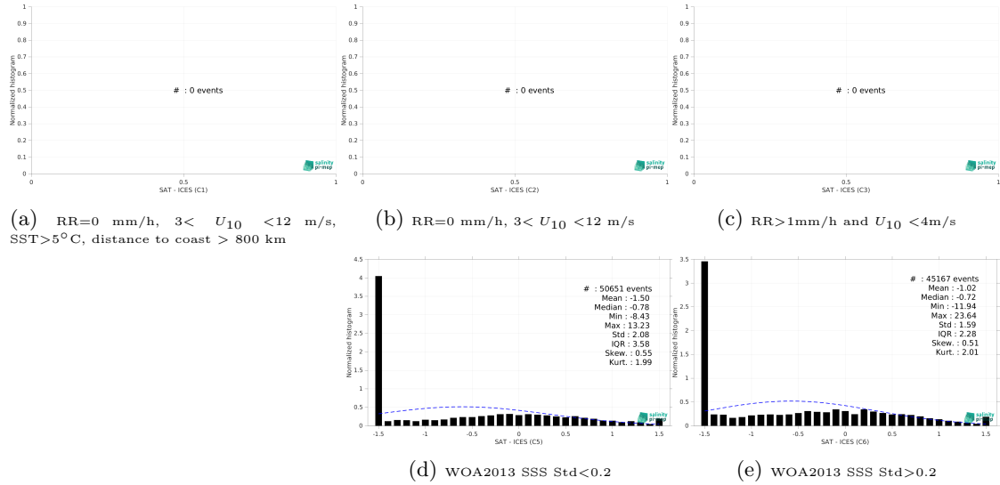
Figure 13: Normalized histogram of \Delta SSS (SMOS SSS L3 Arctic v1.1 - Monthly (CATDS-CECOS-LOCEAN) - ICES) for 5 different subdatasets corresponding to: RR=0 mm/h, 3 < U_{10} < 12 m/s, SST > 5°C, distance to coast > 800 km (a), RR=0 mm/h, 3 < U_{10} < 12 m/s (b), RR > 1mm/h and U_{10} < 4 m/s (c), WOA2013 SSS Std < 0.2 (d), WOA2013 SSS Std > 0.2 (e).
