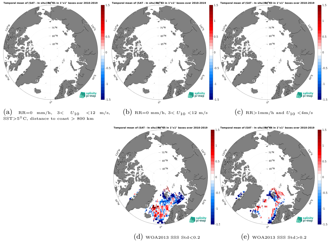
Figure 12: Temporal mean gridded over spatial boxes of size 1^{\circ}\times 1^{\circ} of \Delta\text{SSS} (SMOS SSS L3 Arctic v1.1 - Monthly (CATDS-CECOS-LOCEAN) - ICES) for 5 different subdatasets corresponding to:RR=0 mm/h, 3 < U_{10} < 12 m/s, SST >5^{\circ}\text{C} , distance to coast > 800 km (a), RR=0 mm/h, 3 < U_{10} < 12 m/s (b), RR >1 mm/h and U_{10} < 4 m/s (c), WOA2013 SSS Std <0.2 (d), WOA2013 SSS Std >0.2 (e).
