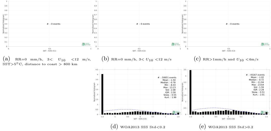
Figure 13: Normalized histogram of \Delta SSS (SMOS SSS L3 Arctic v1.1 - Monthly (CATDS-CECOS-LOCEAN) - ICES) for 5 different subdatasets corresponding to: RR=0 mm/h, 3 < U_{10} < 12 m/s, SST >5^{\circ} C, distance to coast > 800 km (a), RR=0 mm/h, 3 < U_{10} < 12 m/s (b), RR >1 mm/h and U_{10} < 4 m/s (c), WOA2013 SSS Std <0.2 (d), WOA2013 SSS Std >0.2 (e).
