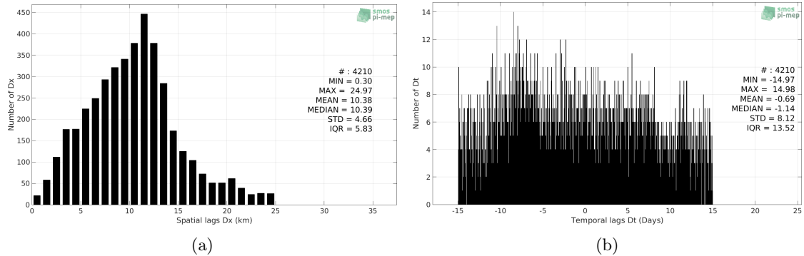
Figure 4: Histograms of the spatial (a) and temporal (b) lags between the time of the Surface drifters measurements and the date of the corresponding SMOS SSS L3 ARCTIC v1.1 - Monthly (CATDS-CECOS-LOCEAN) SSS product.
