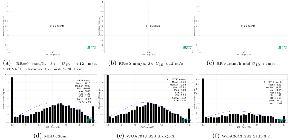
Figure 13: Normalized histogram of \Delta SSS (SMOS SSS L3 Arctic v1.1 - Monthly (CATDS-CECOS-LOCEAN) - Argo) for 6 different subdatasets corresponding to: RR=0 mm/h, 3 < U_{10} < 12 m/s, SST > 5°C, distance to coast > 800 km (a), RR=0 mm/h, 3 < U_{10} < 12 m/s (b), RR > 1mm/h and U_{10} < 4 m/s (c), MLD < 20m (d), WOA2013 SSS Std < 0.2 (e), WOA2013 SSS Std > 0.2 (f).
