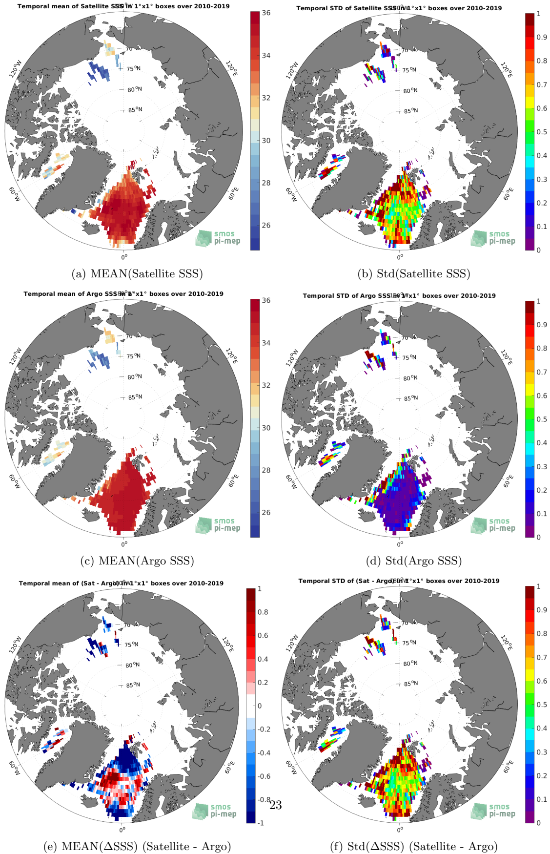
Figure 6: Temporal mean (left) and Std (right) of SSS from SMOS SSS L3 Arctic v1.1 - Monthly (CATDS-CECOS-LOCEAN) (top), Argo (middle), and of \Delta SSS (Satellite - Argo). Only match-pairs are used to generate these maps.
