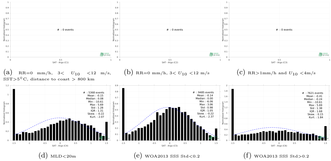
Figure 13: Normalized histogram of \Delta SSS (SMOS SSS L3 Arctic v1.1 - Monthly (CATDS-CECOS-LOCEAN) - Argo) for 6 different subdatasets corresponding to: RR=0 mm/h, 3 < U_{10} < 12 m/s, SST>5°C, distance to coast > 800 km (a), RR=0 mm/h, 3 < U_{10} < 12 m/s (b), RR>1mm/h and U_{10} < 4 m/s (c), MLD<20m (d), WOA2013 SSS Std<0.2 (e), WOA2013 SSS Std>0.2 (f).
