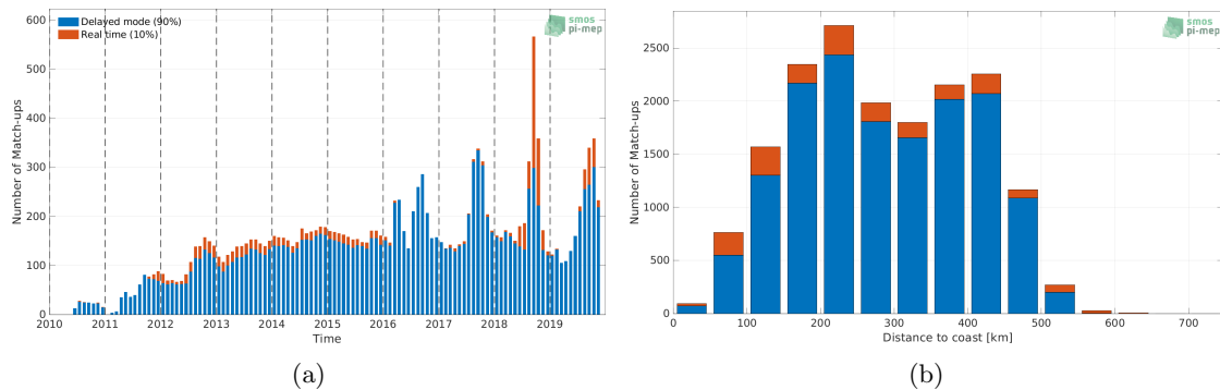
Figure 1: Number of match-ups between Argo and SMOS SSS L3 Arctic v1.1 - Monthly (CATDS-CECOS-LOCEAN) SSS as a function of time (a) and as function of the distance to coast (b) over the Arctic Ocean Pi-MEP region and for the full satellite product period.
