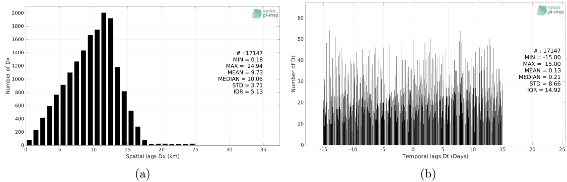
Figure 5: Histograms of the spatial (a) and temporal (b) lags between the location/time of the Argo measurement and the date of the corresponding SMOS SSS L3 Arctic v1.1 - Monthly (CATDS-CECOS-LOCEAN) SSS pixel.
