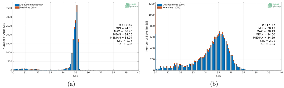
Figure 2: Histograms of SSS from Argo (a) and SMOS SSS L3 Arctic v1.1 - Monthly (CATDS-CECOS-LOCEAN) (b) considering all match-up pairs per bins of 0.1 over the Arctic Ocean Pi-MEP region and for the full satellite product period.
