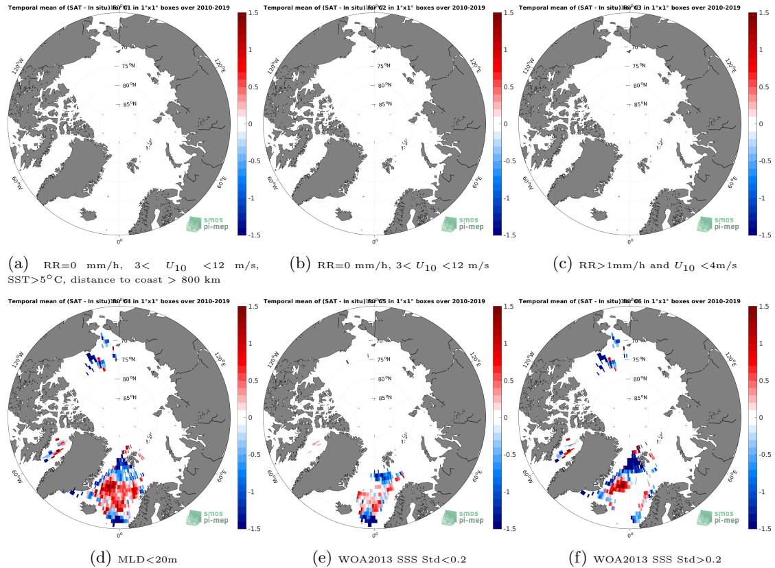
Figure 12: Temporal mean gridded over spatial boxes of size 1^{\circ}\times 1^{\circ} of \Delta\text{SSS} (SMOS SSS L3 Arctic v1.1 - Monthly (CATDS-CECOS-LOCEAN) - Argo) for 6 different subdatasets corresponding to: RR=0 mm/h, 3 < U_{10} < 12 m/s, SST > 5^{\circ}\text{C} , distance to coast > 800 km (a), RR=0 mm/h, 3 < U_{10} < 12 m/s (b), RR > 1 mm/h and U_{10} < 4 m/s (c), MLD < 20\text{m} (d), WOA2013 SSS Std < 0.2 (e), WOA2013 SSS Std > 0.2 (f).
