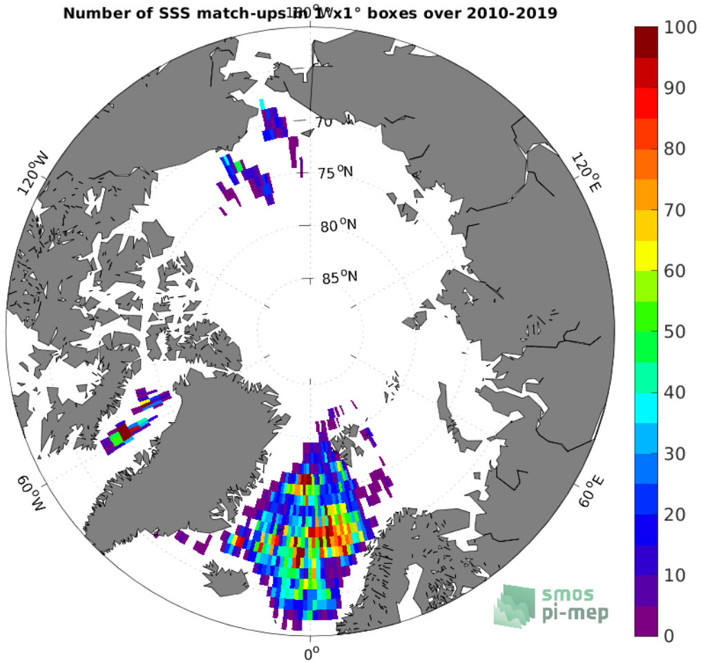
Figure 4: Number of SSS match-ups between Argo SSS and the SMOS SSS L3 Arctic v1.1 - Monthly (CATDS-CECOS-LOCEAN) SSS product for the Arctic Ocean Pi-MEP region over 1^{\circ} \times 1^{\circ} boxes and for the full satellite product period.
