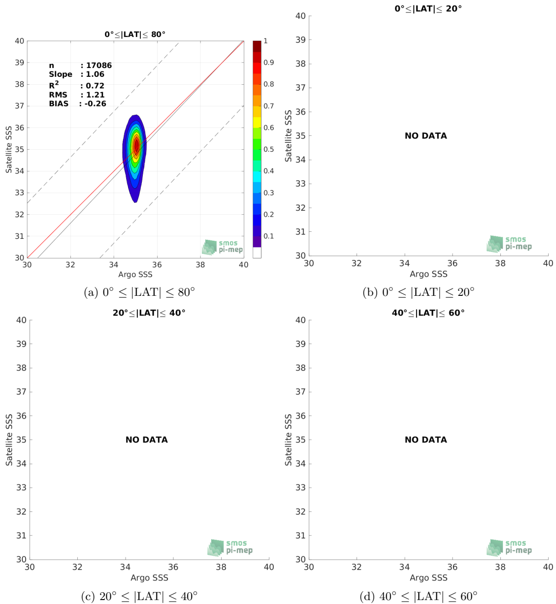
Figure 9: Contour maps of the concentration of SMOS SSS L3 Arctic v1.1 - Monthly (CATDS-CECOS-LOCEAN) SSS (y-axis) versus Argo SSS (x-axis) at match-up pairs for different latitude bands. For each plot, the red line shows x=y . The black thin and dashed lines indicate a linear fit through the data cloud and the \pm 95\% confidence levels, respectively. The number match-up pairs n , the slope and R^2 coefficient of the linear fit, the root mean square (RMS) and the mean bias between satellite and in situ data are indicated for each latitude band in each plots.
