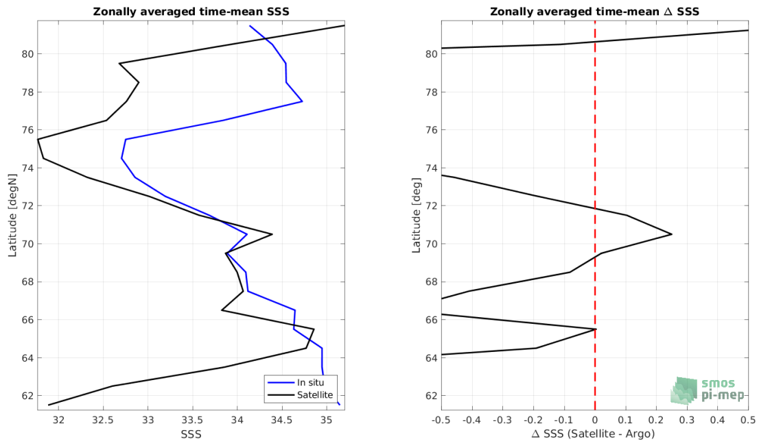
Figure 8: Left panel: Zonal mean SSS from SMOS SSS L3 Arctic v1.1 - Monthly (CATDS-CECOS-LOCEAN) satellite product (black) and from Argo (blue). Right panel: Zonal mean of \Delta SSS (Satellite - Argo) for all the collected Pi-MEP match-up pairs estimated over the full satellite product period.
