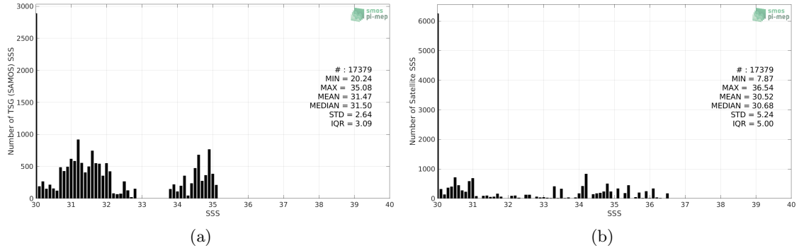
Figure 2: Histograms of SSS from TSG (SAMOS) (a) and SMOS SSS L3 v2 - Monthly - 0.25 Deg (CATDS-CECOS-IFREMER) (b) considering all match-up pairs per bins of 0.1 over the Arctic Ocean Pi-MEP region and for the full satellite product period.
