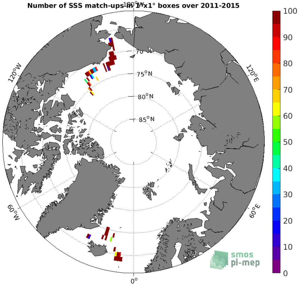
Figure 4: Number of SSS match-ups between TSG (SAMOS) SSS and the SMOS SSS L3 v2 - Monthly - 0.25 Deg (CATDS-CECOS-IFREMER) SSS product for the Arctic Ocean Pi-MEP region over 1°x1° boxes and for the full satellite product period.
