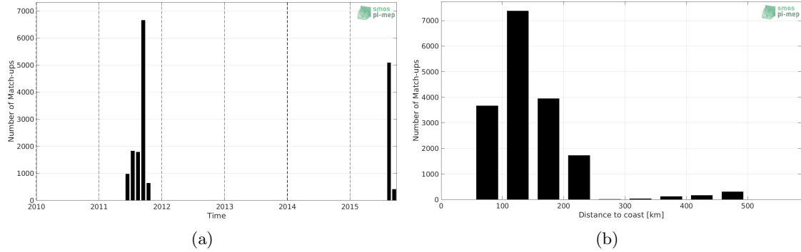
Figure 1: Number of match-ups between TSG (SAMOS) and SMOS SSS L3 v2 - Monthly - 0.25 Deg (CATDS-CECOS-IFREMER) SSS as a function of time (a) and as function of the distance to coast (b) over the Arctic Ocean Pi-MEP region and for the full satellite product period.
