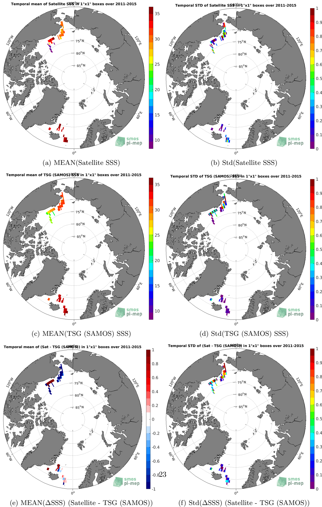
Figure 6: Temporal mean (left) and Std (right) of SSS from SMOS SSS L3 v2 - Monthly - 0.25 Deg (CATDS-CECOS-IFREMER) (top), TSG (SAMOS) (middle), and of \Delta SSS (Satellite - TSG (SAMOS)). Only match-up pairs are used to generate these maps.
