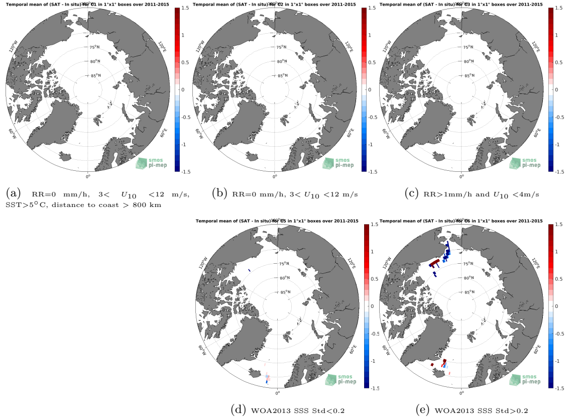
Figure 12: Temporal mean gridded over spatial boxes of size 1^{\circ}\times 1^{\circ} of \Delta\text{SSS} (SMOS SSS L3 v2 - Monthly - 0.25 Deg (CATDS-CECOS-IFREMER) - TSG (SAMOS)) for 5 different subdatasets corresponding to:RR=0 mm/h, 3 < U_{10} < 12 m/s, SST >5^{\circ}\text{C} , distance to coast > 800 km (a), RR=0 mm/h, 3 < U_{10} < 12 m/s (b), RR >1 mm/h and U_{10} < 4 m/s (c), WOA2013 SSS Std <0.2 (d), WOA2013 SSS Std >0.2 (e).
