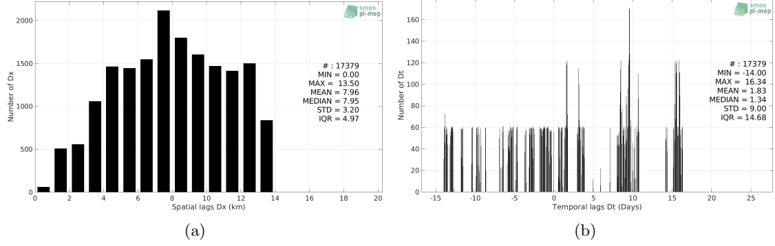
Figure 5: Histograms of the spatial (a) and temporal (b) lags between the location/time of the TSG (SAMOS) measurement and the date of the corresponding SMOS SSS L3 v2 - Monthly - 0.25 Deg (CATDS-CECOS-IFREMER) SSS pixel.
