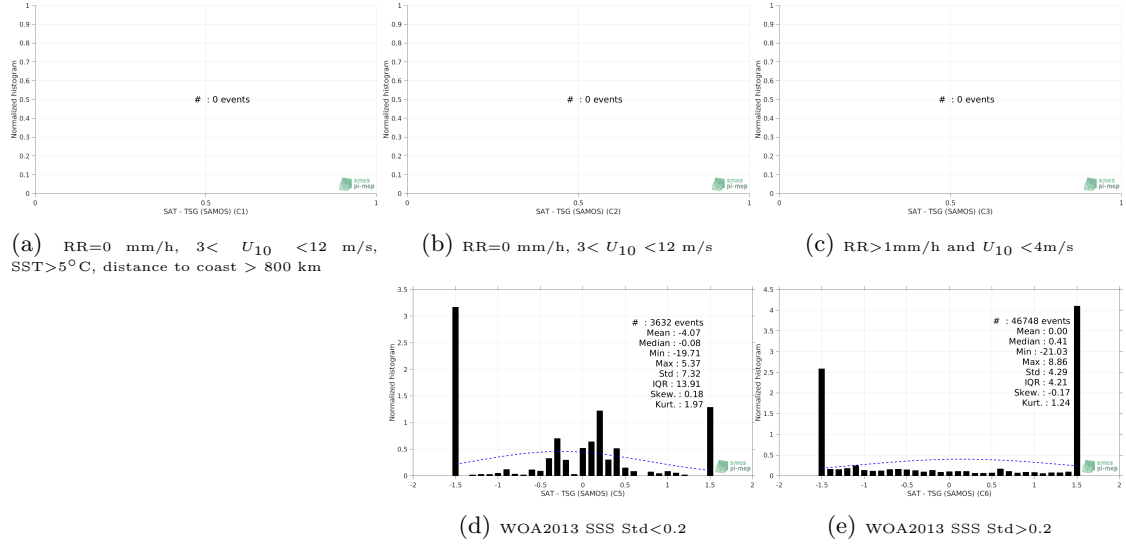
Figure 13: Normalized histogram of \Delta\text{SSS} (SMOS SSS L3 v2 - Monthly - 0.25 Deg (CATDS-CECOS-IFREMER) - TSG (SAMOS)) for 5 different subdatasets corresponding to: RR=0 mm/h, 3 < U_{10} < 12 m/s, SST > 5^\circ\text{C} , distance to coast > 800 km (a), RR=0 mm/h, 3 < U_{10} < 12 m/s (b), RR > 1\text{mm/h} and U_{10} < 4\text{m/s} (c), WOA2013 SSS Std<0.2 (d), WOA2013 SSS Std>0.2 (e).
