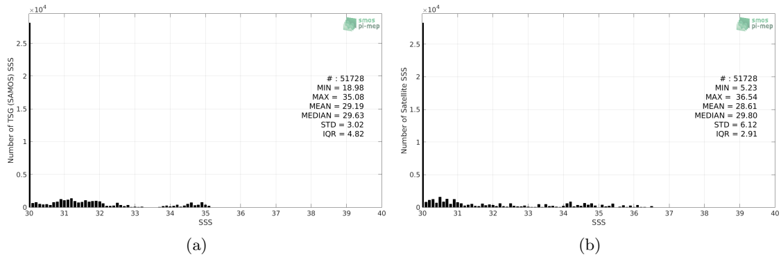
Figure 2: Histograms of SSS from TSG (SAMOS) (a) and SMOS SSS L3 v2 - Monthly - 0.25 Deg (CATDS-CECOS-IFREMER) (b) considering all match-up pairs per bins of 0.1 over the Arctic Ocean Pi-MEP region and for the full satellite product period.
