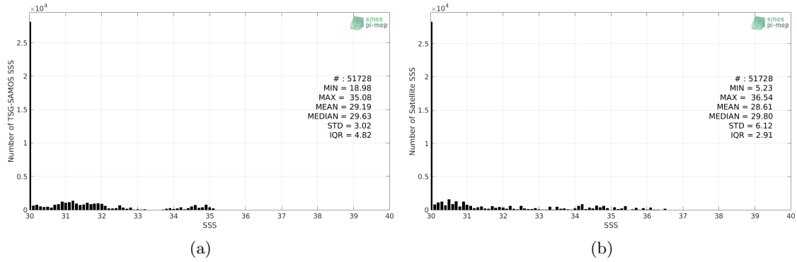
Figure 2: Histograms of SSS from TSG-SAMOS (a) and SMOS L3 v2 - Monthly - 0.25 Deg (CATDS-CECOS-IFREMER) (b) considering all match-up pairs per bins of 0.1 over the Arctic Ocean Pi-MEP region and for the full satellite product period.
