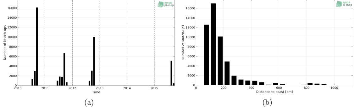
Figure 1: Number of match-ups between TSG-SAMOS and SMOS L3 v2 - Monthly - 0.25 Deg (CATDS-CECOS-IFREMER) SSS as a function of time (a) and as function of the distance to coast (b) over the Arctic Ocean Pi-MEP region and for the full satellite product period.
