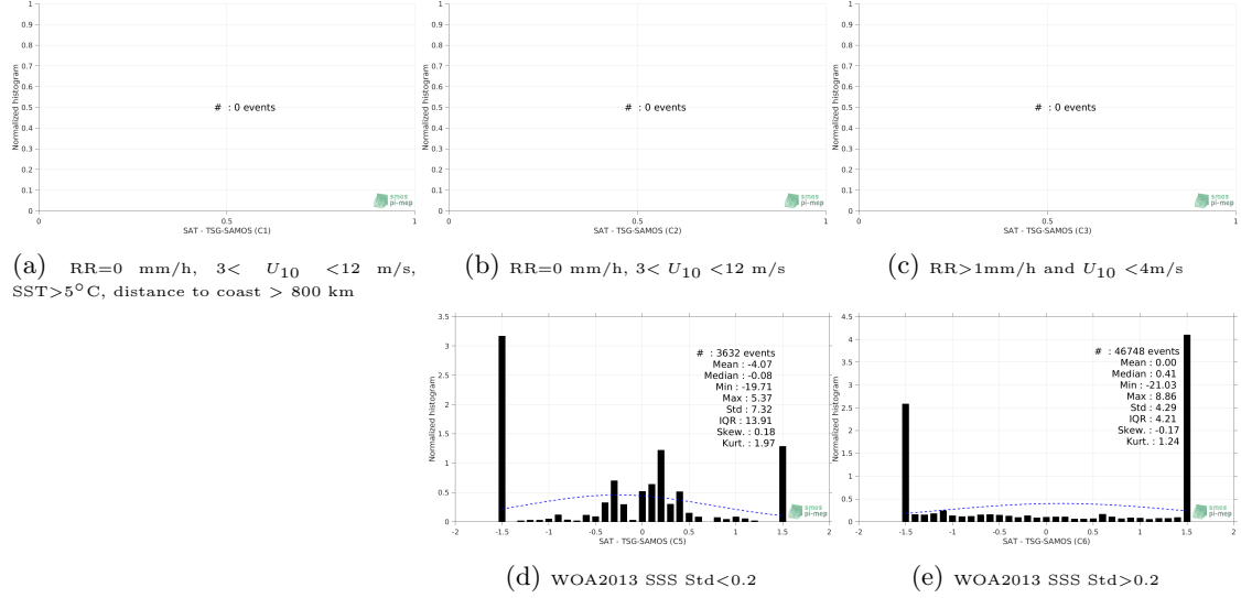
Figure 13: Normalized histogram of \Delta\text{SSS} (SMOS L3 v2 - Monthly - 0.25 Deg (CATDS-CECOS-IFREMER) - TSG-SAMOS) for 5 different subdatasets corresponding to: RR=0 mm/h, 3 < U_{10} < 12 m/s, SST > 5^\circ\text{C} , distance to coast > 800 km (a), RR=0 mm/h, 3 < U_{10} < 12 m/s (b), RR > 1\text{mm/h} and U_{10} < 4\text{m/s} (c), WOA2013 SSS Std < 0.2 (d), WOA2013 SSS Std > 0.2 (e).
