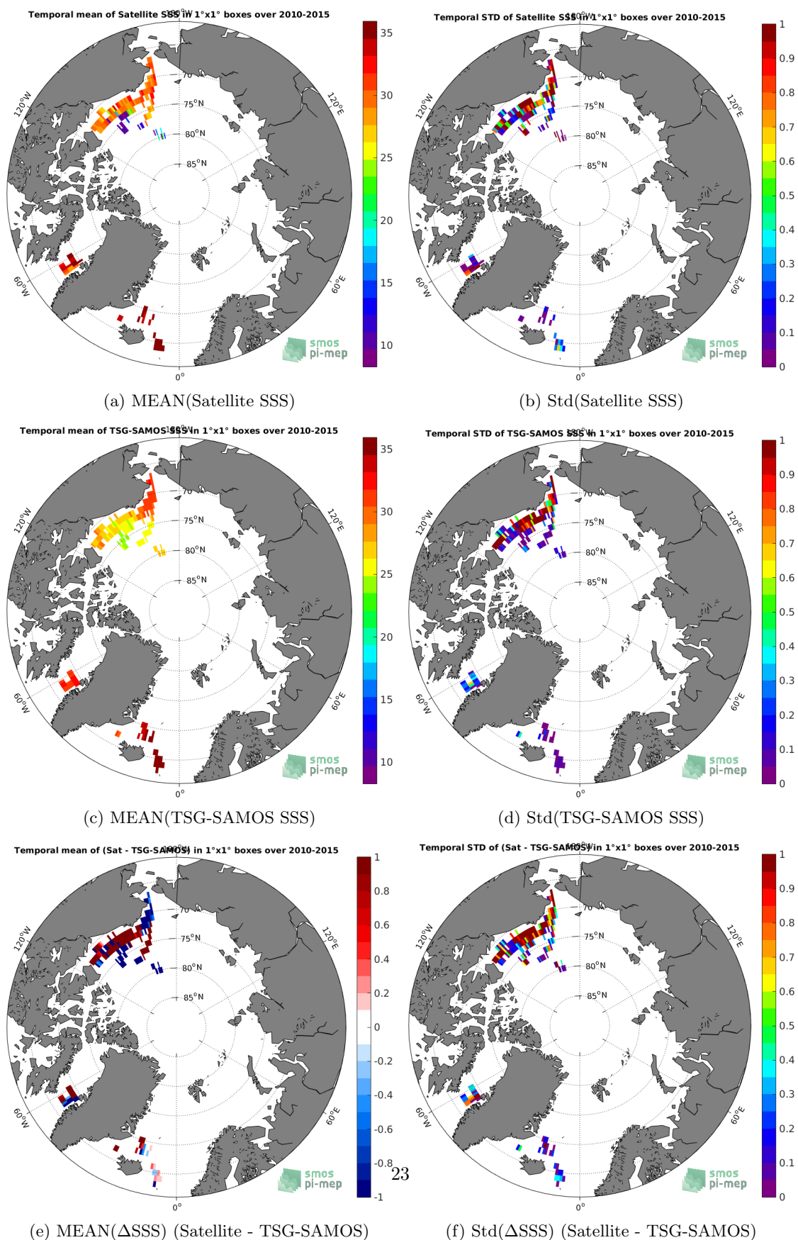
Figure 6: Temporal mean (left) and Std (right) of SSS from SMOS L3 v2 - Monthly - 0.25 Deg (CATDS-CECOS-IFREMER) (top), TSG-SAMOS (middle), and of \Delta SSS (Satellite - TSG-SAMOS). Only match-up pairs are used to generate these maps.
