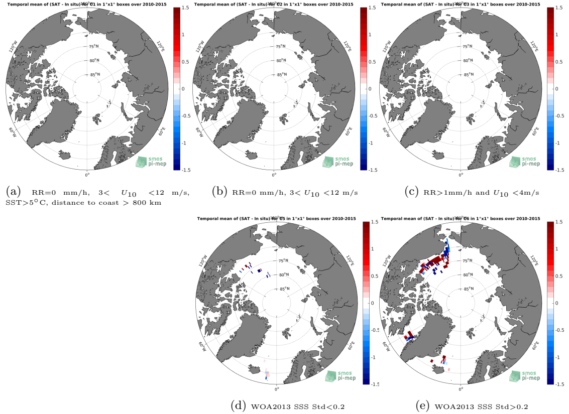
Figure 12: Temporal mean gridded over spatial boxes of size 1^{\circ}\times 1^{\circ} of \Delta\text{SSS} (SMOS L3 v2 - Monthly - 0.25^{\circ} Deg (CATDS-CECOS-IFREMER) - TSG-SAMOS) for 5 different subdatasets corresponding to: \text{RR}=0 mm/h, 3 < U_{10} < 12 m/s, \text{SST} > 5^{\circ}\text{C} , distance to coast > 800 km (a), \text{RR}=0 mm/h, 3 < U_{10} < 12 m/s (b), \text{RR} > 1 mm/h and U_{10} < 4 m/s (c), WOA2013 SSS Std < 0.2 (d), WOA2013 SSS Std > 0.2 (e).
