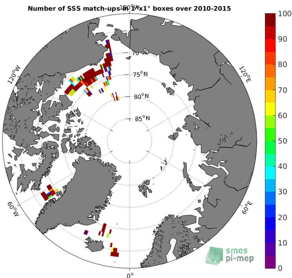
Figure 4: Number of SSS match-ups between TSG-SAMOS SSS and the SMOS L3 v2 - Monthly - 0.25 Deg (CATDS-CECOS-IFREMER) SSS product for the Arctic Ocean Pi-MEP region over 1^\circ \times 1^\circ boxes and for the full satellite product period.
