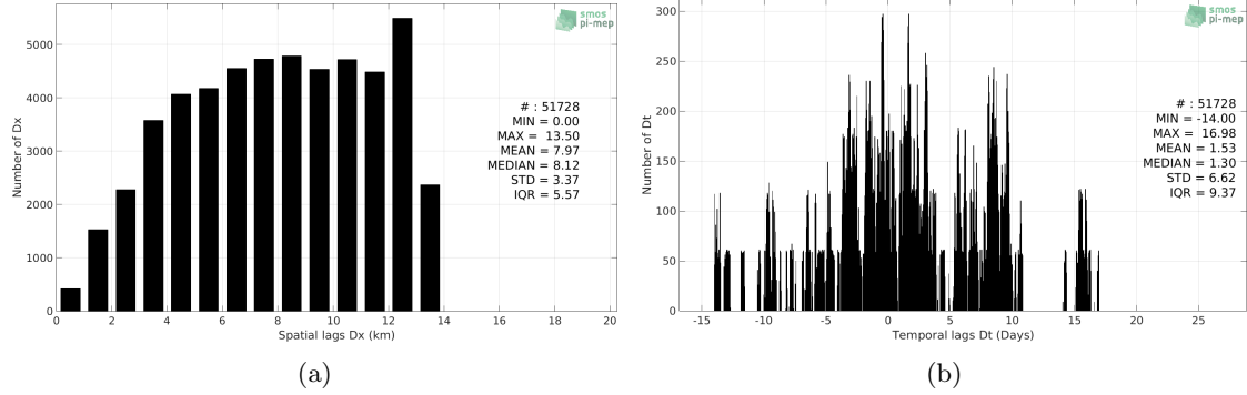
Figure 5: Histograms of the spatial (a) and temporal (b) lags between the time of the TSG-SAMOS measurements and the date of the corresponding SMOS L3 v2 - Monthly - 0.25 Deg (CATDS-CECOS-IFREMER) SSS product.
