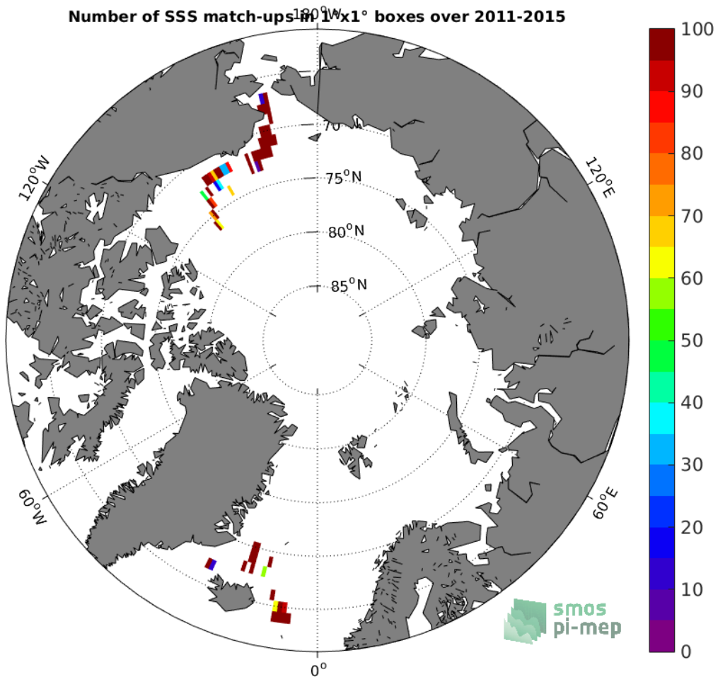
Figure 4: Number of SSS match-ups between TSG-SAMOS SSS and the SMOS-L3-CATDS-IFREMER-CECOS-V2-MONTHLY-0.25DEG SSS product for the Arctic Ocean Pi-MEP region over 1°x1° boxes and for the full satellite product period.
