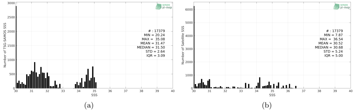
Figure 2: Histograms of SSS from TSG-SAMOS (a) and SMOS-L3-CATDS-IFREMER-CECOS-V2-MONTHLY-0.25DEG (b) considering all match-up pairs per bins of 0.1 over the Arctic Ocean Pi-MEP region and for the full satellite product period.
