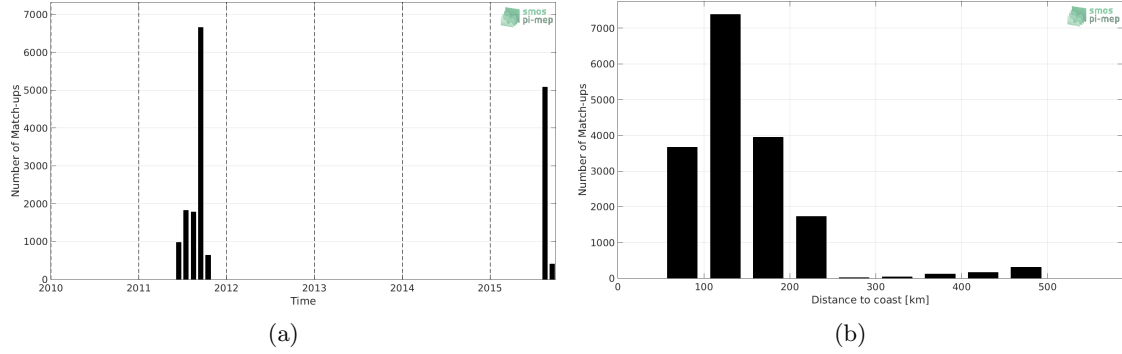
Figure 1: Number of match-ups between TSG-SAMOS and SMOS-L3-CATDS-IFREMER-CECOS-V2-MONTHLY-0.25DEG SSS as a function of time (a) and as function of the distance to coast (b) over the Arctic Ocean Pi-MEP region and for the full satellite product period.
