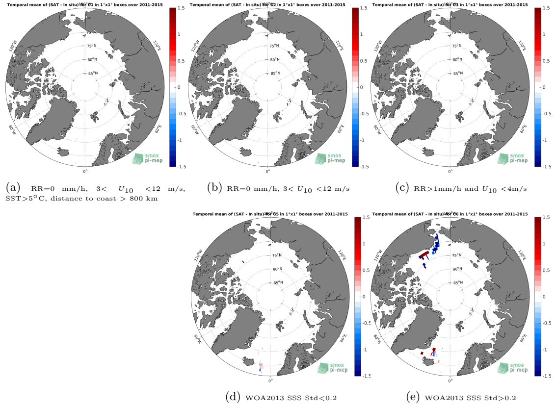
Figure 12: Temporal mean gridded over spatial boxes of size 1^\circ \times 1^\circ of \Delta SSS (SMOS-L3-CATDS-IFREMER-CECOS-V2-MONTHLY-0.25DEG - TSG-SAMOS) for 5 different subdatasets corresponding to:RR=0 mm/h, 3 < U_{10} < 12 m/s, SST >5^\circ\text{C} , distance to coast > 800 km (a), RR=0 mm/h, 3 < U_{10} < 12 m/s (b), RR >1 mm/h and U_{10} < 4 m/s (c), WOA2013 SSS Std <0.2 (d), WOA2013 SSS Std >0.2 (e).
