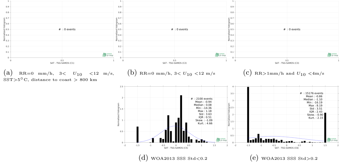
Figure 13: Normalized histogram of \Delta\text{SSS} (SMOS-L3-CATDS-IFREMER-CECOS-V2-MONTHLY-0.25DEG - TSG-SAMOS) for 5 different subdatasets corresponding to: RR=0 mm/h, 3 < U_{10} < 12 m/s, SST > 5^{\circ}\text{C} , distance to coast > 800 km (a), RR=0 mm/h, 3 < U_{10} < 12 m/s (b), RR > 1\text{mm/h} and U_{10} < 4\text{m/s} (c), WOA2013 SSS Std < 0.2 (d), WOA2013 SSS Std > 0.2 (e).
