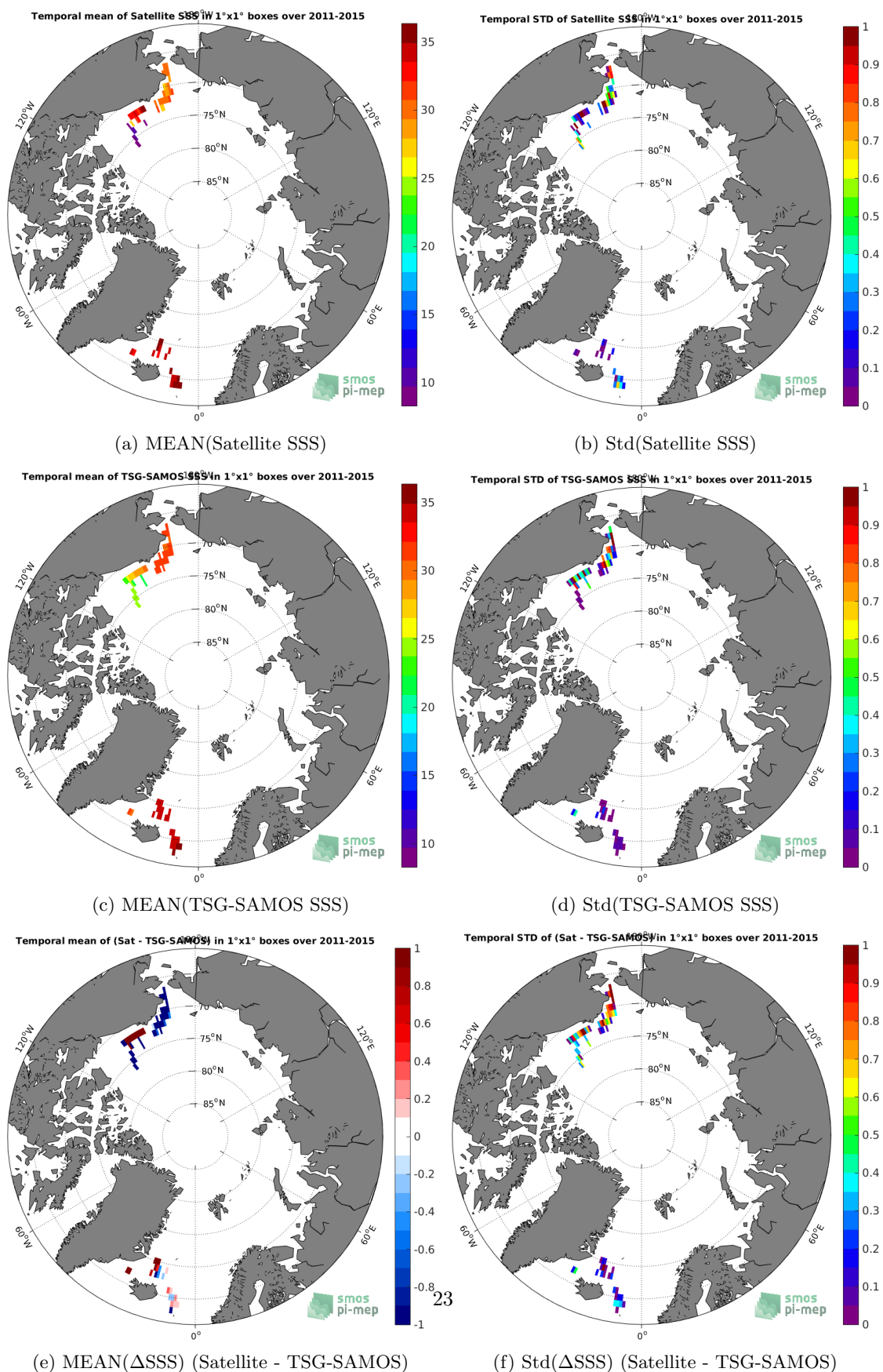
Figure 6: Temporal mean (left) and Std (right) of SSS from SMOS-L3-CATDS-IFREMER-CECOS-V2-MONTHLY-0.25DEG (top), TSG-SAMOS (middle), and of \Delta SSS (Satellite - TSG-SAMOS). Only match-up pairs are used to generate these maps.
