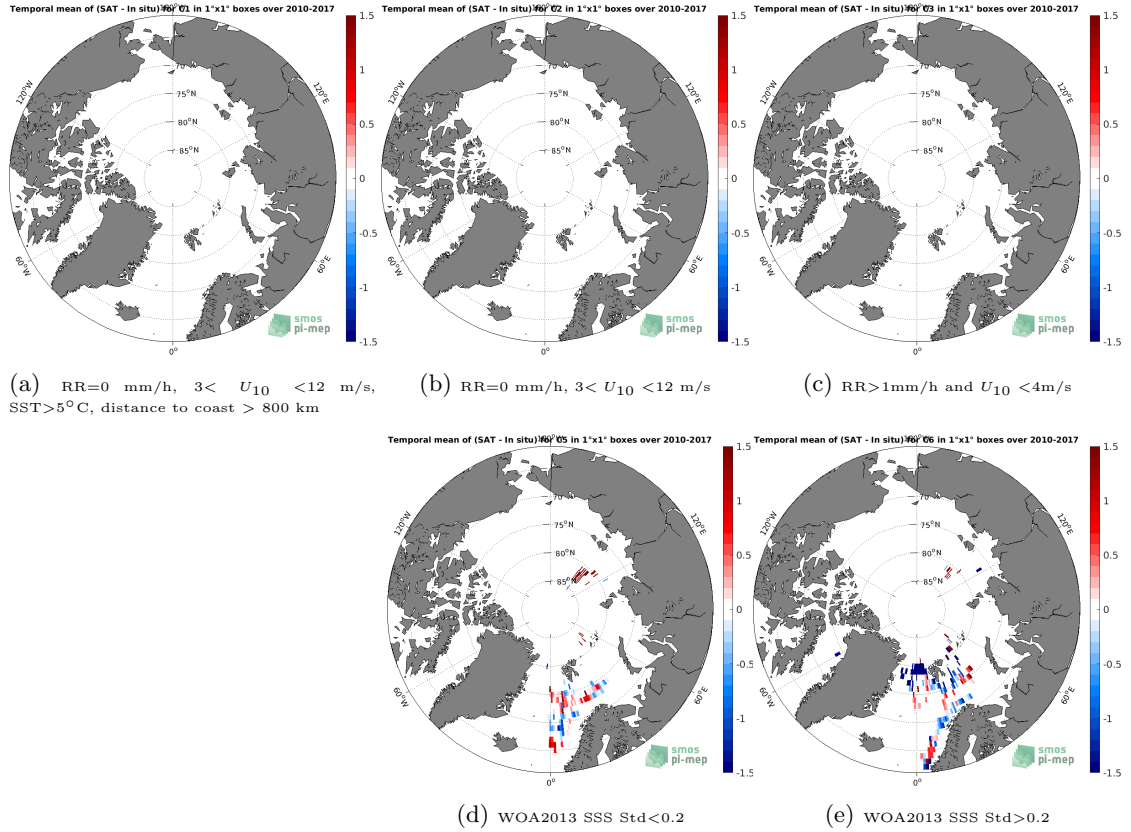
Figure 12: Temporal mean gridded over spatial boxes of size 1^{\circ}\times 1^{\circ} of \Delta\text{SSS} (SMOS SSS L3 v2 - Monthly - 0.25 Deg (CATDS-CECOS-IFREMER) - TSG (Polarstern)) for 5 different subdatasets corresponding to: RR=0 mm/h, 3 < U_{10} < 12 m/s, SST > 5^{\circ}\text{C} , distance to coast > 800 km (a), RR=0 mm/h, 3 < U_{10} < 12 m/s (b), RR > 1 mm/h and U_{10} < 4 m/s (c), WOA2013 SSS Std < 0.2 (d), WOA2013 SSS Std > 0.2 (e).
