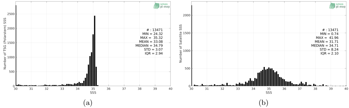
Figure 2: Histograms of SSS from TSG (Polarstern) (a) and SMOS SSS L3 v2 - Monthly - 0.25 Deg (CATDS-CECOS-IFREMER) (b) considering all match-up pairs per bins of 0.1 over the Arctic Ocean Pi-MEP region and for the full satellite product period.
