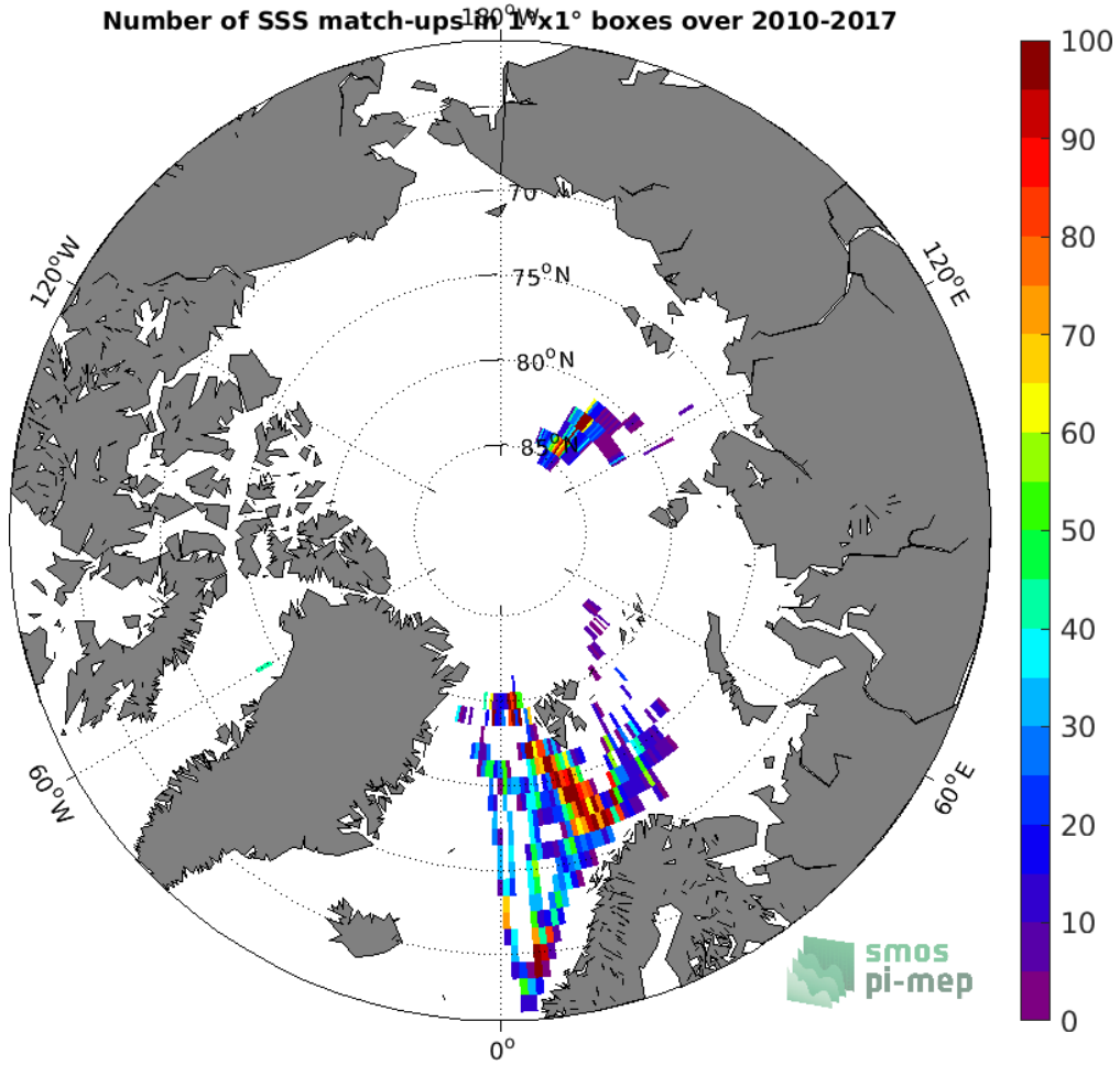
Figure 4: Number of SSS match-ups between TSG (Polarstern) SSS and the SMOS SSS L3 v2 - Monthly - 0.25 Deg (CATDS-CECOS-IFREMER) SSS product for the Arctic Ocean Pi-MEP region over 1°x1° boxes and for the full satellite product period.
