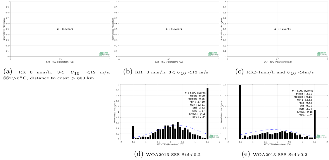
Figure 13: Normalized histogram of \Delta\text{SSS} (SMOS SSS L3 v2 - Monthly - 0.25 Deg (CATDS-CECOS-IFREMER) - TSG (Polarstern)) for 5 different subdatasets corresponding to: RR=0 mm/h, 3 < U_{10} < 12 m/s, SST > 5^\circ\text{C} , distance to coast > 800 km (a), RR=0 mm/h, 3 < U_{10} < 12 m/s (b), RR > 1 mm/h and U_{10} < 4 m/s (c), WOA2013 SSS Std < 0.2 (d), WOA2013 SSS Std > 0.2 (e).
