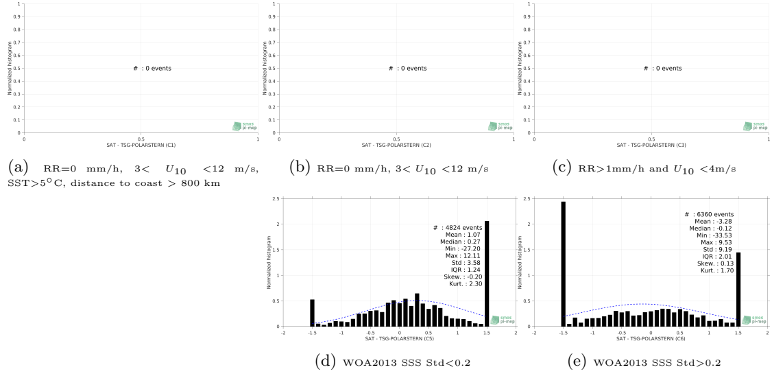
Figure 13: Normalized histogram of \Delta\text{SSS} (SMOS L3 v2 - Monthly - 0.25 Deg (CATDS-CECOS-IFREMER) - TSG-POLARSTERN) for 5 different subdatasets corresponding to: RR=0 mm/h, 3 < U_{10} < 12 m/s, SST > 5^\circ\text{C} , distance to coast > 800 km (a), RR=0 mm/h, 3 < U_{10} < 12 m/s (b), RR > 1\text{mm/h} and U_{10} < 4\text{m/s} (c), WOA2013 SSS Std < 0.2 (d), WOA2013 SSS Std > 0.2 (e).
