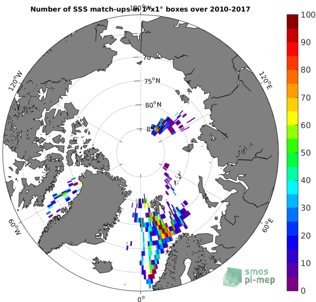
Figure 4: Number of SSS match-ups between TSG-POLARSTERN SSS and the SMOS L3 v2 - Monthly - 0.25 Deg (CATDS-CECOS-IFREMER) SSS product for the Arctic Ocean Pi-MEP region over 1°x1° boxes and for the full satellite product period.
