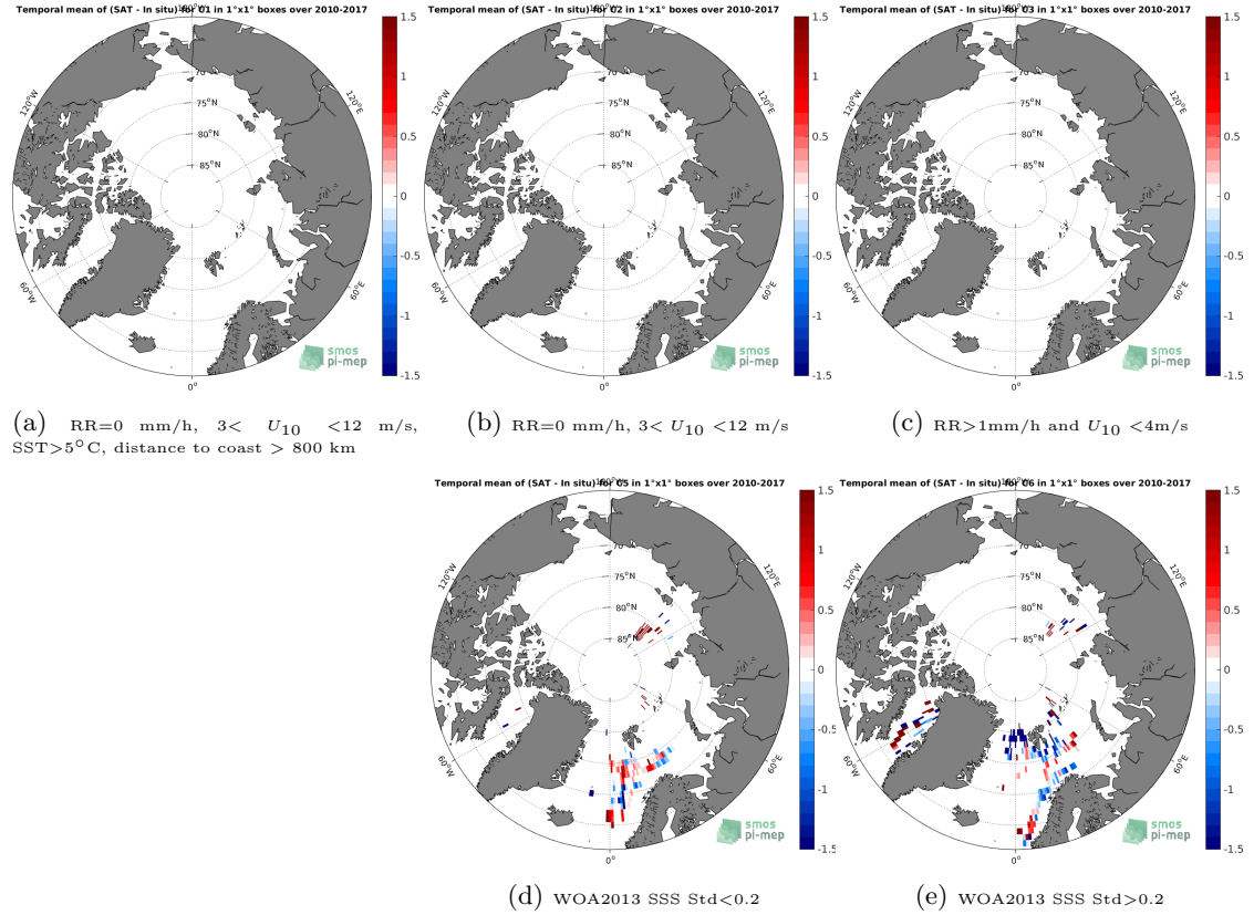
Figure 12: Temporal mean gridded over spatial boxes of size 1^{\circ}\times 1^{\circ} of \Delta\text{SSS} (SMOS L3 v2 - Monthly - 0.25 Deg (CATDS-CECOS-IFREMER) - TSG-POLARSTERN) for 5 different sub-datasets corresponding to: RR=0 mm/h, 3 < U_{10} < 12 m/s, SST >5^{\circ}\text{C} , distance to coast > 800 km (a), RR=0 mm/h, 3 < U_{10} < 12 m/s (b), RR >1 mm/h and U_{10} < 4 m/s (c), WOA2013 SSS Std <0.2 (d), WOA2013 SSS Std >0.2 (e).
