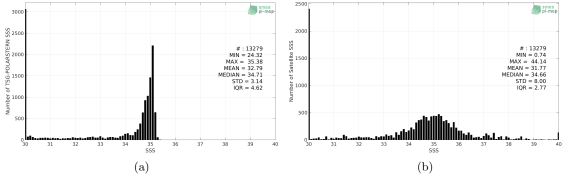
Figure 2: Histograms of SSS from TSG-POLARSTERN (a) and SMOS L3 v2 - Monthly - 0.25 Deg (CATDS-CECOS-IFREMER) (b) considering all match-up pairs per bins of 0.1 over the Arctic Ocean Pi-MEP region and for the full satellite product period.
