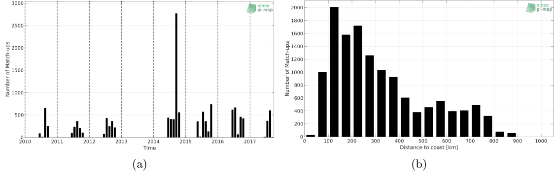
Figure 1: Number of match-ups between TSG-POLARSTERN and SMOS L3 v2 - Monthly - 0.25 Deg (CATDS-CECOS-IFREMER) SSS as a function of time (a) and as function of the distance to coast (b) over the Arctic Ocean Pi-MEP region and for the full satellite product period.
