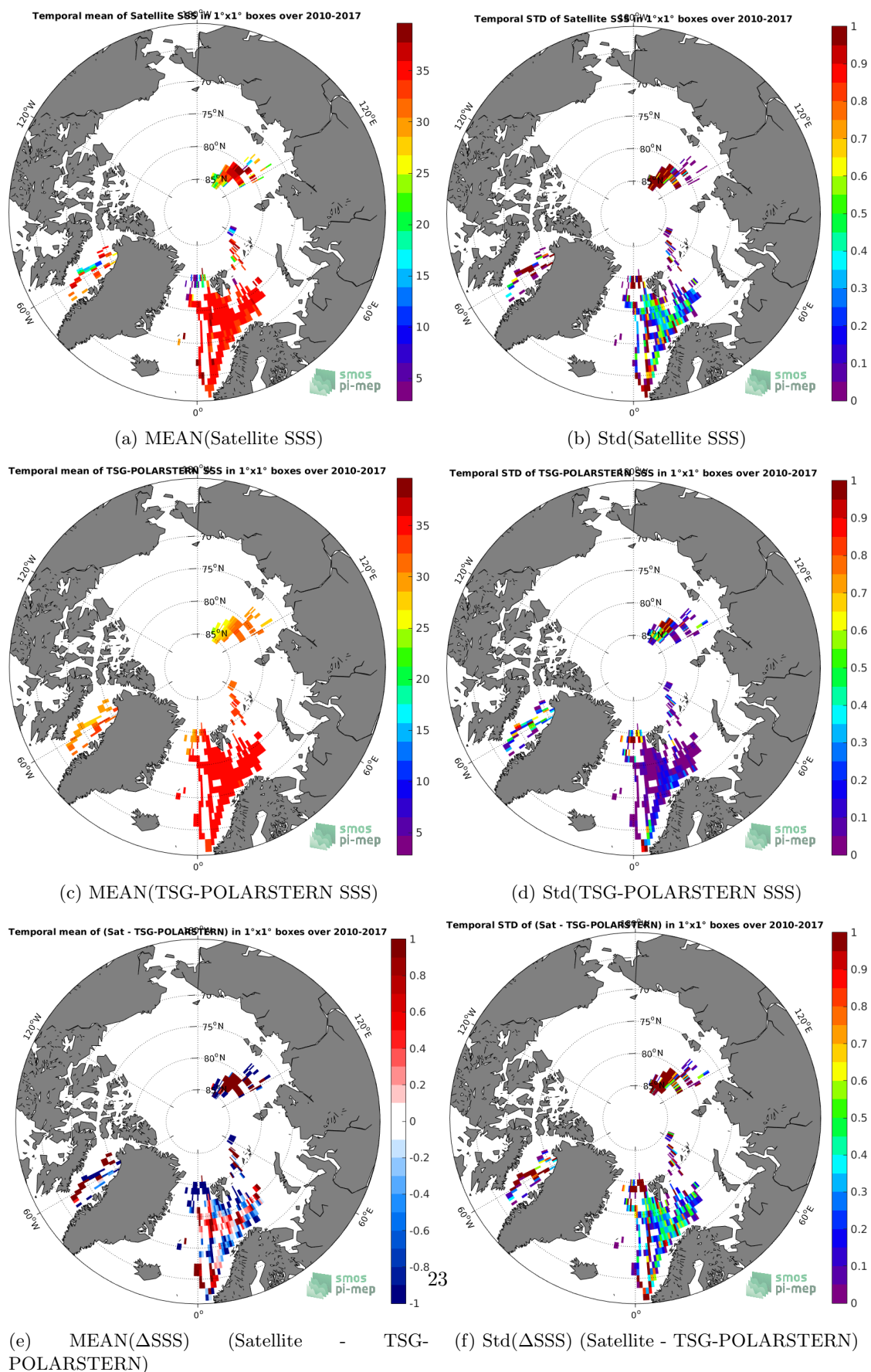
Figure 6: Temporal mean (left) and Std (right) of SSS from SMOS L3 v2 - Monthly - 0.25 Deg (CATDS-CECOS-IFREMER) (top), TSG-POLARSTERN (middle), and of \Delta SSS (Satellite - TSG-POLARSTERN). Only match-up pairs are used to generate these maps.
