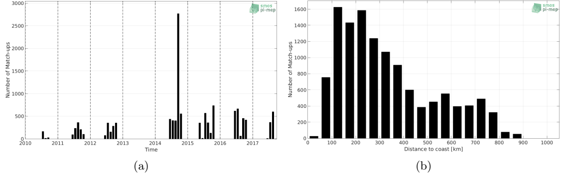
Figure 1: Number of match-ups between TSG-POLARSTERN and SMOS-L3-CATDS-IFREMER-CECOS-V2-MONTHLY-0.25DEG SSS as a function of time (a) and as function of the distance to coast (b) over the Arctic Ocean Pi-MEP region and for the full satellite product period.
