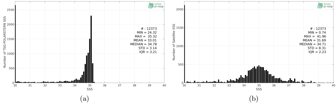
Figure 2: Histograms of SSS from TSG-POLARSTERN (a) and SMOS-L3-CATDS-IFREMER-CECOS-V2-MONTHLY-0.25DEG (b) considering all match-up pairs per bins of 0.1 over the Arctic Ocean Pi-MEP region and for the full satellite product period.
