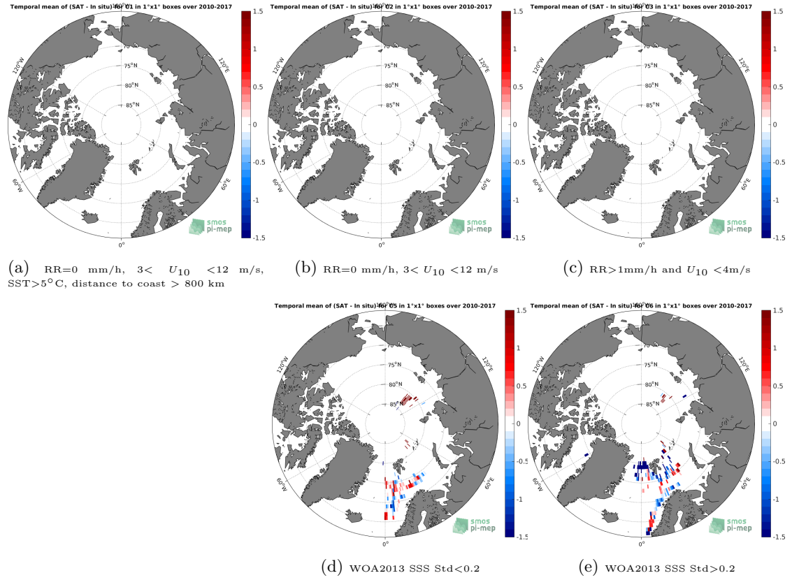
Figure 12: Temporal mean gridded over spatial boxes of size 1^\circ \times 1^\circ of \Delta SSS (SMOS-L3-CATDS-IFREMER-CECOS-V2-MONTHLY-0.25DEG - TSG-POLARSTERN) for 5 different subdatasets corresponding to: RR=0 mm/h, 3 < U_{10} < 12 m/s, SST > 5^\circ C , distance to coast > 800 km (a), RR=0 mm/h, 3 < U_{10} < 12 m/s (b), RR > 1 mm/h and U_{10} < 4 m/s (c), WOA2013 SSS Std < 0.2 (d), WOA2013 SSS Std > 0.2 (e).
