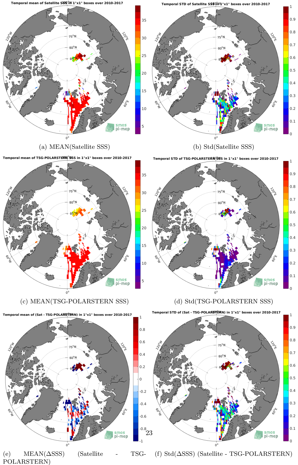
Figure 6: Temporal mean (left) and Std (right) of SSS from SMOS-L3-CATDS-IFREMER-CECOS-V2-MONTHLY-0.25DEG (top), TSG-POLARSTERN (middle), and of \Delta SSS (Satellite - TSG-POLARSTERN). Only match-up pairs are used to generate these maps.
