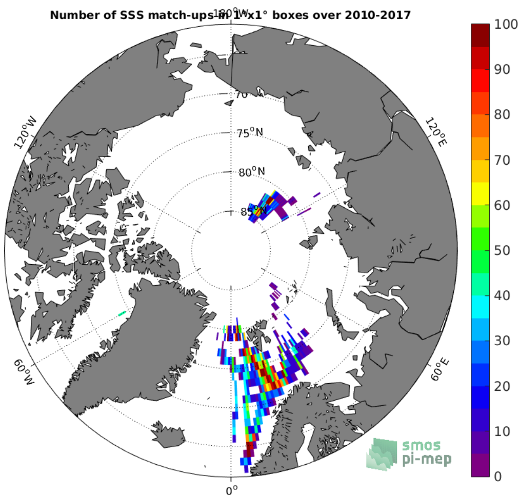
Figure 4: Number of SSS match-ups between TSG-POLARSTERN SSS and the SMOS-L3-CATDS-IFREMER-CECOS-V2-MONTHLY-0.25DEG SSS product for the Arctic Ocean Pi-MEP region over 1^\circ \times 1^\circ boxes and for the full satellite product period.
