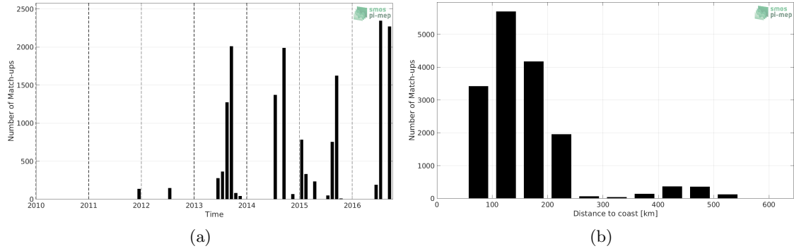
Figure 1: Number of match-ups between TSG (LEGOS-DM) and SMOS SSS L3 v2 - Monthly - 0.25 Deg (CATDS-CECOS-IFREMER) SSS as a function of time (a) and as function of the distance to coast (b) over the Arctic Ocean Pi-MEP region and for the full satellite product period.
