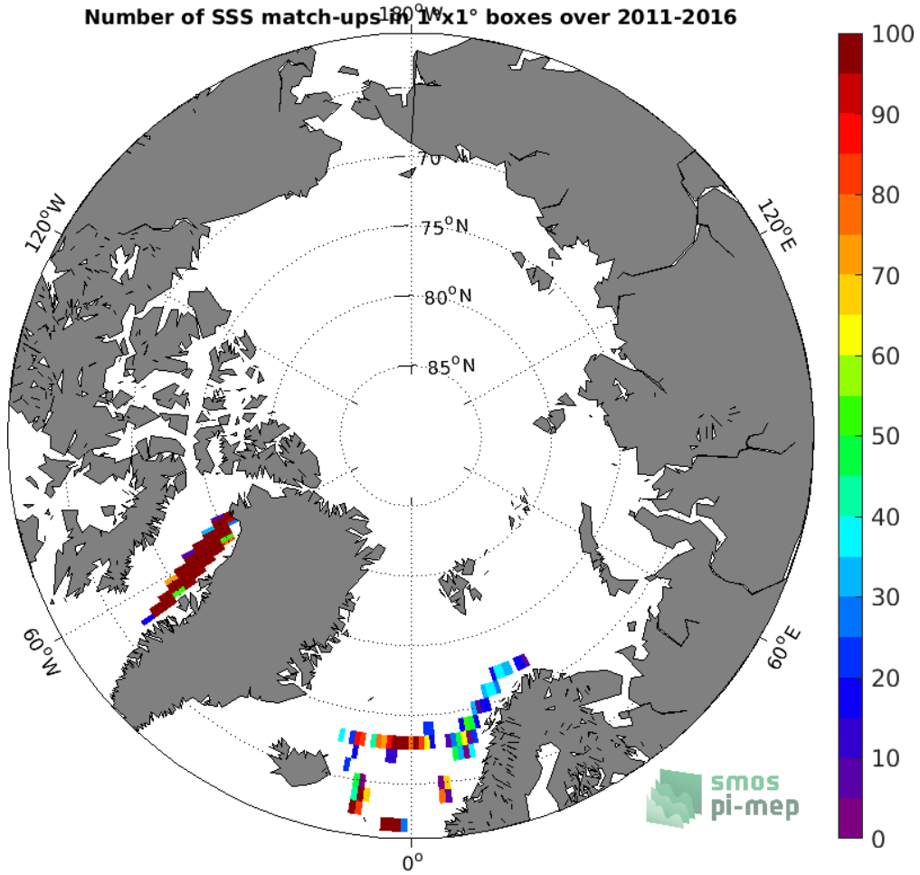
Figure 4: Number of SSS match-ups between TSG (LEGOS-DM) SSS and the SMOS SSS L3 v2 - Monthly - 0.25 Deg (CATDS-CECOS-IFREMER) SSS product for the Arctic Ocean Pi-MEP region over 1°x1° boxes and for the full satellite product period.
