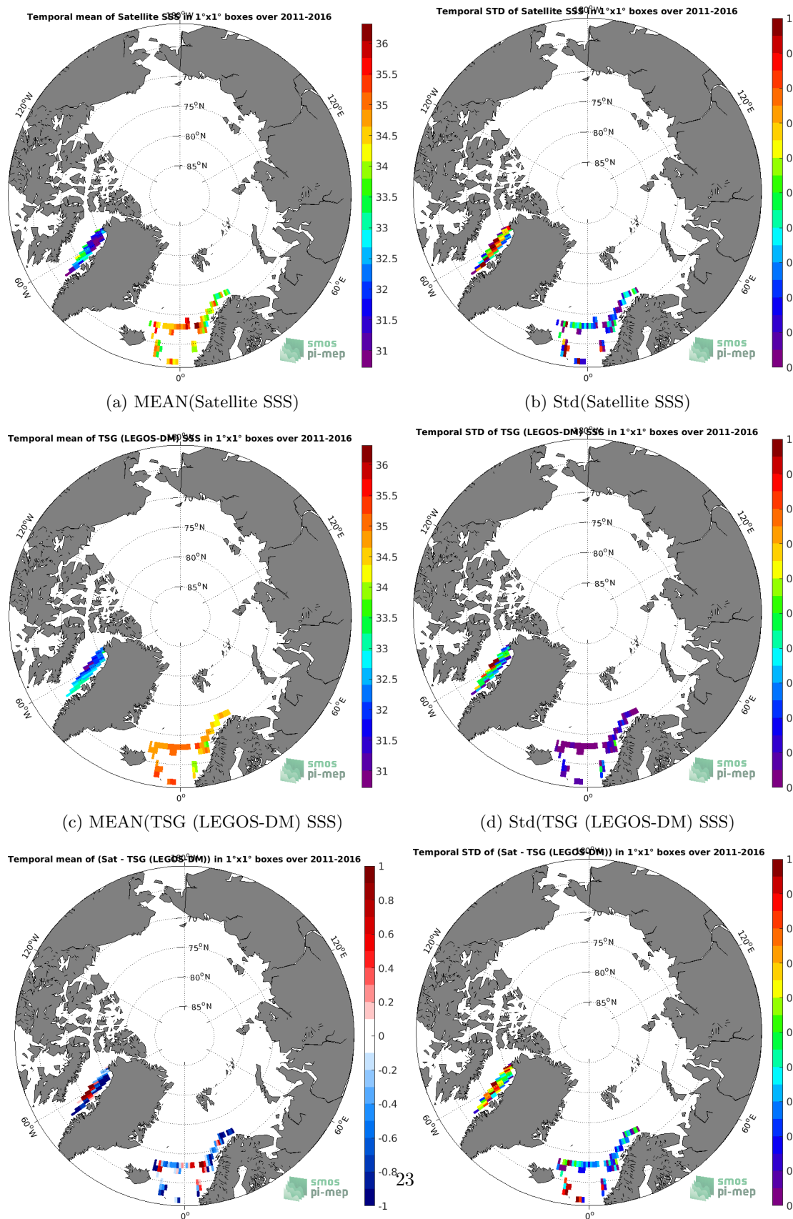
Figure 6: Temporal mean (left) and Std (right) of SSS from SMOS SSS L3 v2 - Monthly - 0.25 Deg (CATDS-CECOS-IFREMER) (top), TSG (LEGOS-DM) (middle), and of \Delta SSS (Satellite - TSG (LEGOS-DM)). Only match-up pairs are used to generate these maps.
