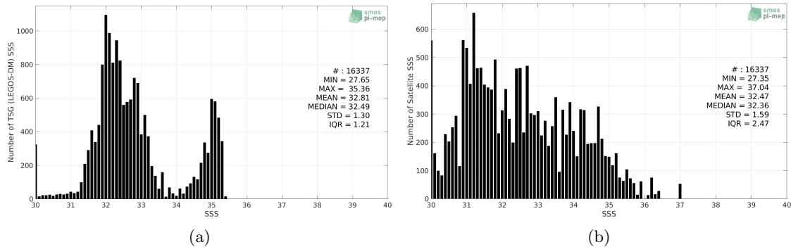
Figure 2: Histograms of SSS from TSG (LEGOS-DM) (a) and SMOS SSS L3 v2 - Monthly - 0.25 Deg (CATDS-CECOS-IFREMER) (b) considering all match-up pairs per bins of 0.1 over the Arctic Ocean Pi-MEP region and for the full satellite product period.
