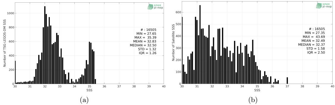
Figure 2: Histograms of SSS from TSG-LEGOS-DM (a) and SMOS L3 v2 - Monthly - 0.25 Deg (CATDS-CECOS-IFREMER) (b) considering all match-up pairs per bins of 0.1 over the Arctic Ocean Pi-MEP region and for the full satellite product period.
