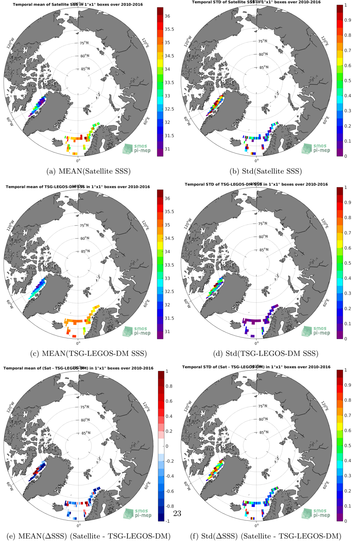
Figure 6: Temporal mean (left) and Std (right) of SSS from SMOS L3 v2 - Monthly - 0.25 Deg (CATDS-CECOS-IFREMER) (top), TSG-LEGOS-DM (middle), and of \Delta SSS (Satellite - TSG-LEGOS-DM). Only match-up pairs are used to generate these maps.
