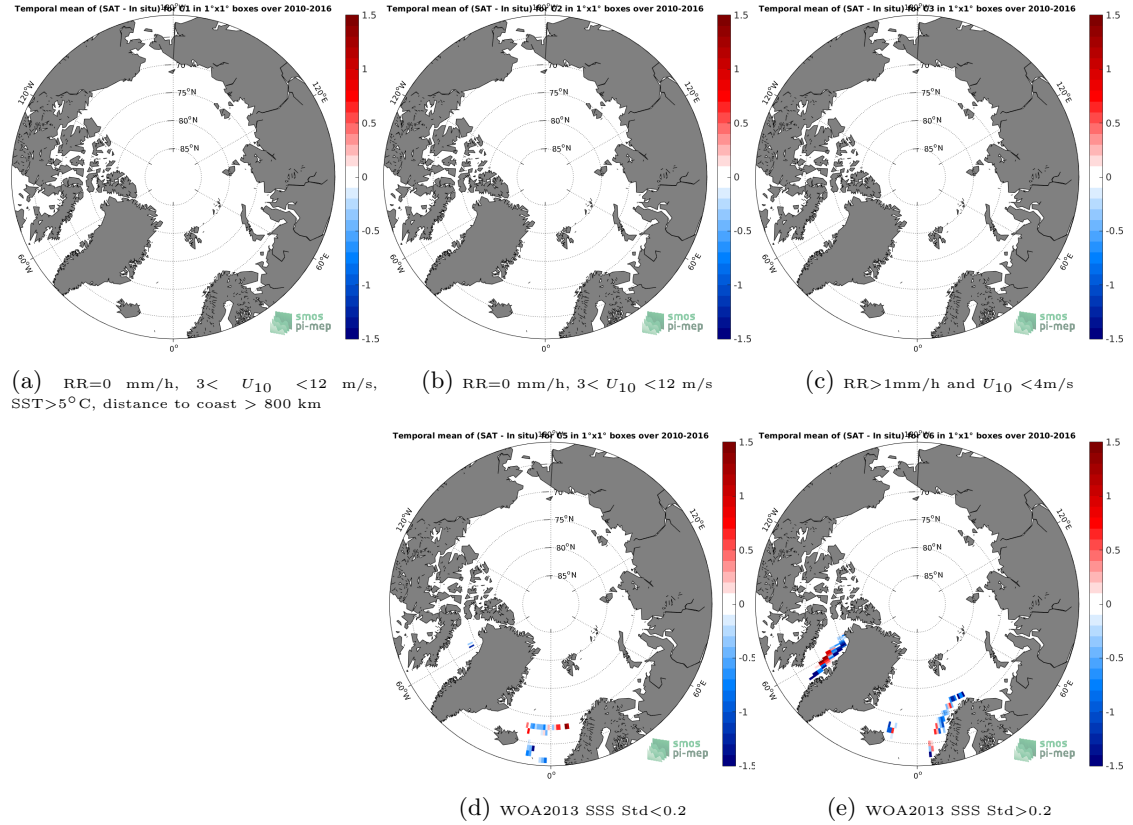
Figure 12: Temporal mean gridded over spatial boxes of size 1^{\circ}\times 1^{\circ} of \Delta\text{SSS} (SMOS L3 v2 - Monthly - 0.25 Deg (CATDS-CECOS-IFREMER) - TSG-LEGOS-DM) for 5 different subdatasets corresponding to: RR=0 mm/h, 3 < U_{10} < 12 m/s, SST > 5^{\circ}\text{C} , distance to coast > 800 km (a), RR=0 mm/h, 3 < U_{10} < 12 m/s (b), RR > 1 mm/h and U_{10} < 4 m/s (c), WOA2013 SSS Std < 0.2 (d), WOA2013 SSS Std > 0.2 (e).
