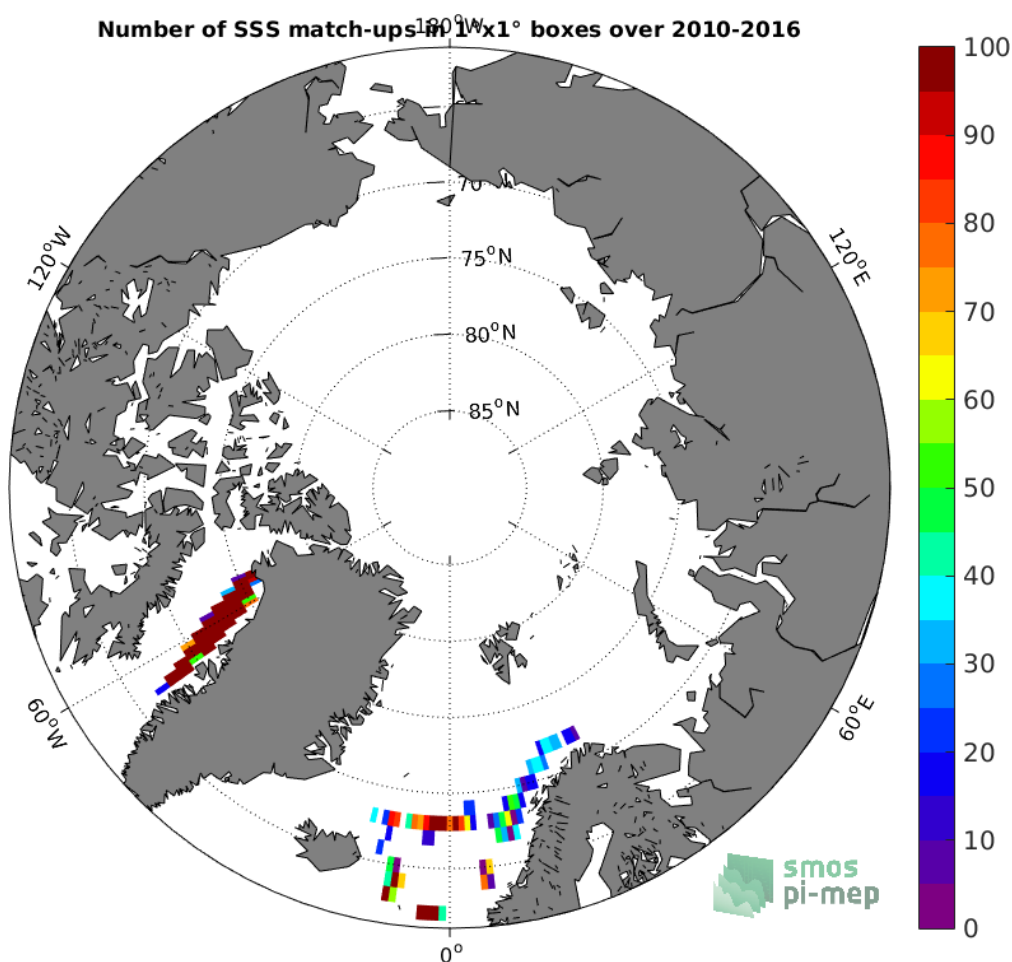
Figure 4: Number of SSS match-ups between TSG-LEGOS-DM SSS and the SMOS L3 v2 - Monthly - 0.25 Deg (CATDS-CECOS-IFREMER) SSS product for the Arctic Ocean Pi-MEP region over 1°x1° boxes and for the full satellite product period.
