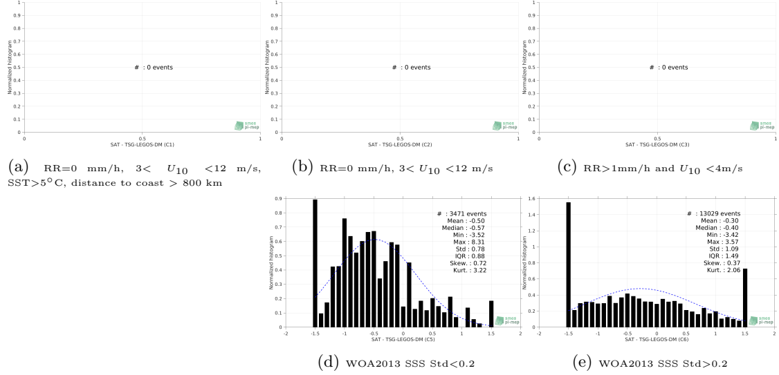
Figure 13: Normalized histogram of \Delta SSS (SMOS L3 v2 - Monthly - 0.25 Deg (CATDS-CECOS-IFREMER) - TSG-LEGOS-DM) for 5 different subdatasets corresponding to: RR=0 mm/h, 3 < U_{10} < 12 m/s, SST>5°C, distance to coast > 800 km (a), RR=0 mm/h, 3 < U_{10} < 12 m/s (b), RR>1 mm/h and U_{10} < 4 m/s (c), WOA2013 SSS Std<0.2 (d), WOA2013 SSS Std>0.2 (e).
