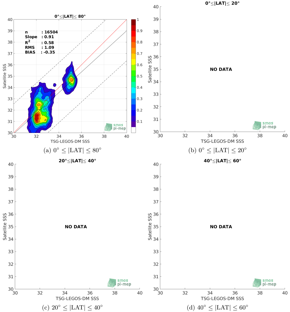
Figure 9: Contour maps of the concentration of SMOS L3 v2 - Monthly - 0.25 Deg (CATDS-CECOS-IFREMER) SSS (y-axis) versus TSG-LEGOS-DM SSS (x-axis) at match-up pairs for different latitude bands. For each plot, the red line shows x=y . The black thin and dashed lines indicate a linear fit through the data cloud and the \pm 95\% confidence levels, respectively. The number match-up pairs n , the slope and R^2 coefficient of the linear fit, the root mean square (RMS) and the mean bias between satellite and in situ data are indicated for each latitude band in each plots.
