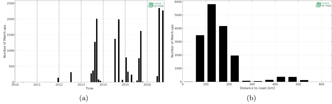
Figure 1: Number of match-ups between TSG-LEGOS-DM and SMOS L3 v2 - Monthly - 0.25 Deg (CATDS-CECOS-IFREMER) SSS as a function of time (a) and as function of the distance to coast (b) over the Arctic Ocean Pi-MEP region and for the full satellite product period.
