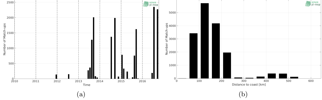
Figure 1: Number of match-ups between TSG-LEGOS-DM and SMOS-L3-CATDS-IFREMER-CECOS-V2-MONTHLY-0.25DEG SSS as a function of time (a) and as function of the distance to coast (b) over the Arctic Ocean Pi-MEP region and for the full satellite product period.
