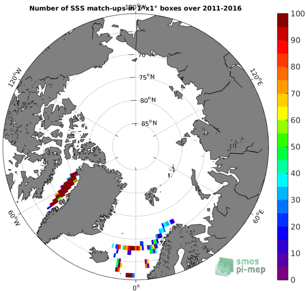
Figure 4: Number of SSS match-ups between TSG-LEGOS-DM SSS and the SMOS-L3-CATDS-IFREMER-CECOS-V2-MONTHLY-0.25DEG SSS product for the Arctic Ocean Pi-MEP region over 1°x1° boxes and for the full satellite product period.
