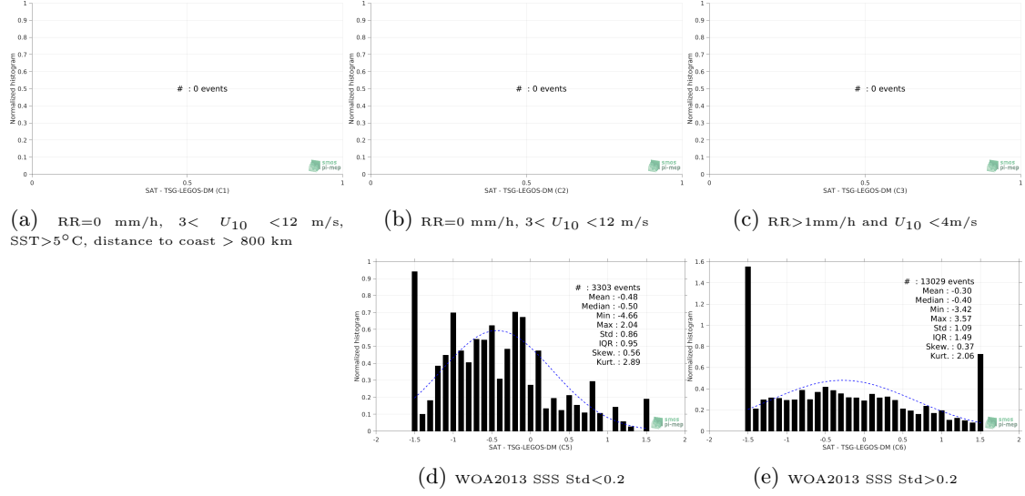
Figure 13: Normalized histogram of \Delta\text{SSS} (SMOS-L3-CATDS-IFREMER-CECOS-V2-MONTHLY-0.25DEG - TSG-LEGOS-DM) for 5 different subdatasets corresponding to: RR=0 mm/h, 3 < U_{10} < 12 m/s, SST > 5^\circ\text{C} , distance to coast > 800 km (a), RR=0 mm/h, 3 < U_{10} < 12 m/s (b), RR > 1\text{mm/h} and U_{10} < 4\text{m/s} (c), WOA2013 SSS Std<0.2 (d), WOA2013 SSS Std>0.2 (e).
