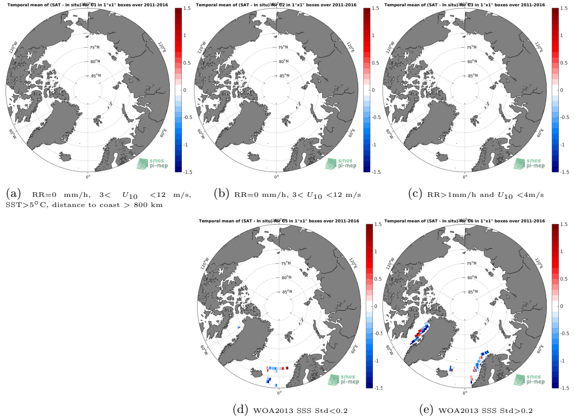
Figure 12: Temporal mean gridded over spatial boxes of size 1^\circ \times 1^\circ of \Delta SSS (SMOS-L3-CATDS-IFREMER-CECOS-V2-MONTHLY-0.25DEG - TSG-LEGOS-DM) for 5 different subdatasets corresponding to: RR=0 mm/h, 3 < U_{10} < 12 m/s, SST > 5^\circ\text{C} , distance to coast > 800 km (a), RR=0 mm/h, 3 < U_{10} < 12 m/s (b), RR > 1 mm/h and U_{10} < 4 m/s (c), WOA2013 SSS Std < 0.2 (d), WOA2013 SSS Std > 0.2 (e).
