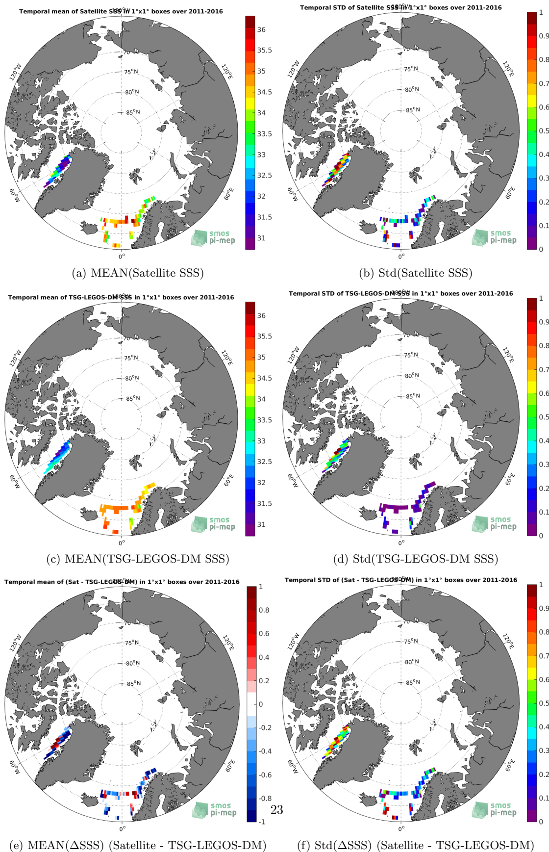
Figure 6: Temporal mean (left) and Std (right) of SSS from SMOS-L3-CATDS-IFREMER-CECOS-V2-MONTHLY-0.25DEG (top), TSG-LEGOS-DM (middle), and of \Delta SSS (Satellite - TSG-LEGOS-DM). Only match-up pairs are used to generate these maps.
