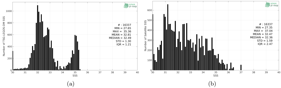
Figure 2: Histograms of SSS from TSG-LEGOS-DM (a) and SMOS-L3-CATDS-IFREMER-CECOS-V2-MONTHLY-0.25DEG (b) considering all match-up pairs per bins of 0.1 over the Arctic Ocean Pi-MEP region and for the full satellite product period.
