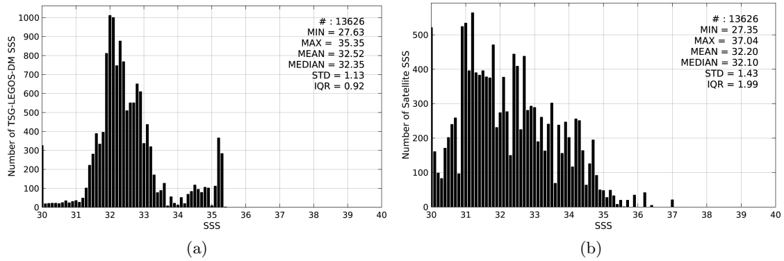
Figure 2: Histograms of SSS from TSG-LEGOS-DM (a) and SMOS-L3-CATDS-IFREMER-CECOS-V2-MONTHLY-0.25DEG (b) considering all match-up pairs per bins of 0.1 over the Arctic Ocean Pi-MEP region and for the full satellite product period.
