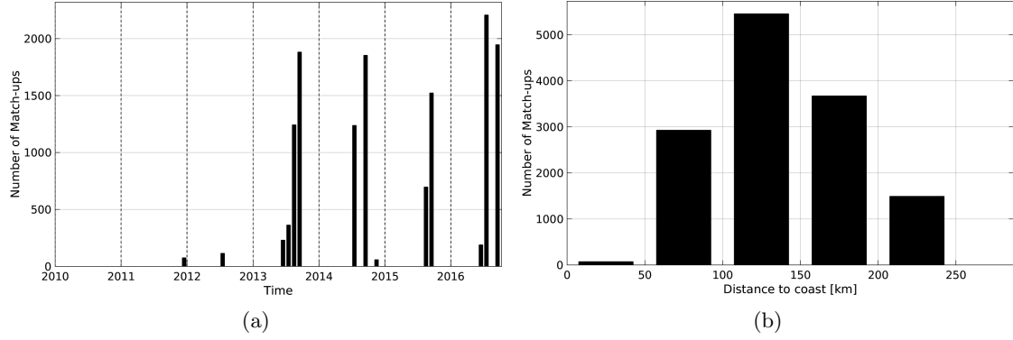
Figure 1: Number of match-ups between TSG-LEGOS-DM and SMOS-L3-CATDS-IFREMER-CECOS-V2-MONTHLY-0.25DEG SSS as a function of time (a) and as function of the distance to coast (b) over the Arctic Ocean Pi-MEP region and for the full satellite product period.
